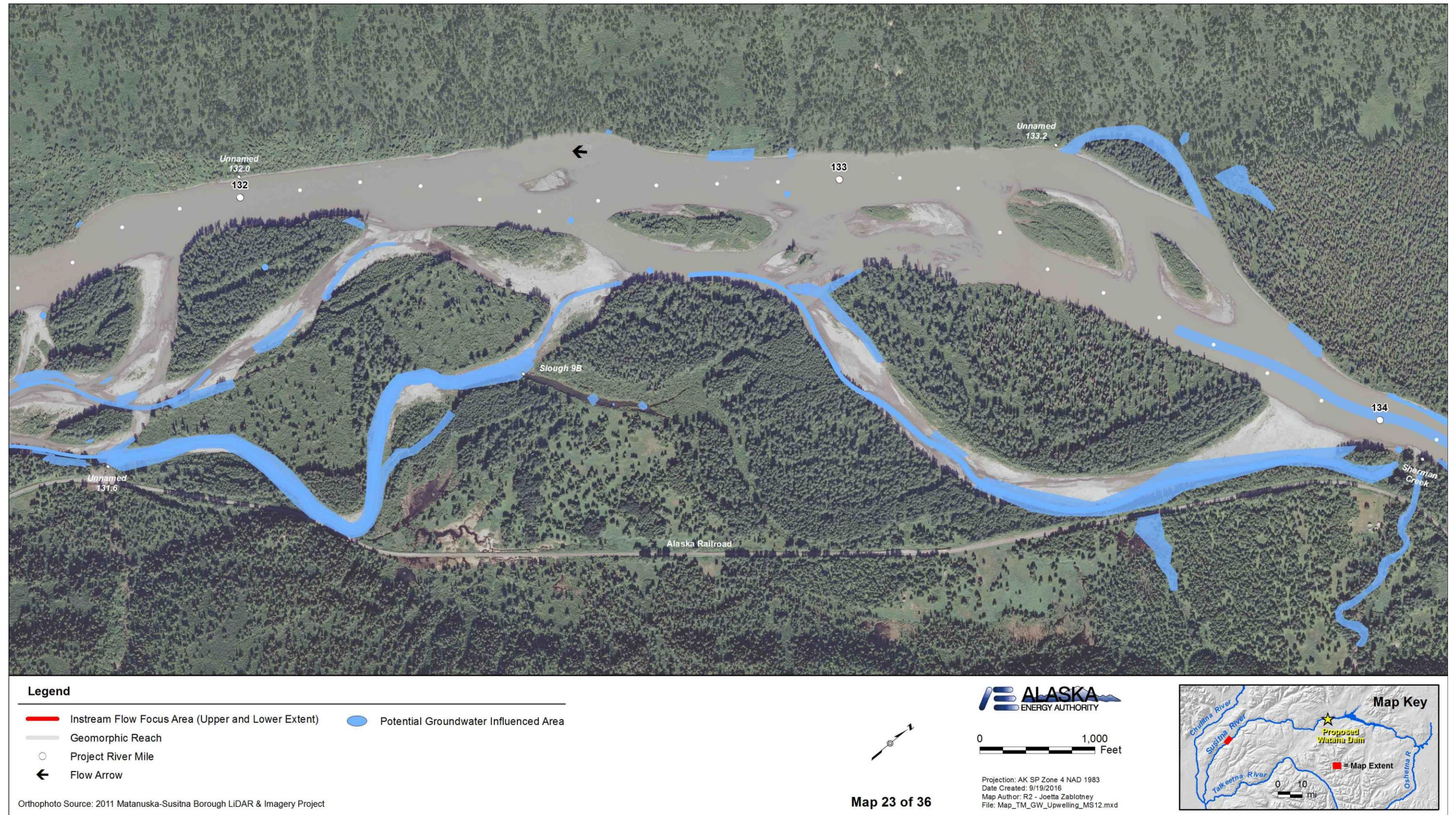
Figure A-23. Locations of potential groundwater influenced areas between PRM 134.1 and PRM 131.6 within the Middle River Segment of the Susitna River.
