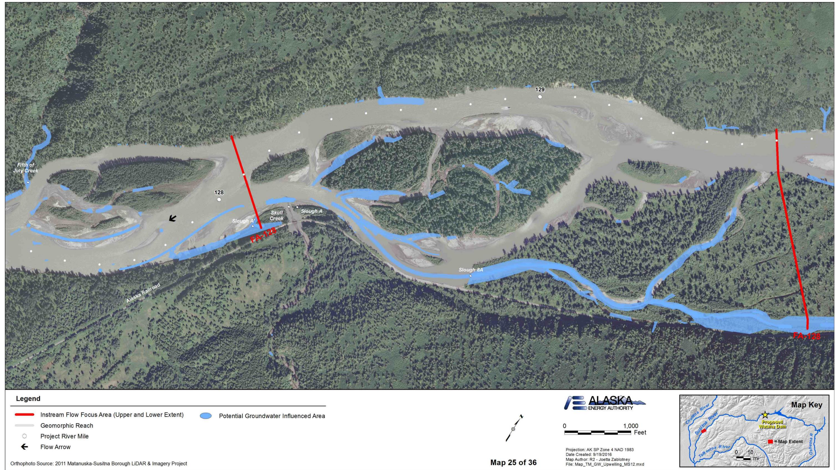
Figure A-25. Locations of potential groundwater influenced areas between PRM 129.8 and PRM 127.4 within the Middle River Segment of the Susitna River.
