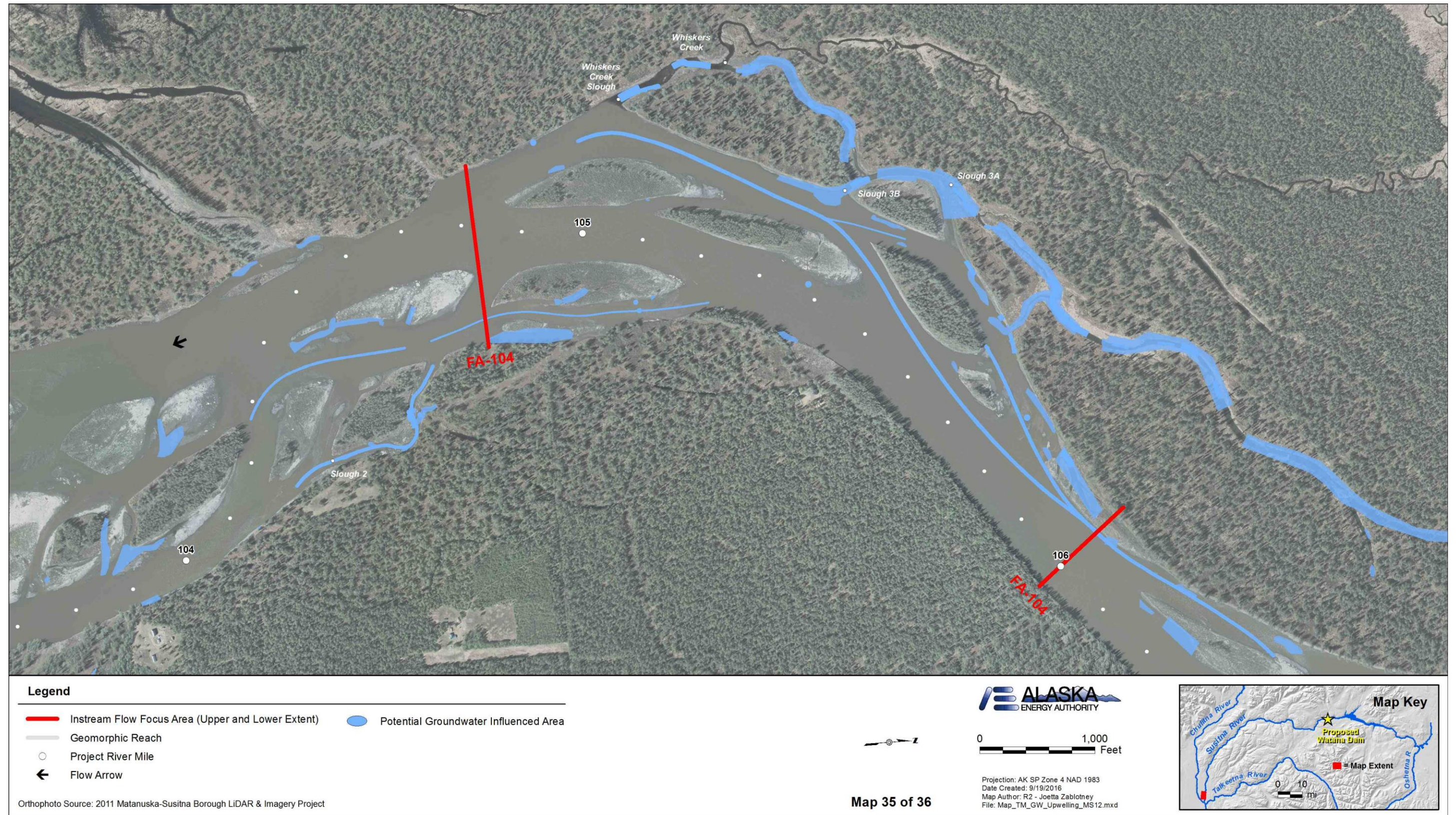
Figure A-35. Locations of potential groundwater influenced areas between PRM 106.2 and PRM 103.7 within the Middle River Segment of the Susitna River.
