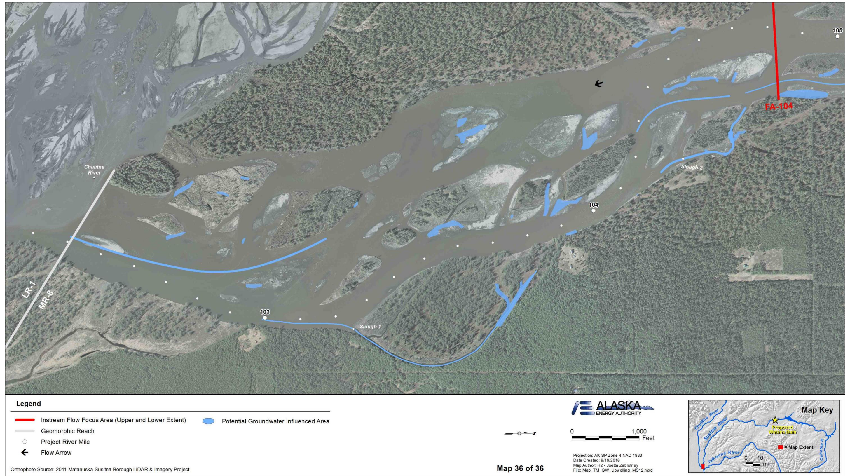
Figure A-36. Locations of potential groundwater influenced areas between PRM 105.0 and PRM 102.3 within the Middle River Segment of the Susitna River/
