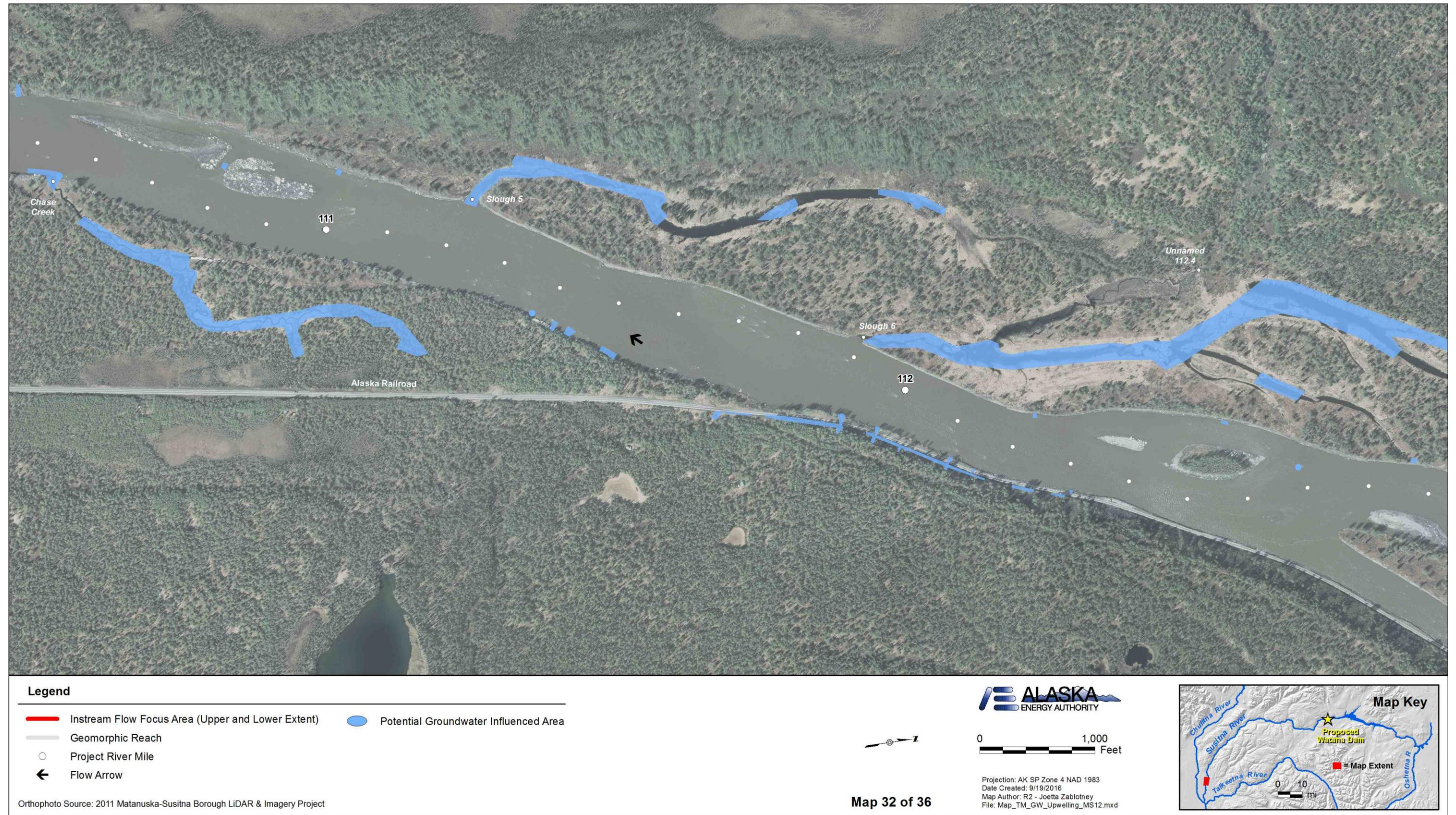
Figure A-32. Locations of potential groundwater influenced areas between PRM 112.9 and PRM 110.5 within the Middle River Segment of the Susitna River.
