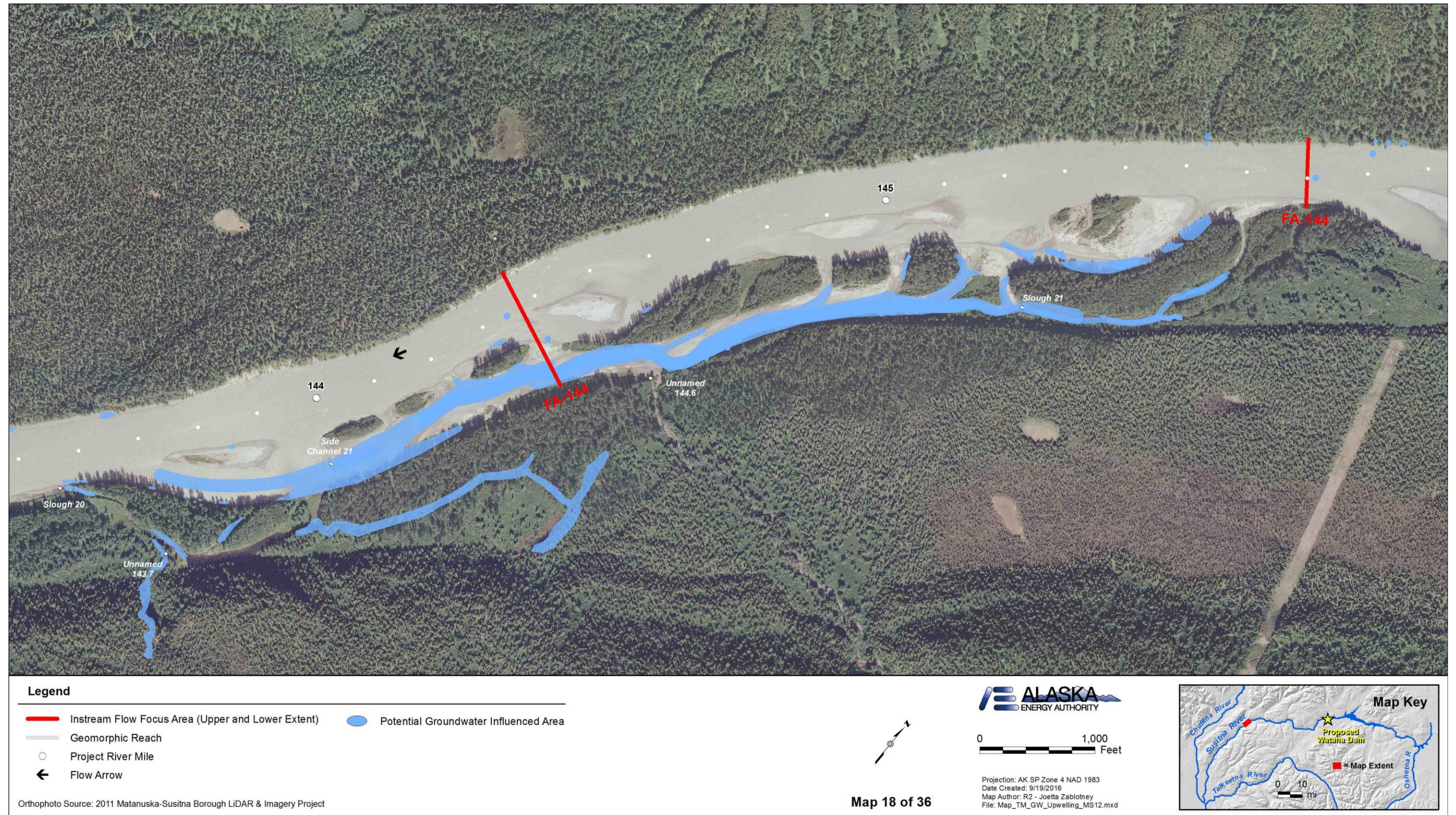
Figure A-18. Locations of potential groundwater influenced areas between PRM 145.9 and PRM 143.5 within the Middle River Segment of the Susitna River.
