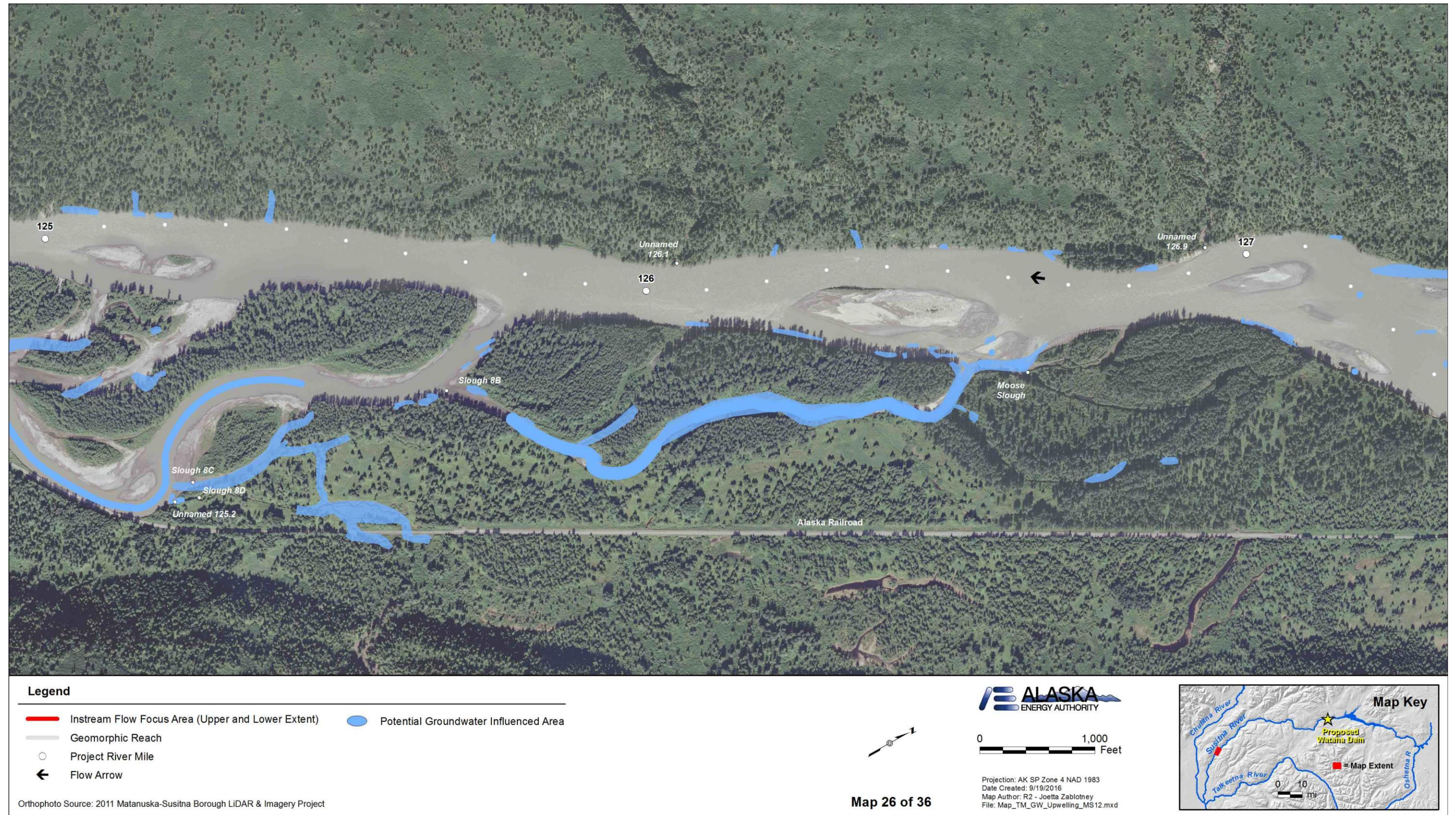
Figure A-26. Locations of potential groundwater influenced areas between PRM 127.4 and PRM 125.0 within the Middle River Segment of the Susitna River.
