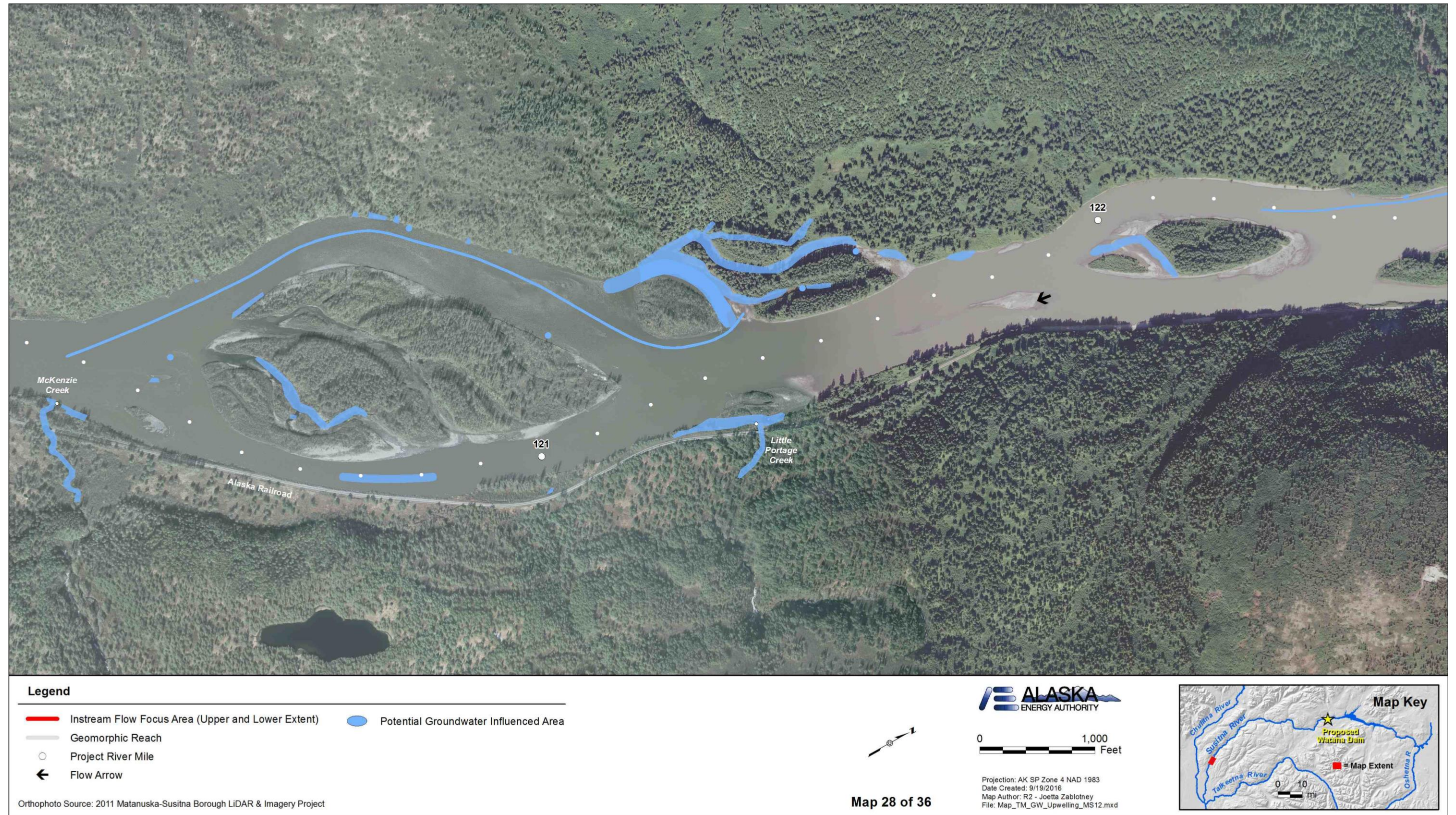
Figure A-28. Locations of potential groundwater influenced areas between PRM 122.5 and PRM 120.1 within the Middle River Segment of the Susitna River.
