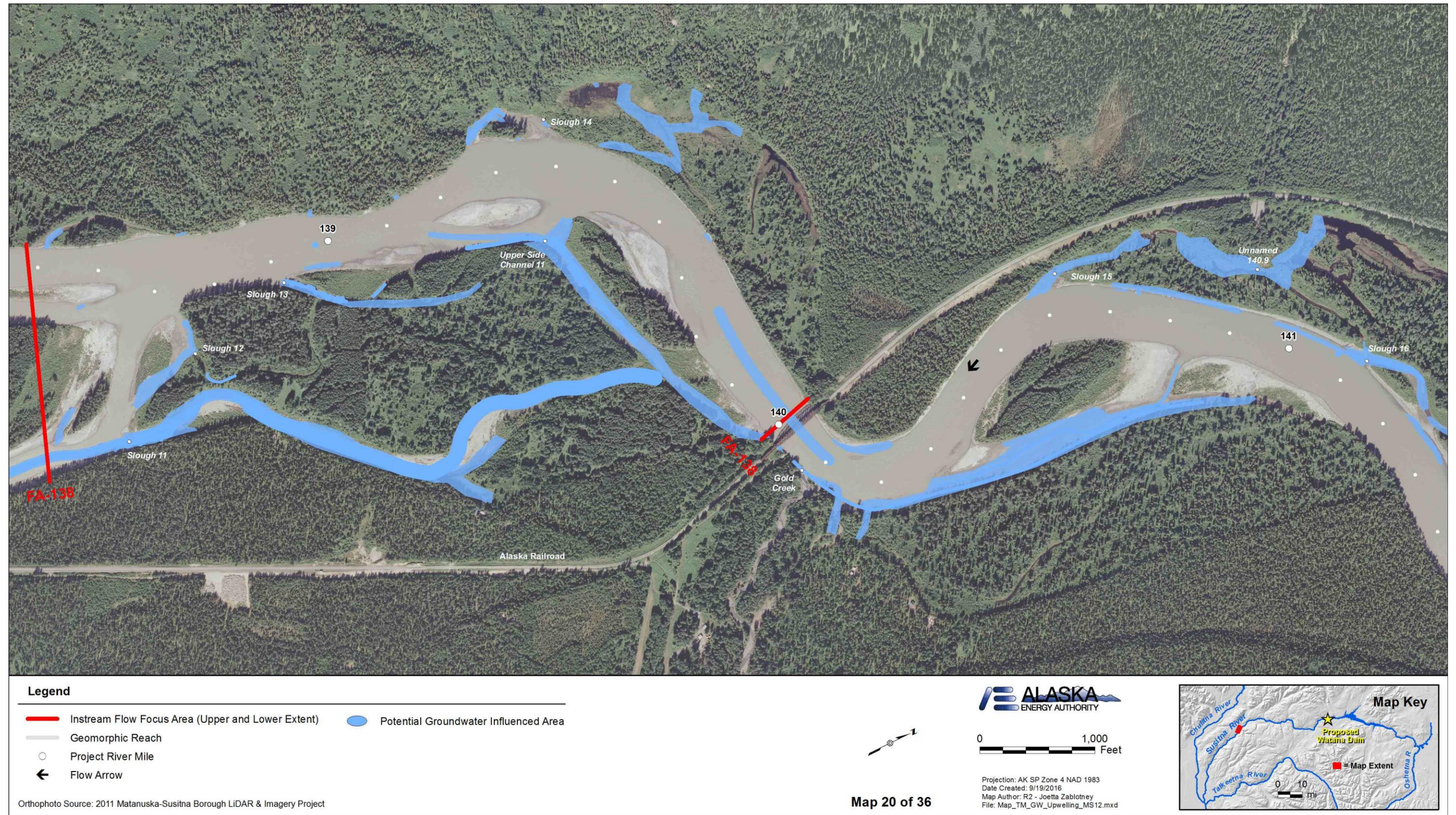
Figure A-20. Locations of potential groundwater influenced areas between PRM 141.4 and PRM 138.5 within the Middle River Segment of the Susitna River.
