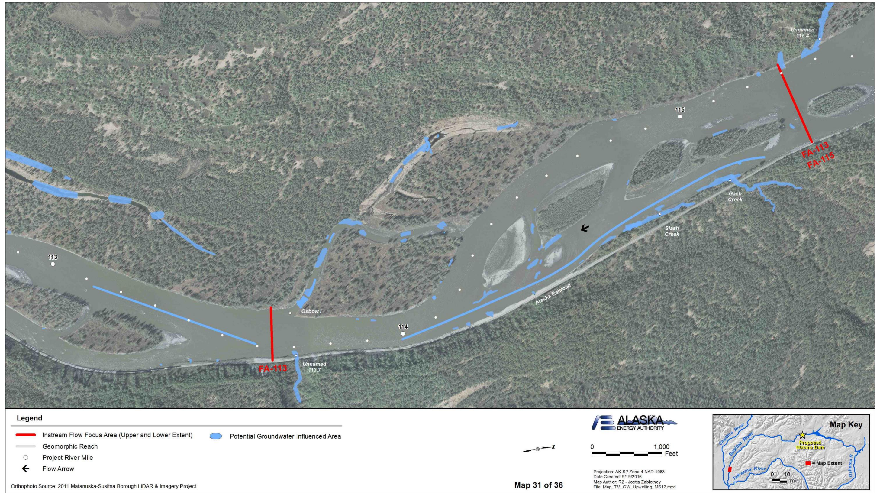
Figure A-31. Locations of potential groundwater influenced areas between PRM 115.5 and PRM 112.9 within the Middle River Segment of the Susitna River.
