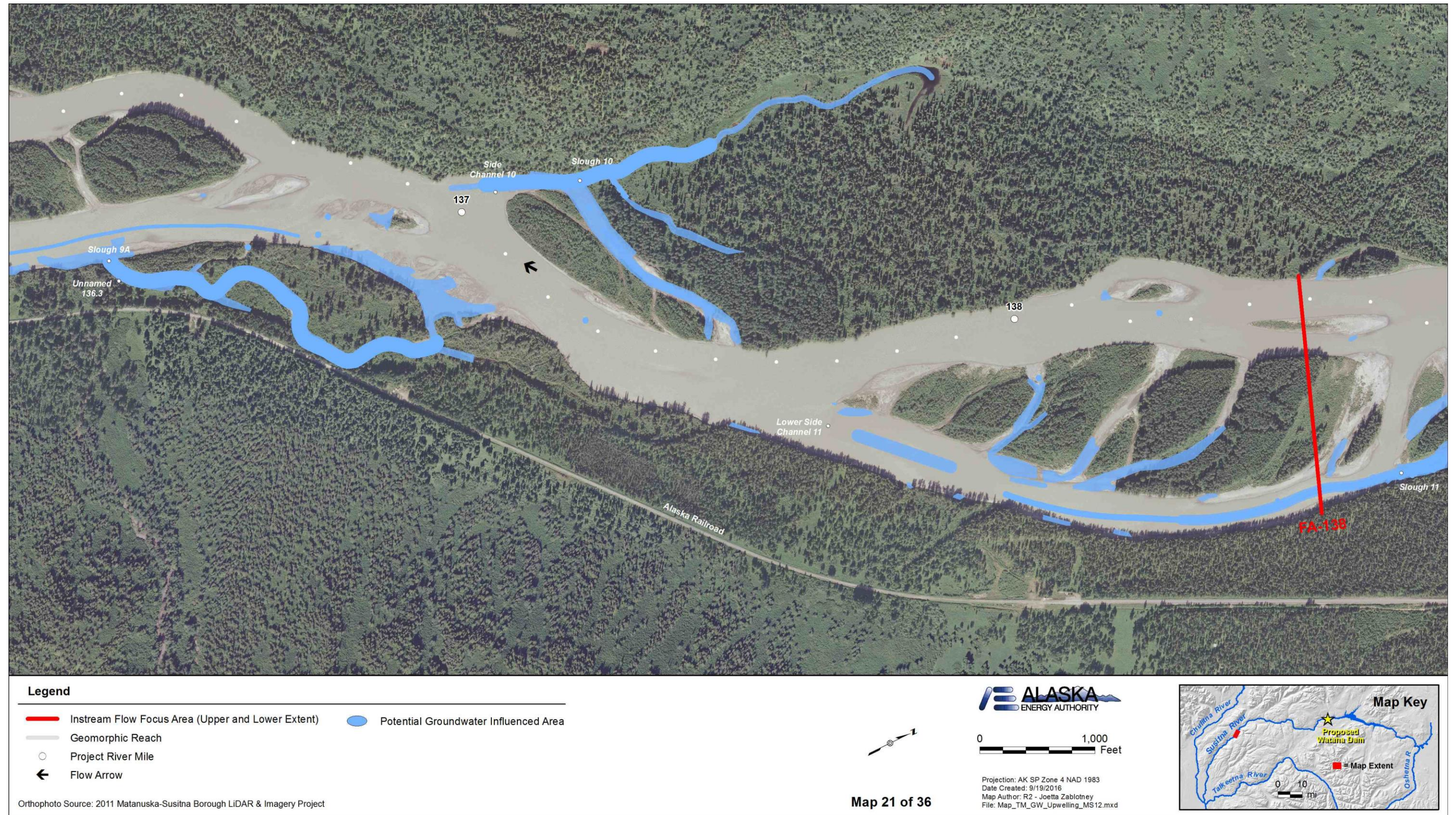
Figure A-21. Locations of potential groundwater influenced areas between PRM 138.7 and PRM 136.3 within the Middle River Segment of the Susitna River.
