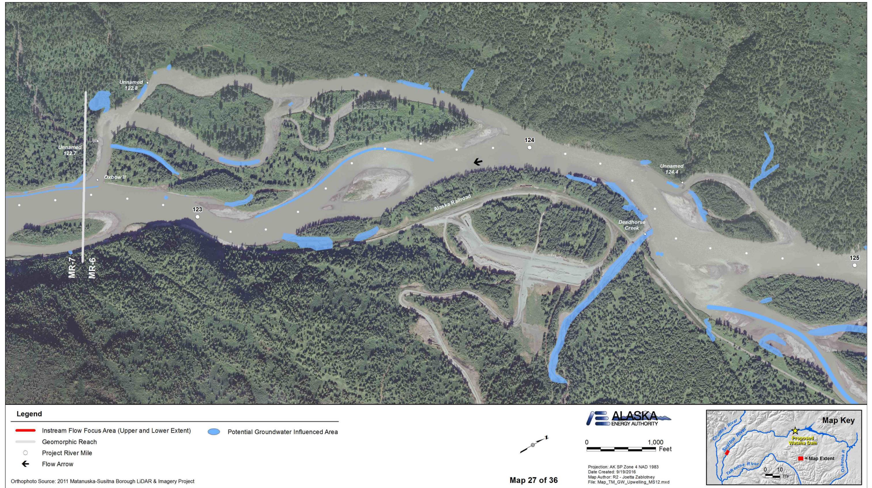
Figure A-27. Locations of potential groundwater influenced areas between PRM 125.0 and PRM 122.5 within the Middle River Segment of the Susitna River.
