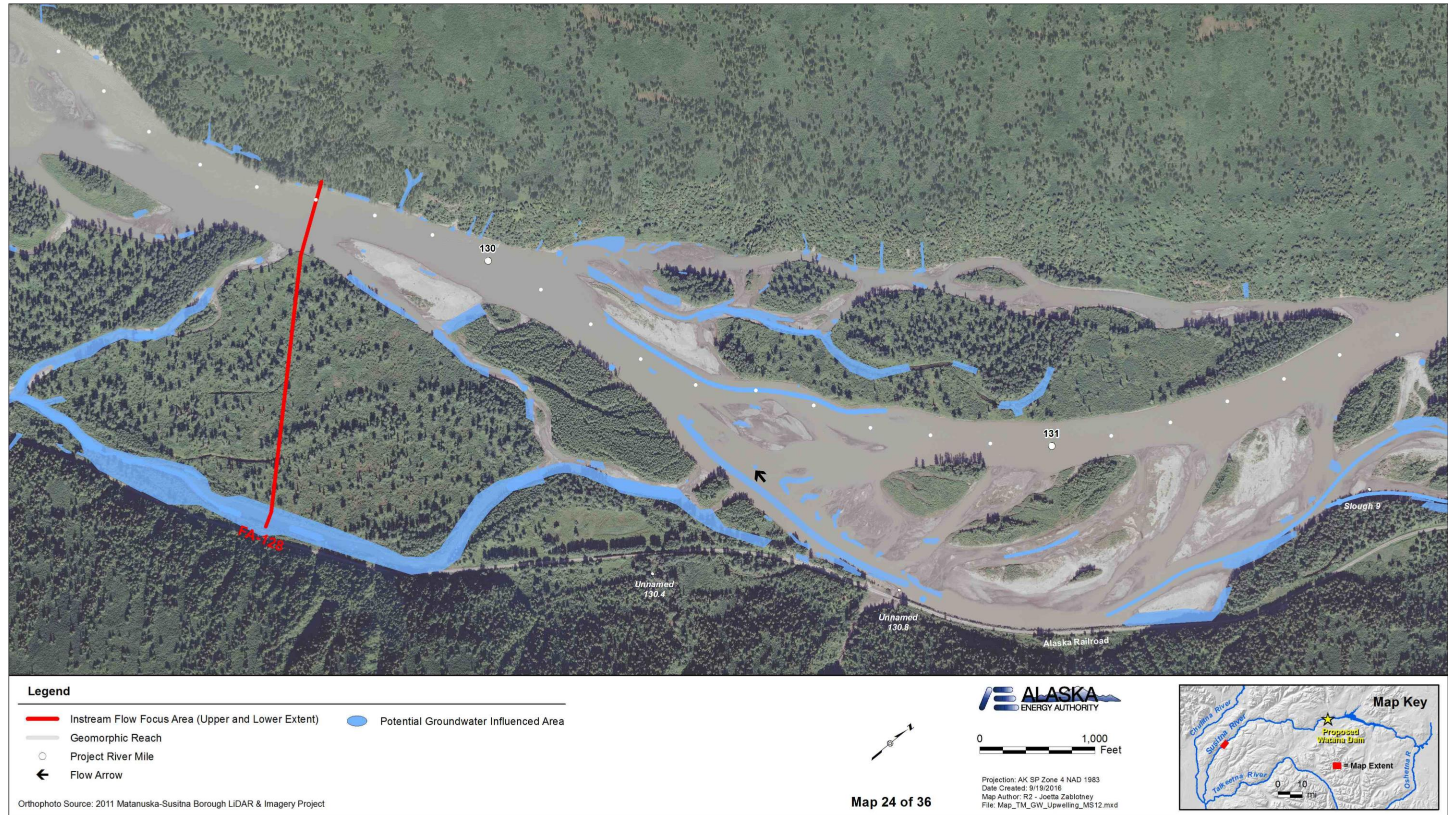
Figure A-24. Locations of potential groundwater influenced areas between PRM 131.6 and PRM 129.2 within the Middle River Segment of the Susitna River.
