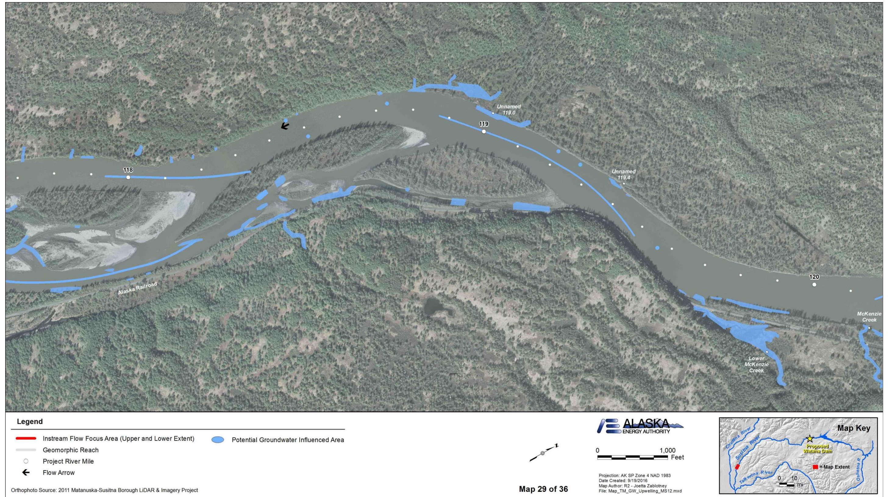
Figure A-29. Locations of potential groundwater influenced areas between PRM 120.1 and PRM 117.7 within the Middle River Segment of the Susitna River.
