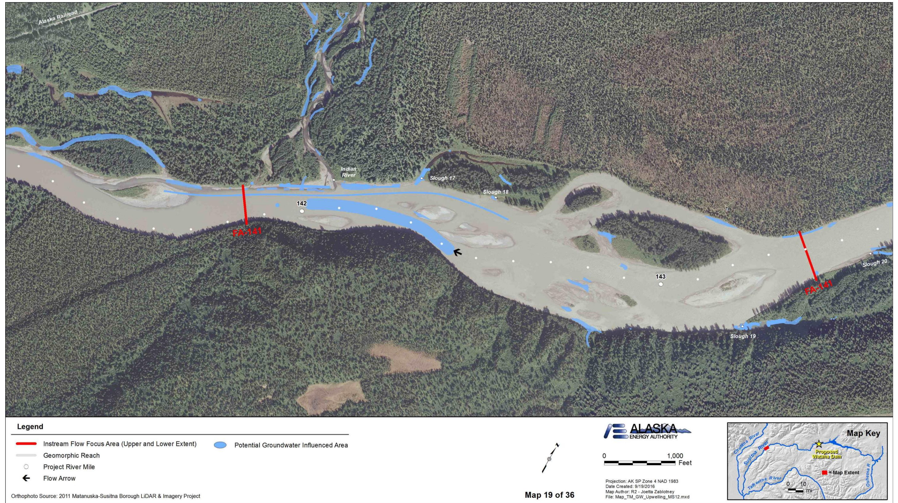
Figure A-19. Locations of potential groundwater influenced areas between PRM 143.6 and PRM 141.2 within the Middle River Segment of the Susitna River.
