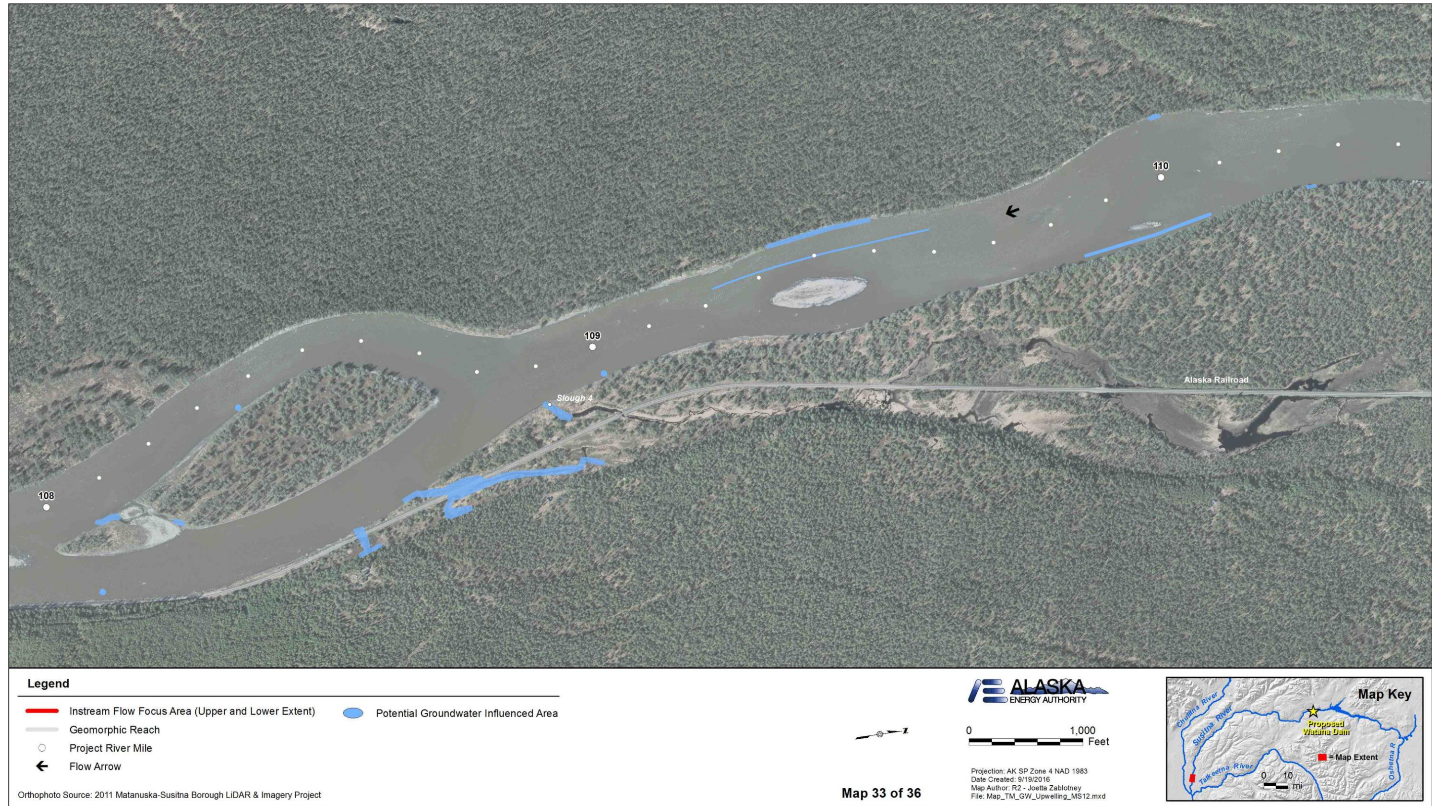
Figure A-33. Locations of potential groundwater influenced areas between PRM 110.4 and PRM 108.0 within the Middle River Segment of the Susitna River.
