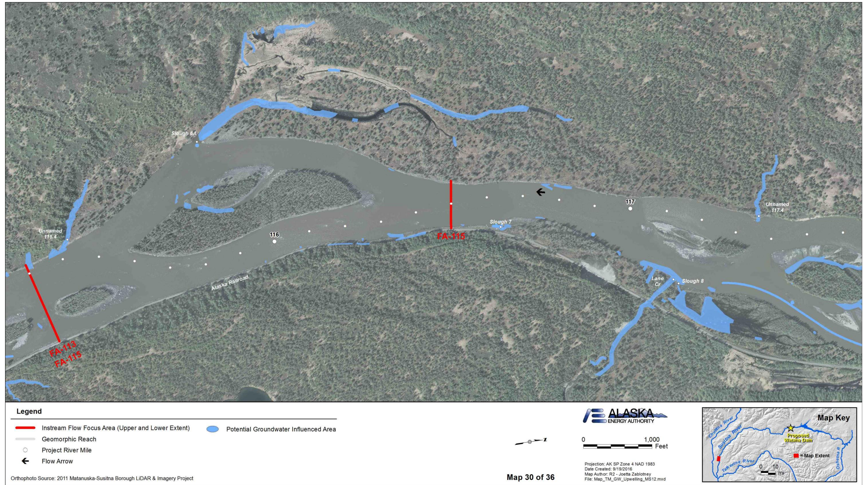
Figure A-30. Locations of potential groundwater influenced areas between PRM 117.6 and PRM 115.3 within the Middle River Segment of the Susitna River.
