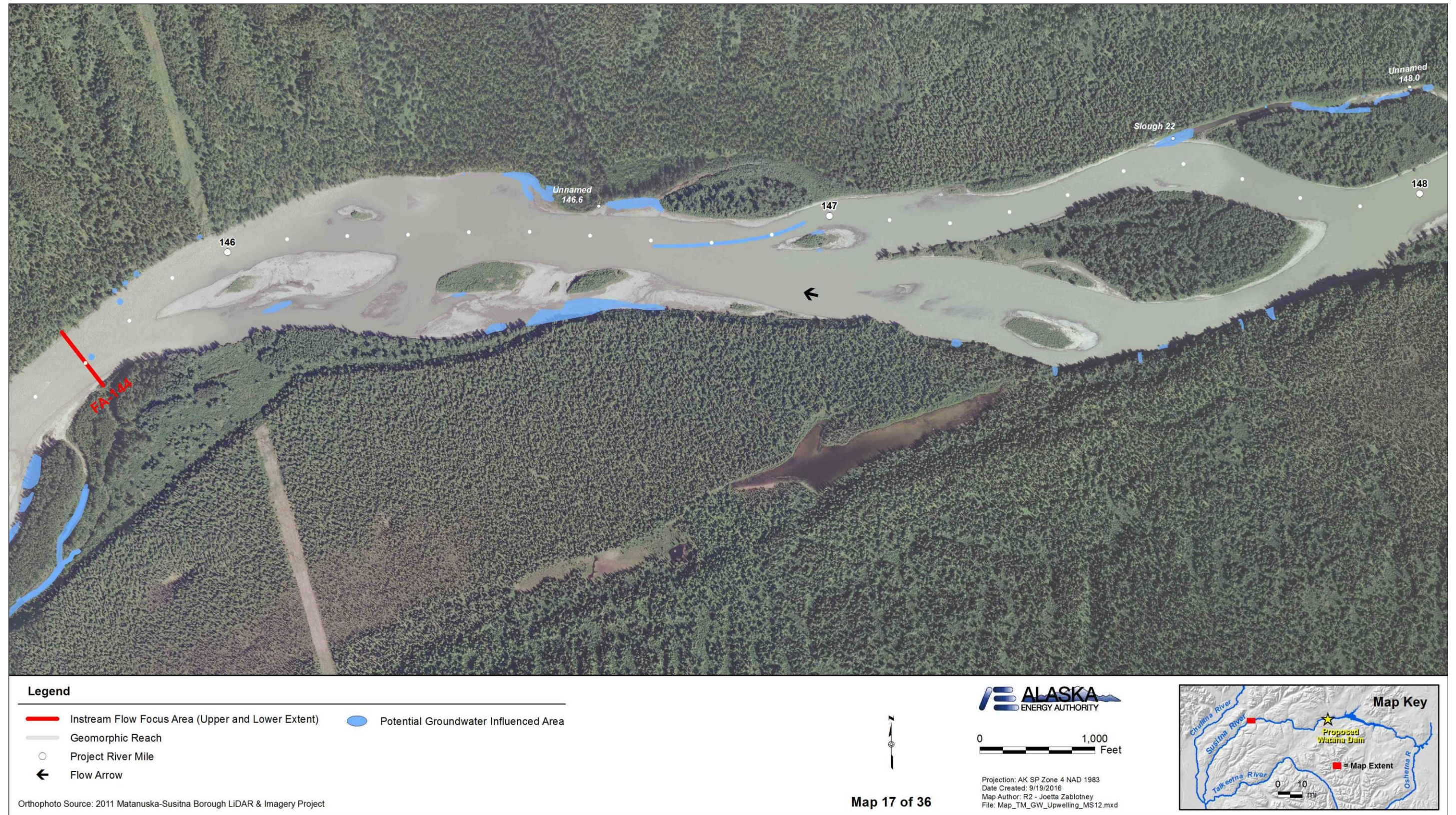
Figure A-17. Locations of potential groundwater influenced areas between PRM 148.0 and PRM 145.6 within the Middle River Segment of the Susitna River.
