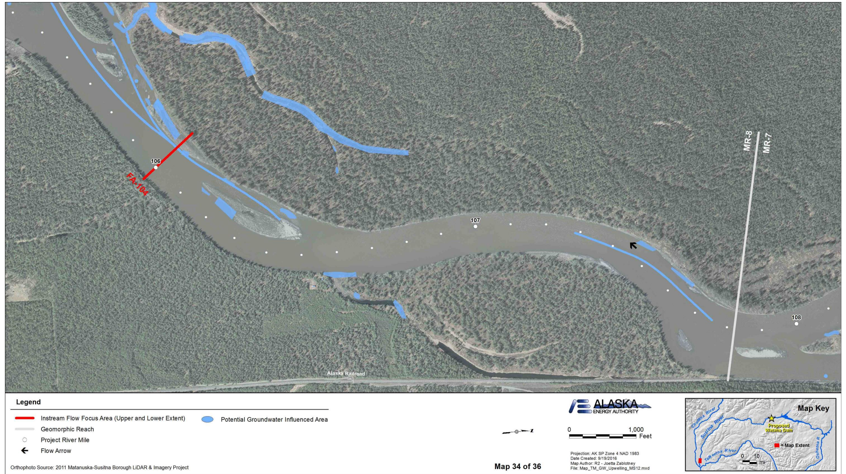
Figure A-34. Locations of potential groundwater influenced areas between PRM 108.1 and PRM 105.4 within the Middle River Segment of the Susitna River.
