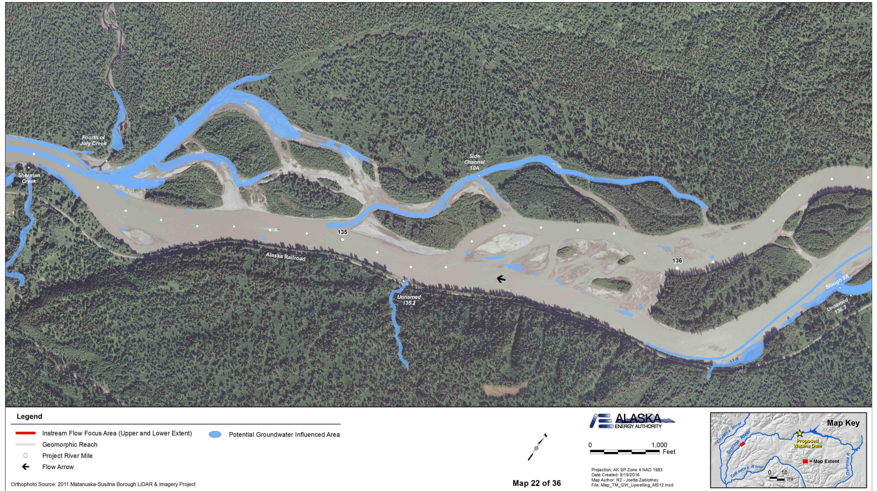
Figure A-22. Locations of potential groundwater influenced areas between PRM 136.6 and PRM 134.1 within the Middle River Segment of the Susitna River.
