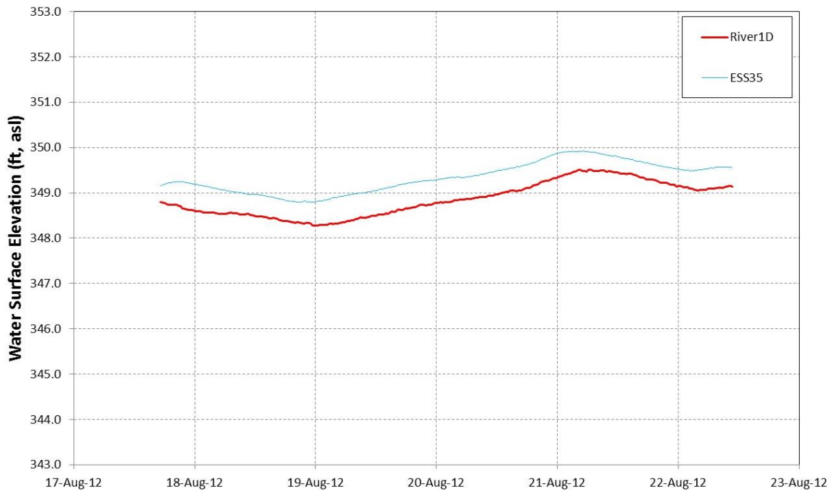
Figure 19: Modelled water levels compared to observed data at PRM 107.1 for Calibration Event 1.
