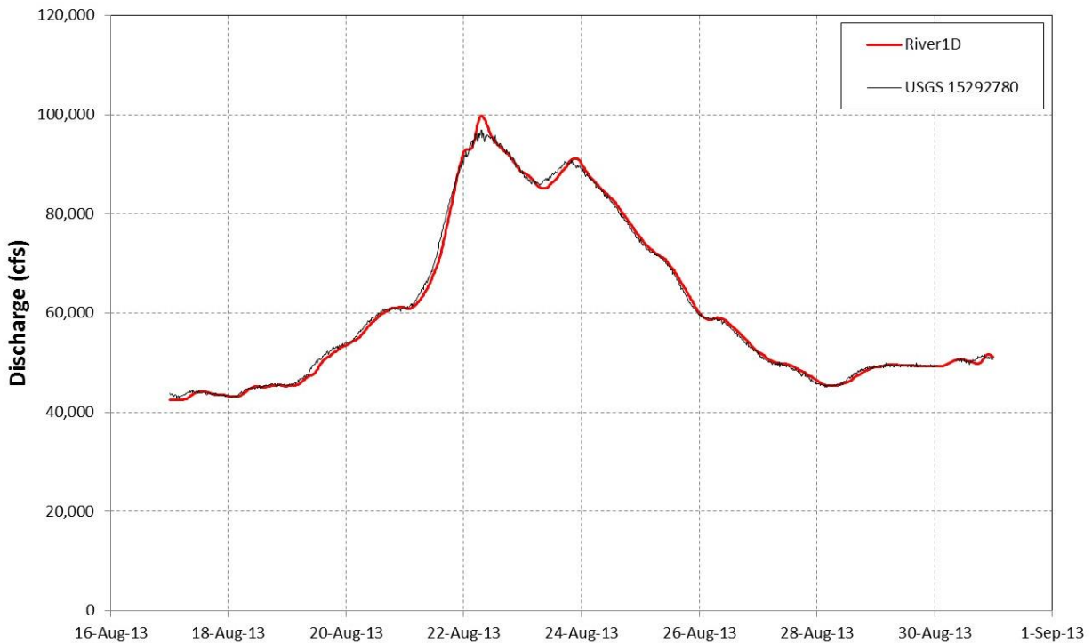
Figure 10. Modelled discharge results compared to observed data at PRM 87.8 for Calibration Event 3.
