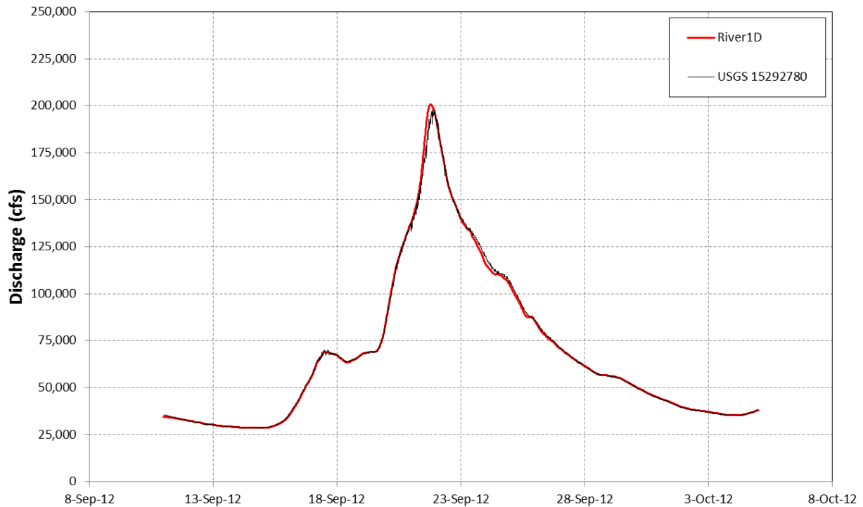
Figure 8. Modelled discharge results compared to observed data at PRM 87.8 for Calibration Event 2.
