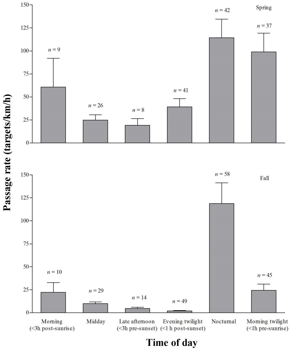
Figure 5.1-6. Passage Rates (mean ± SE) of Targets, Grouped by Time of Day, during Spring and Fall Migration, for Targets Detected within the 1.5-km Radar Range.
