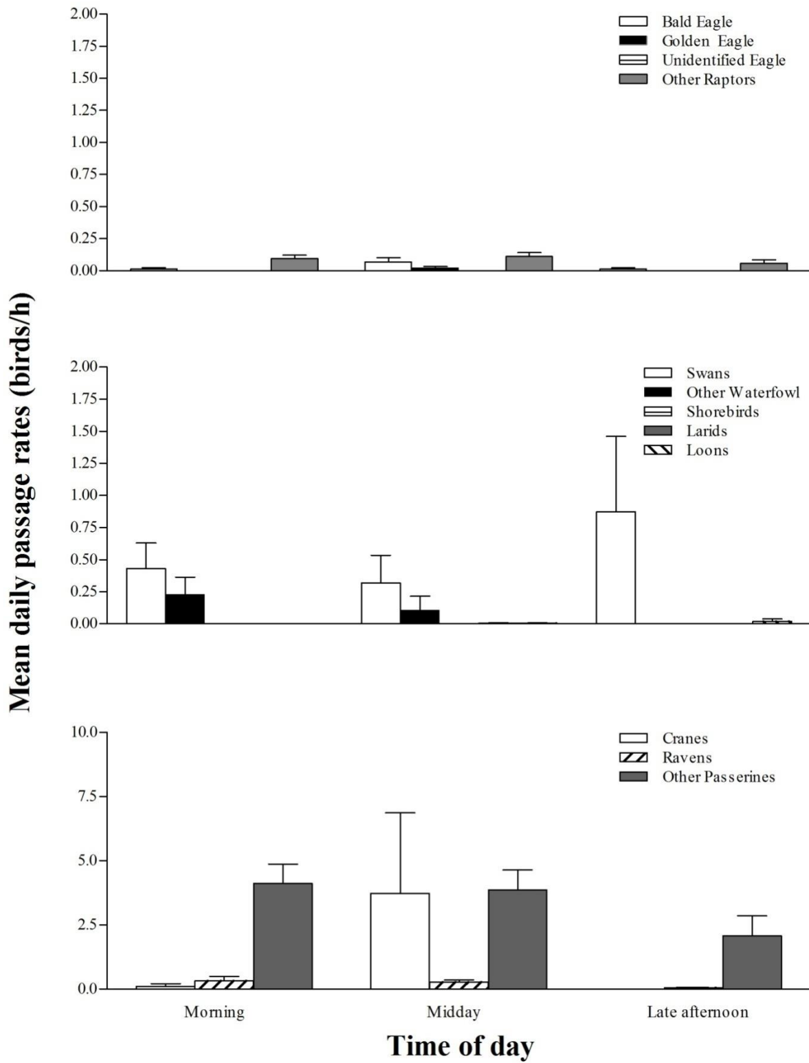
Figure 5.1-21. Mean Movement Rates (birds/h) of Bird Groups by Time of Day during Fall Migration Survey Season.
