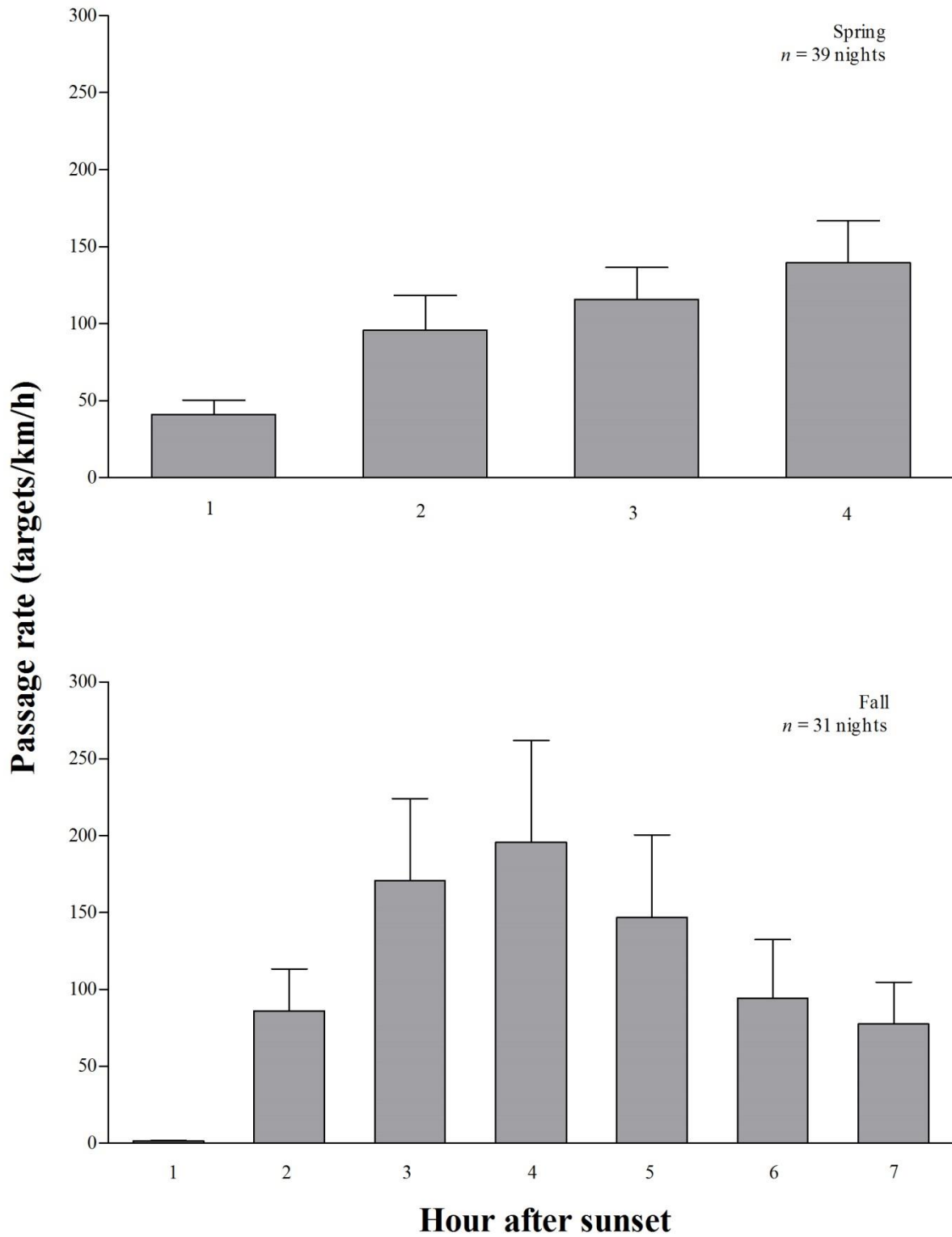
Figure 5.1-7. Passage Rates (mean ± SE) Relative to Hour Post-Sunset During Spring and Fall Migration, for Targets Detected within the 1.5-km Radar Range.
