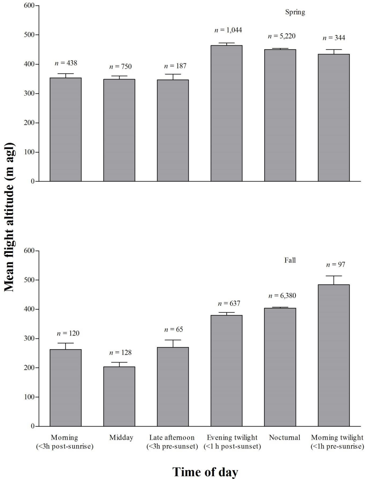
Figure 5.1-11. Mean Flight Altitudes (m agl) of Targets, Grouped by Time of Day, during Spring and Fall Migration for Targets Detected within the 1.5-km Radar Range.
