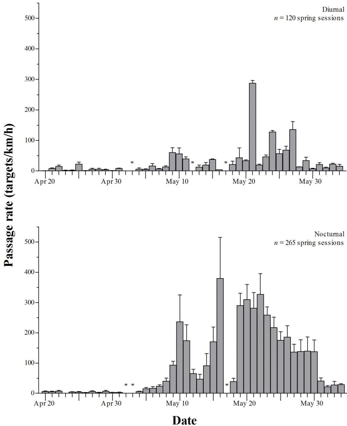
Figure 5.1-5. Spring Diurnal and Nocturnal Passage Rates (mean ± SE) by Date for Targets Detected within the 1.5-km Radar Range. Asterisks indicate that no radar sampling occurred due to weather.
