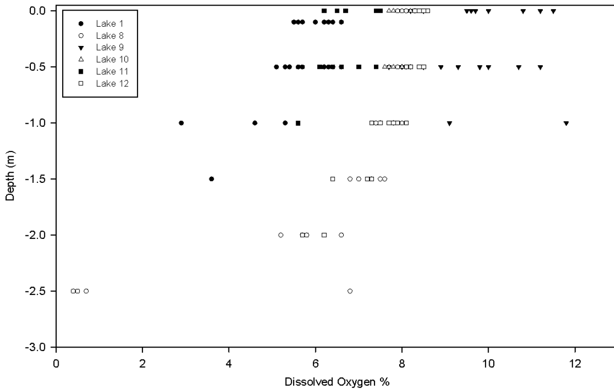
Figure 5.1-3. 2014 dissolved oxygen profiles in Lakes 1-12.
