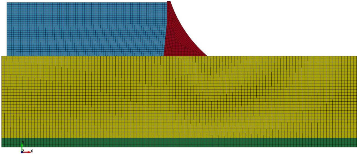
Figure 2 – FEA Mesh in explicit simulation. Reservoir mesh is removed in implicit simulation
