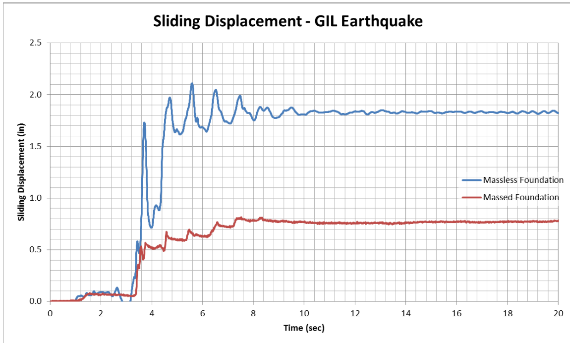
Figure 26 – Sliding Displacement of Dam Monolith
