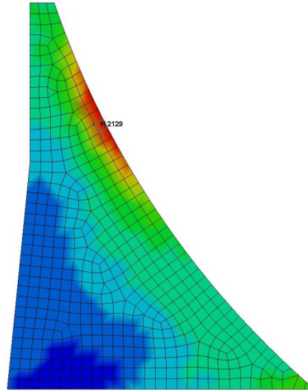
Figure 20 – 1 st Principal Stress at the Moment when it is Maximum on D/S Face of Monolith
