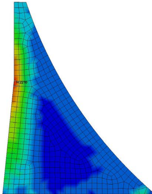
Figure 21 – 1 st Principal Stress at the Moment when it is Maximum on U/S Face of Monolith
