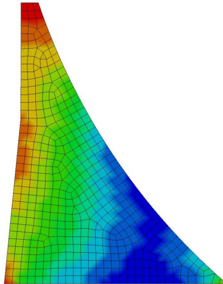
Figure 12 – Static Vertical Stress Distribution in Dam due to Weight of Dam and Reservoir (quasi-static analysis in LS-DYNA)
