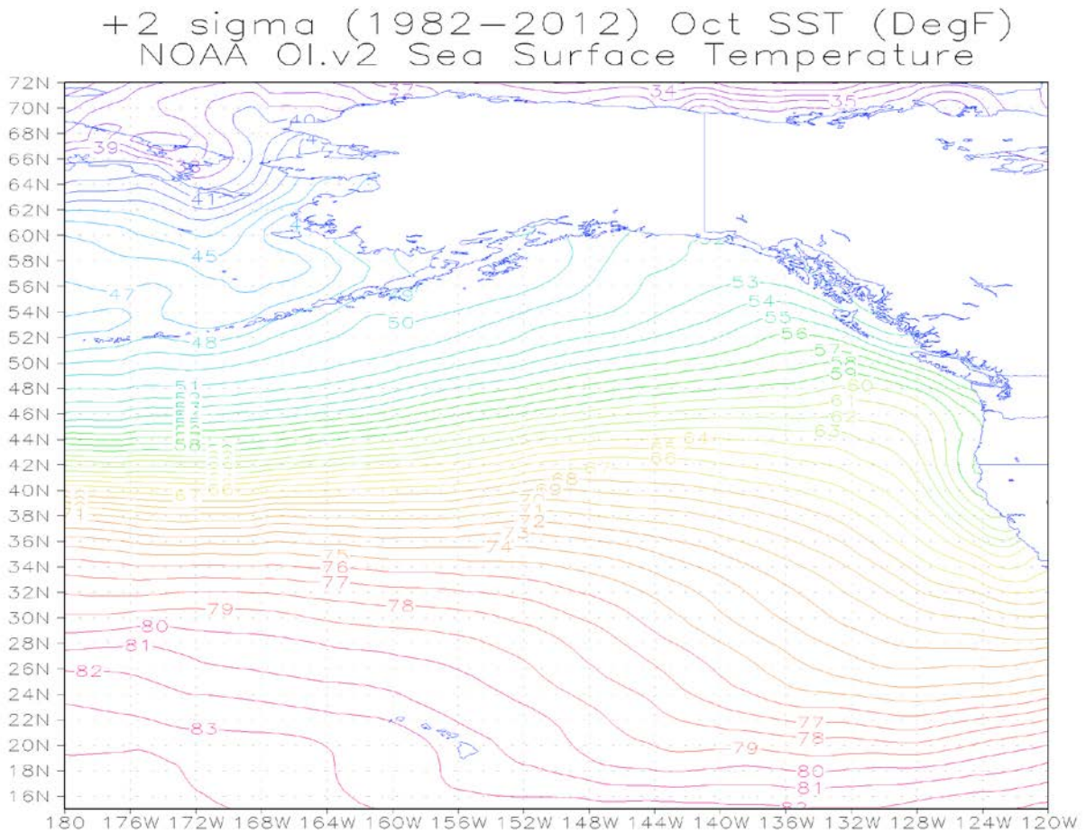
Figure 5.3. +2-sigma sea surface temperature map for October.
