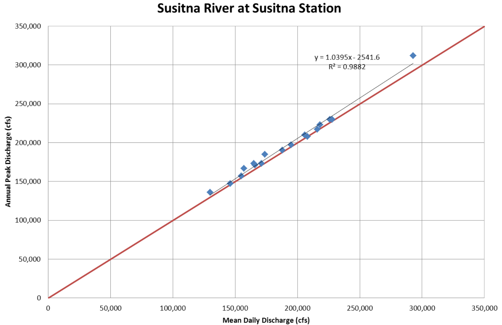
Figure D-11 – Susitna River at Susitna Station regression to extend the Pre-Project USGS available record annual peak data.
