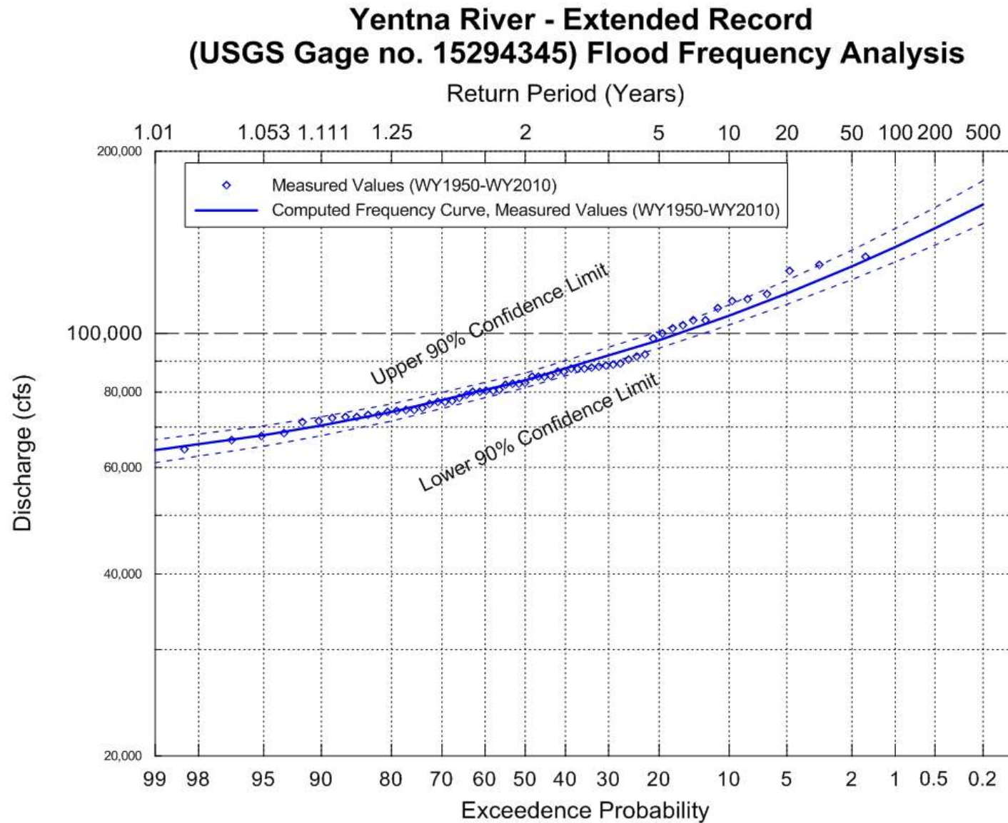
Figure E-10 – Flood Frequency Curve for Yentna River near Susitna Station for Pre-Project Conditions based on the USGS Extended Record
