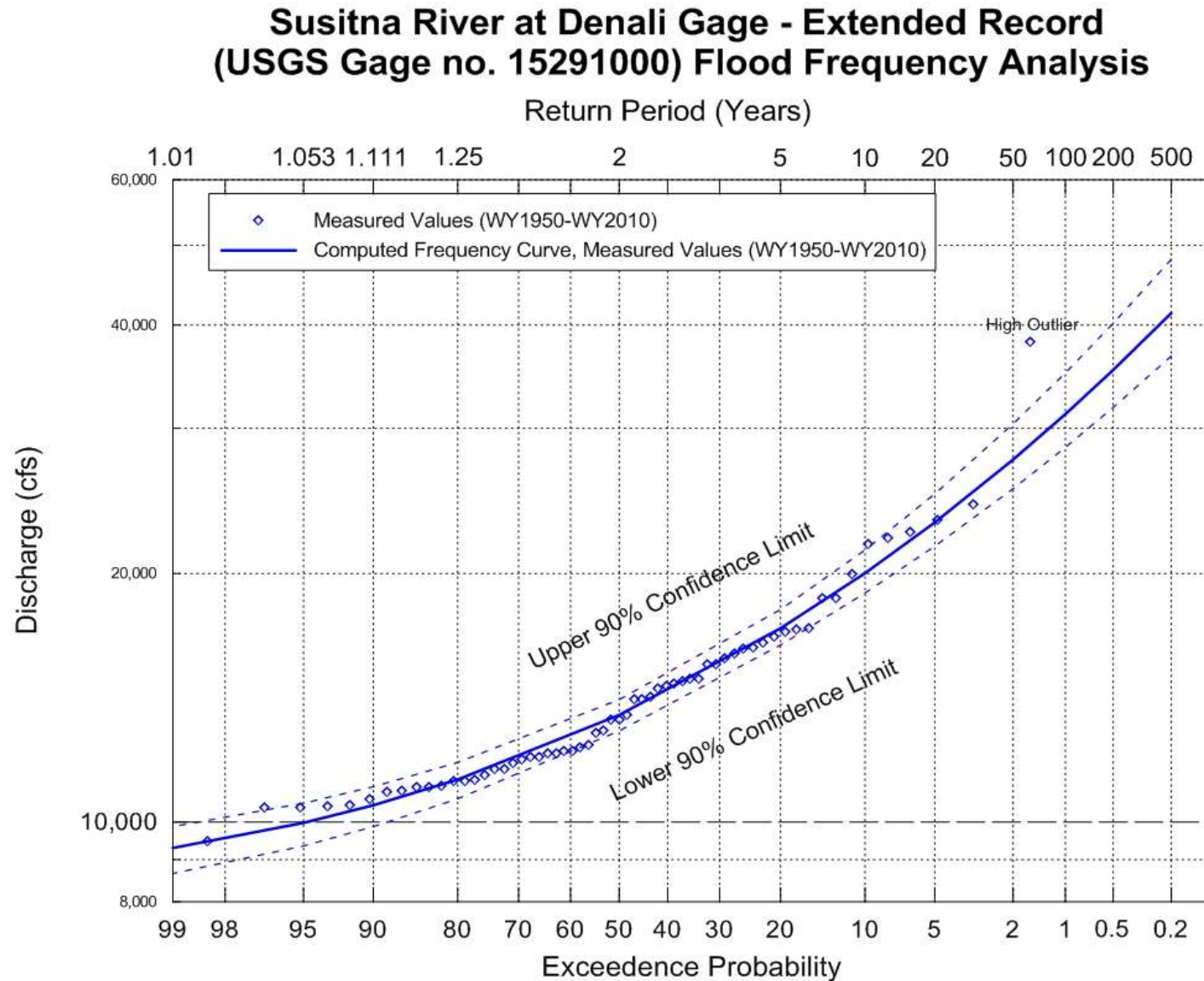
Figure E-1 – Flood Frequency Curve for Susitna River near Denali for Pre-Project Conditions based on the USGS Extended Record
