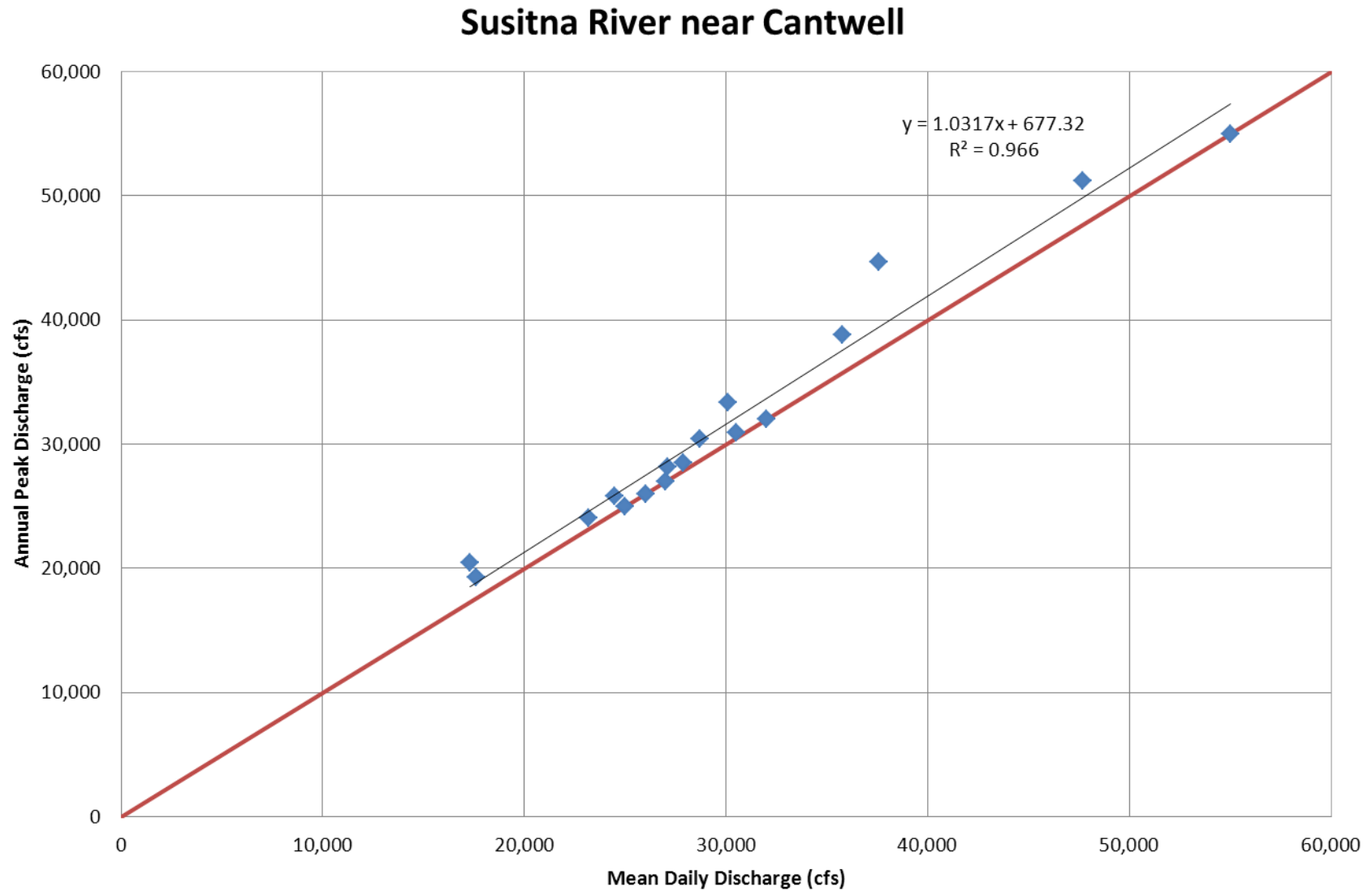
Figure D-3 – Susitna River near Cantwell regression to extend the Pre-Project USGS available record annual peak data.
