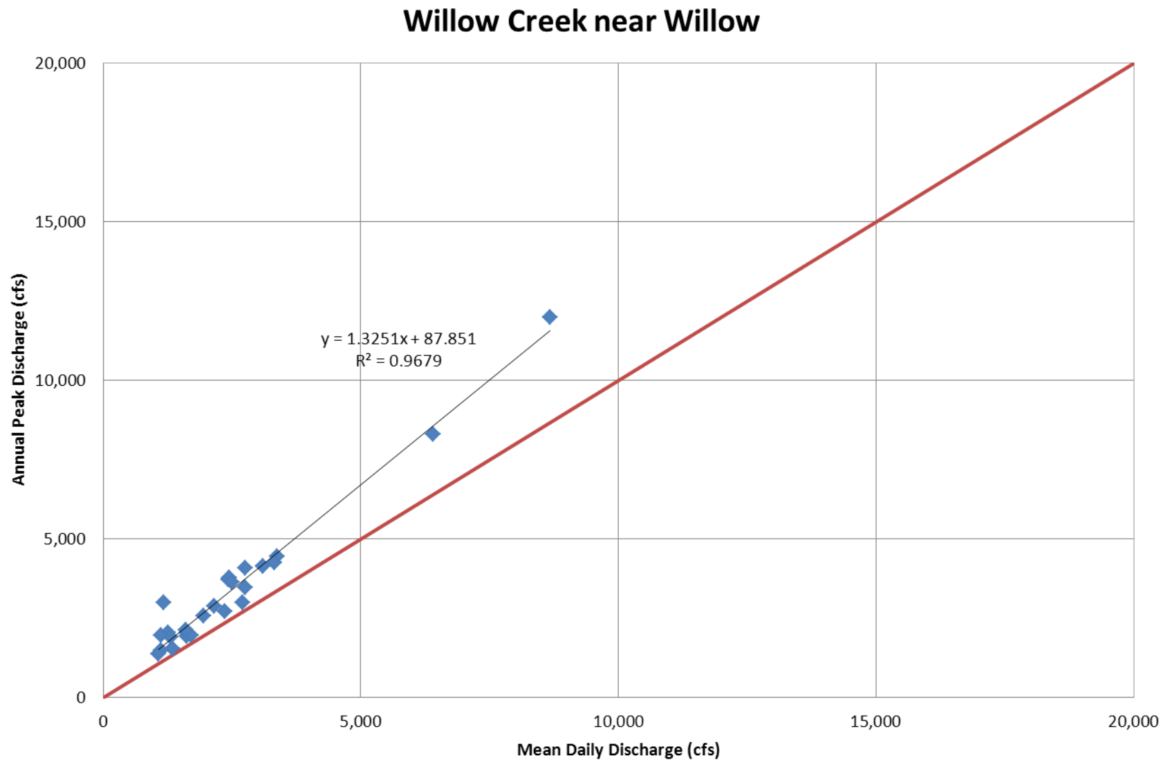
Figure D-8 – Willow Creek near Willow regression to extend the Pre-Project USGS available record annual peak data.
