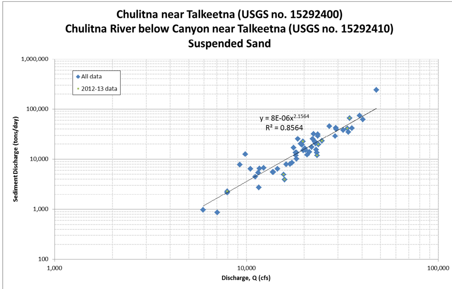
Figure A.6. Suspended sand sediment transport data and rating equation for Chulitna River near Talkeetna and Chulitna River below Canyon near Talkeetna
