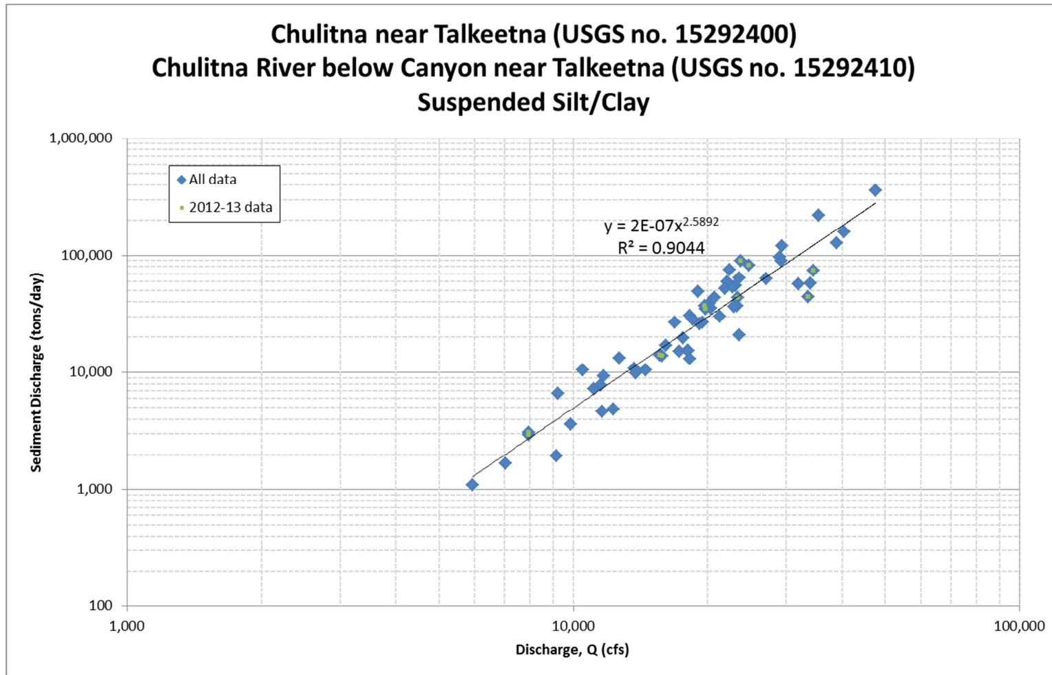
Figure A.5. Suspended silt/clay sediment-transport data and rating equation for Chulitna River near Talkeetna and Chulitna River below Canyon near Talkeetna
