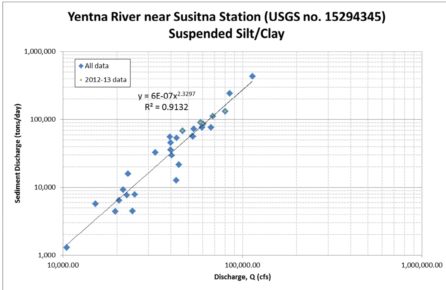
Figure A.17. Suspended silt/clay sediment-transport data and rating equation for Yentna River near Susitna Station
