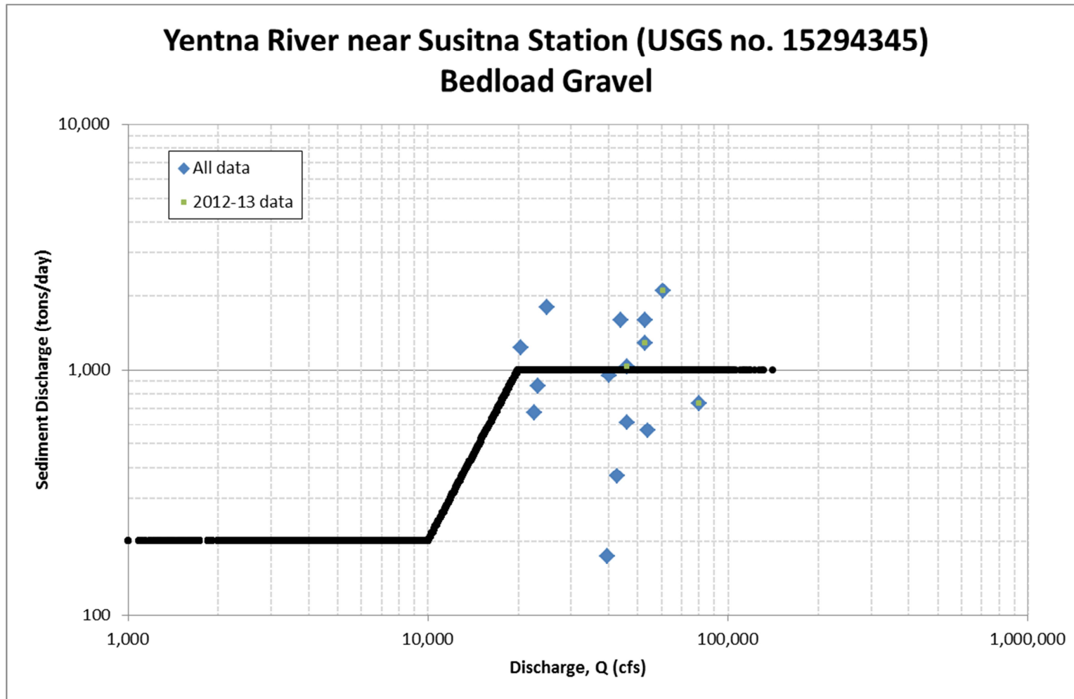
Figure A.20. Bed-load gravel sediment-transport data and rating equation for Yentna River near Susitna Station
