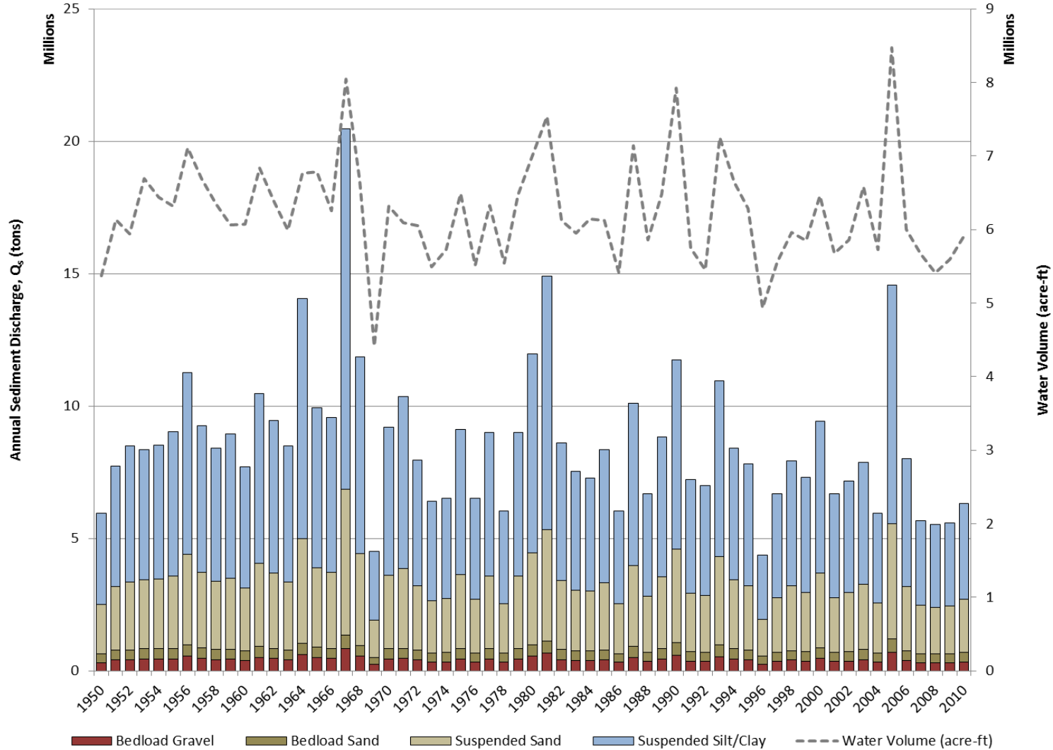
Figure 5.1-4. Estimated annual silt/clay, sand and gravel loads at the Chulitna River near Talkeetna (Gage No. 15292400), Chulitna River below Canyon near Talkeetna (Gage No. 15292410) gage over the 61-year period of flows under pre-Project conditions. Also shown is the annual flow volume for each of the years.
