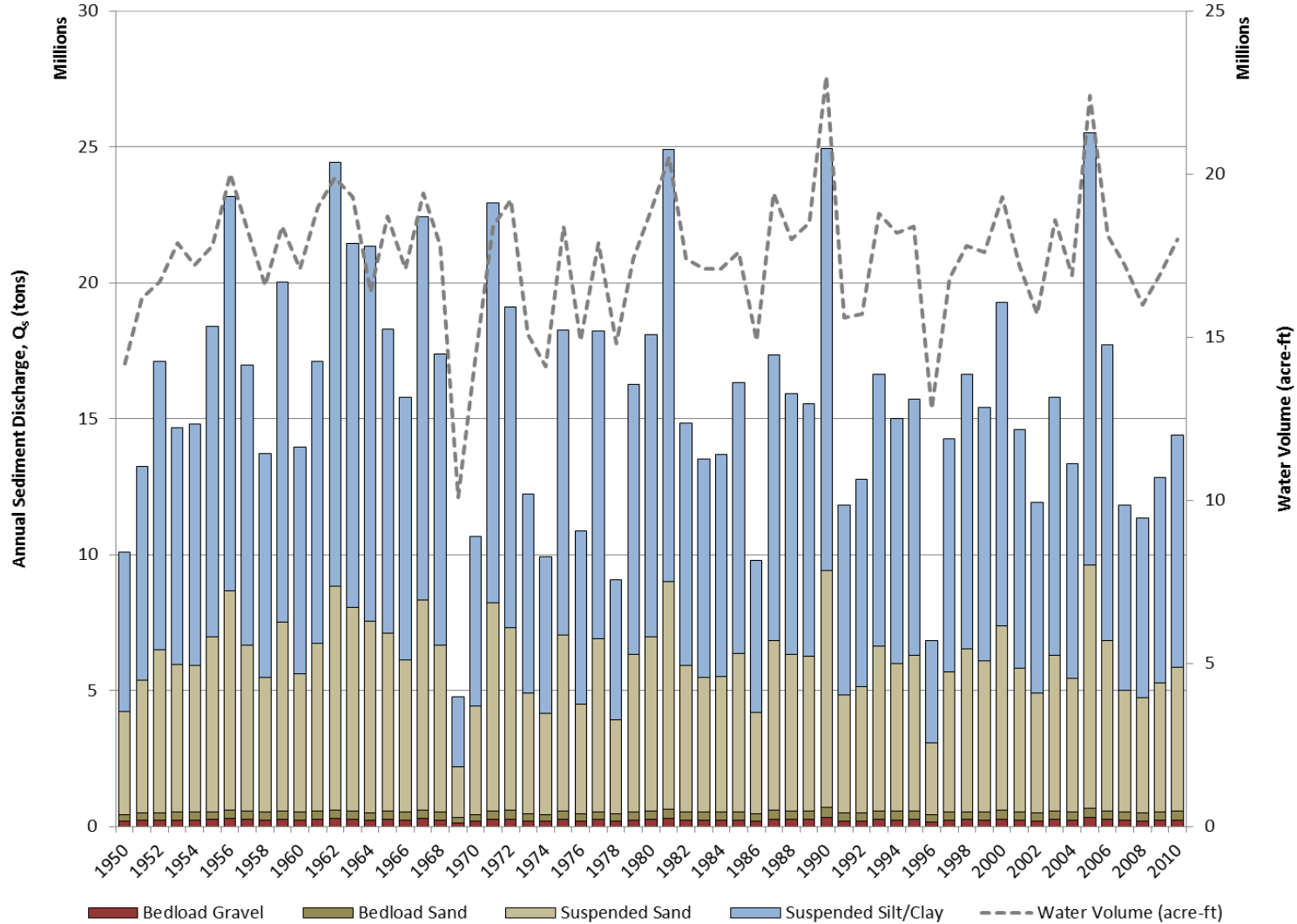
Figure 5.1-2. Estimated annual silt/clay, sand and gravel loads at the Susitna River at Sunshine (Gage No. 15292780) gage over the 61-year period of flows under pre-Project conditions. Also shown is the annual flow volume for each of the years.
