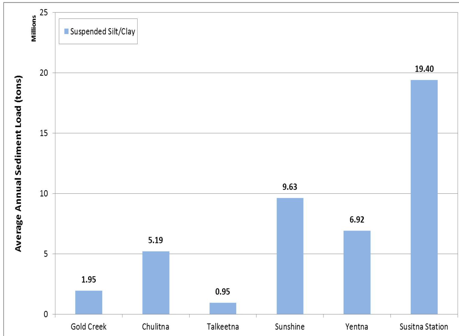
Figure 6.0-1. Average annual silt/clay loads at the three mainstem gages and the three primary tributary gages under pre-Project conditions.
