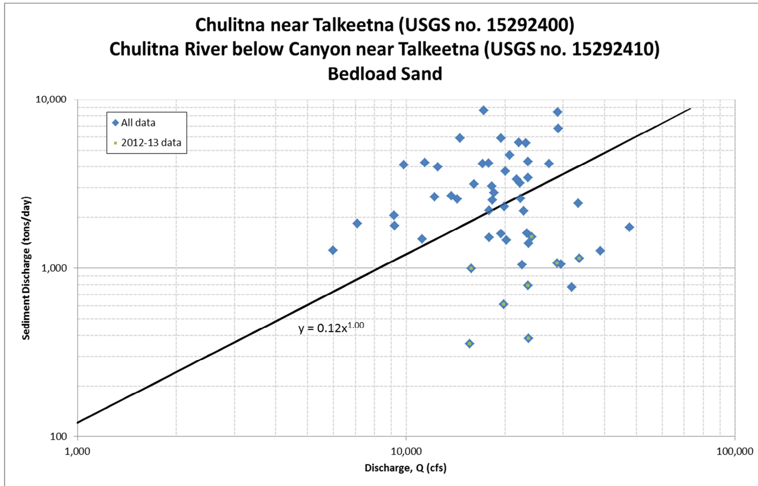
Figure A.7. Bed-load sand sediment-transport data and rating equation for Chulitna River near Talkeetna and Chulitna River below Canyon near Talkeetna
