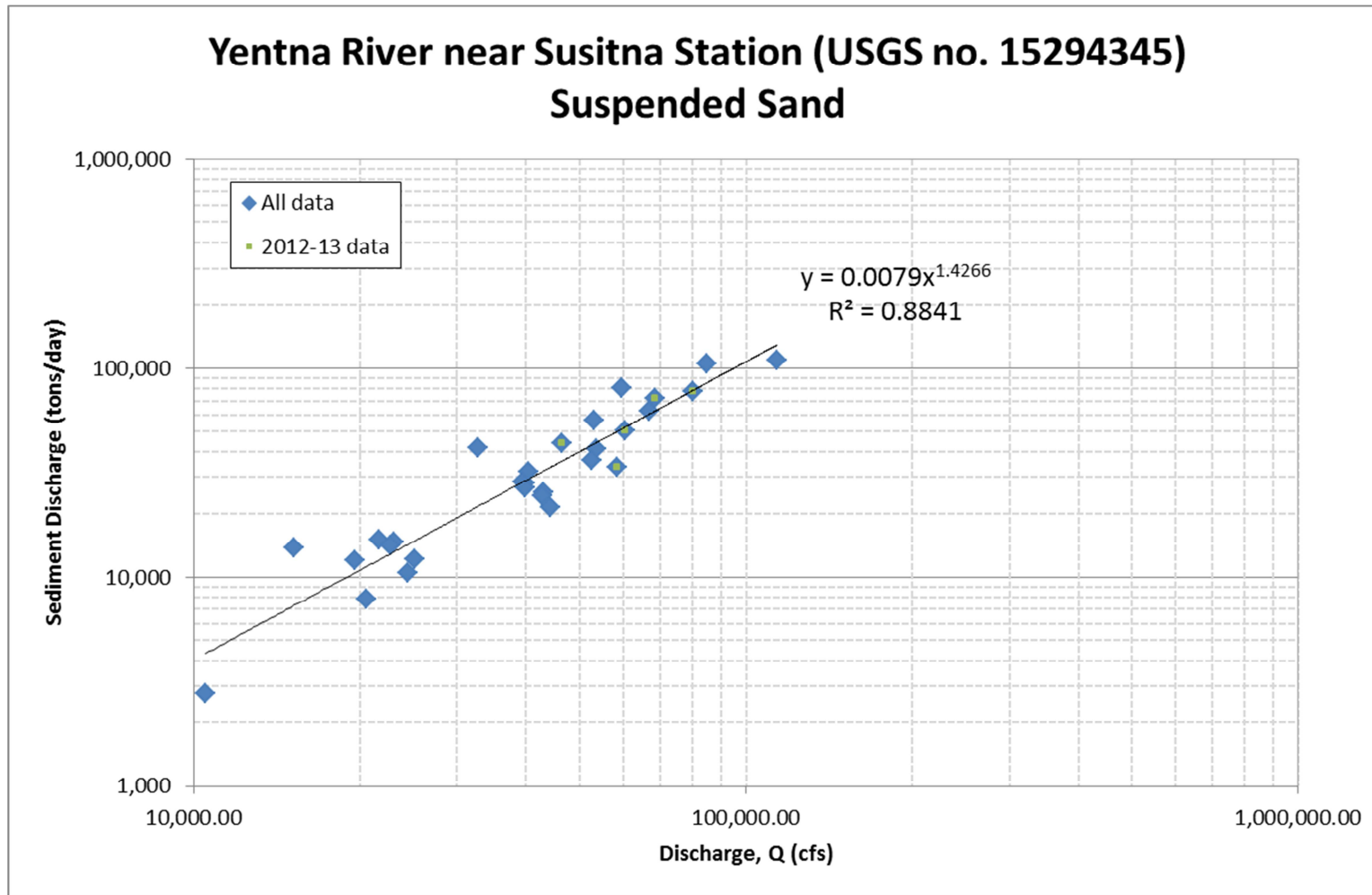
Figure A.18. Suspended sand sediment-transport data and rating equation for Yentna River near Susitna Station
