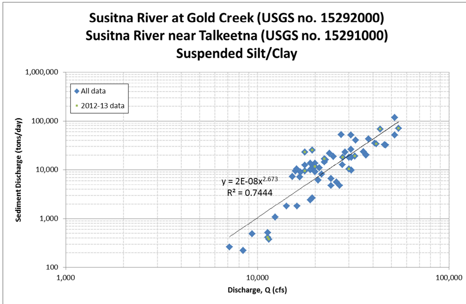
Figure A.1. Suspended silt/clay sediment-transport data and rating equation for Susitna River at Gold Creek and Susitna River near Talkeetna
