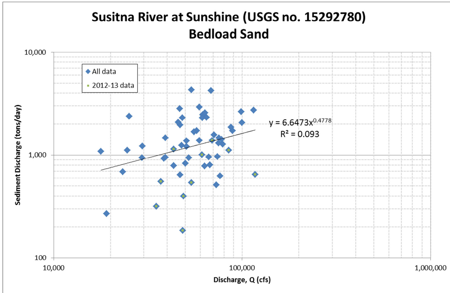
Figure A.15. Bed-load sand sediment-transport data and rating equation for Susitna River at Sunshine
