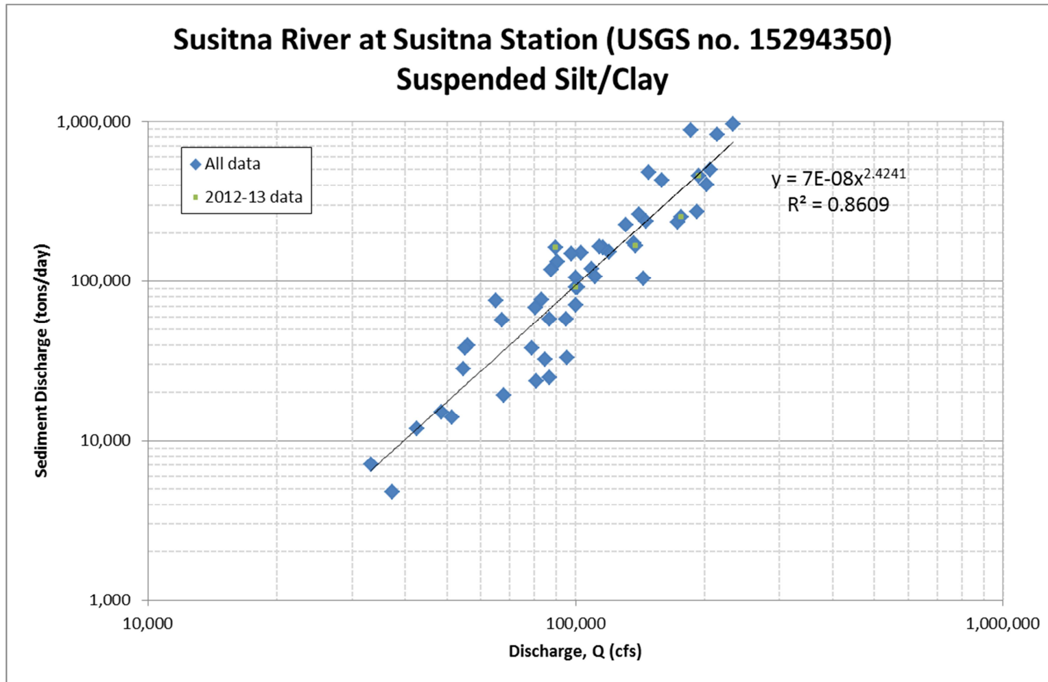
Figure A.21. Suspended silt/clay sediment-transport data and rating equation for Susitna River near Susitna Station
