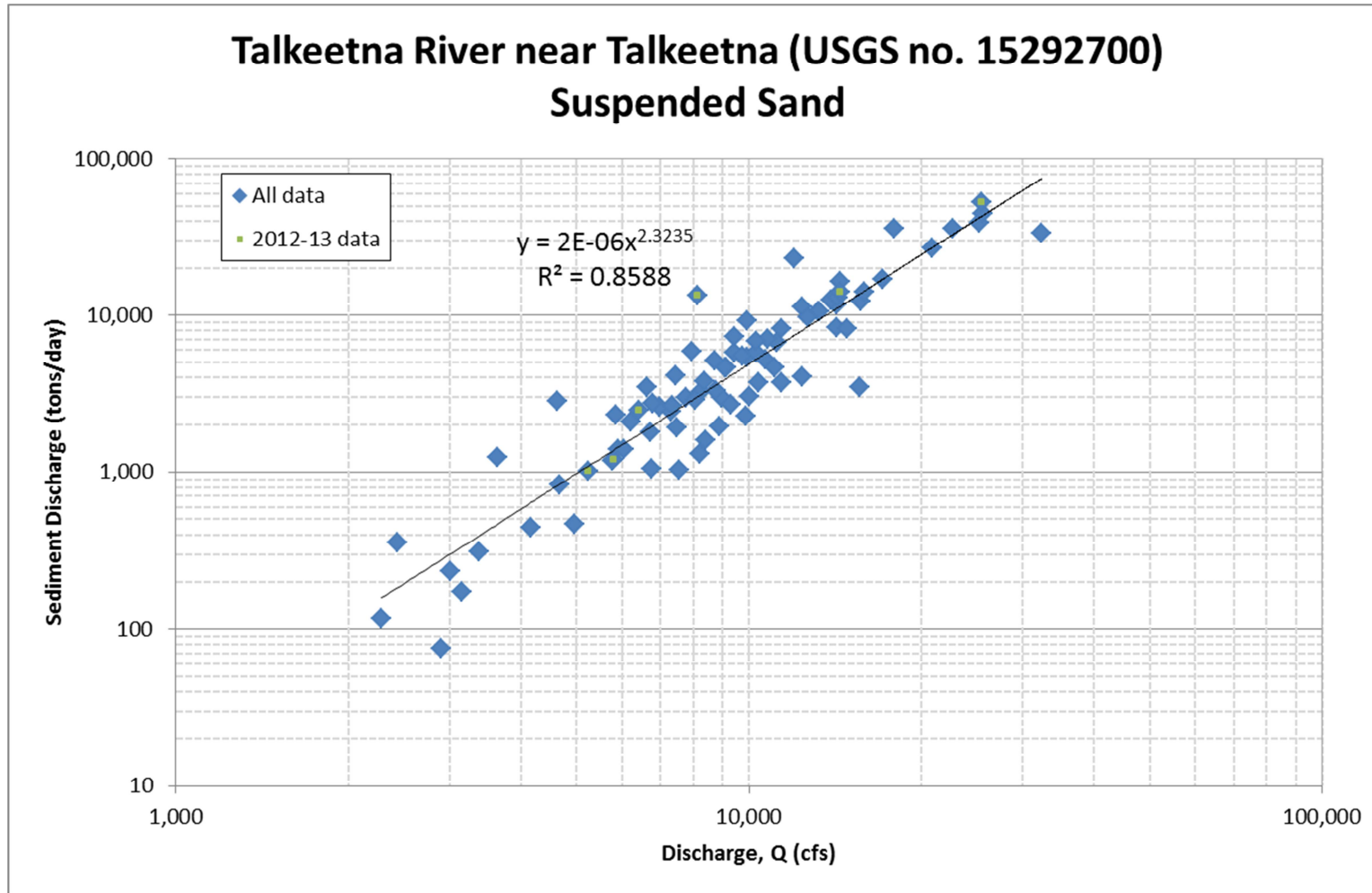
Figure A.10. Suspended sand sediment-transport data and rating equation for Talkeetna River near Talkeetna
