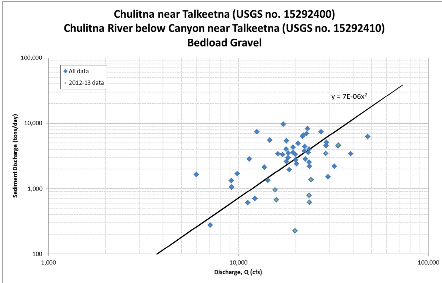
Figure A.8. Bed-load gravel sediment-transport data and rating equation for Chulitna River near Talkeetna and Chulitna River below Canyon near Talkeetna
