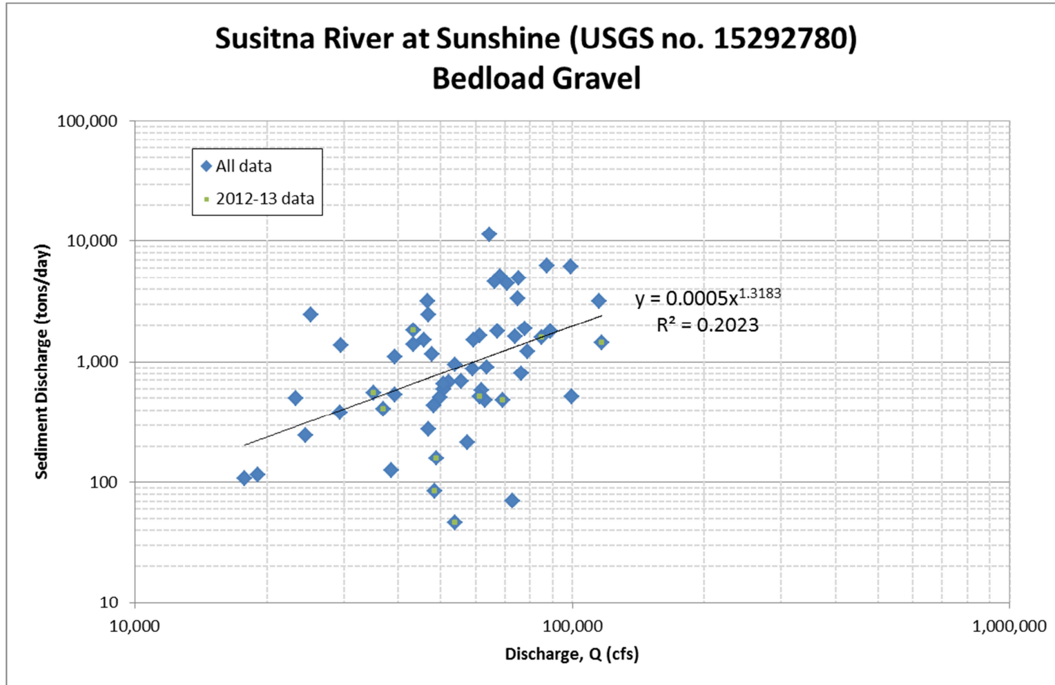
Figure A.16. Bed-load gravel sediment-transport data and rating equation for Susitna River at Sunshine
