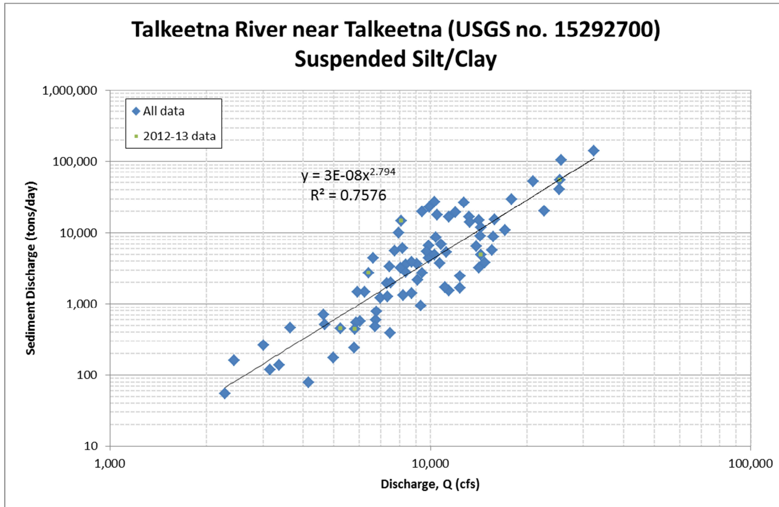
Figure A.9. Suspended silt/clay sediment-transport data and rating equation for Talkeetna River near Talkeetna
