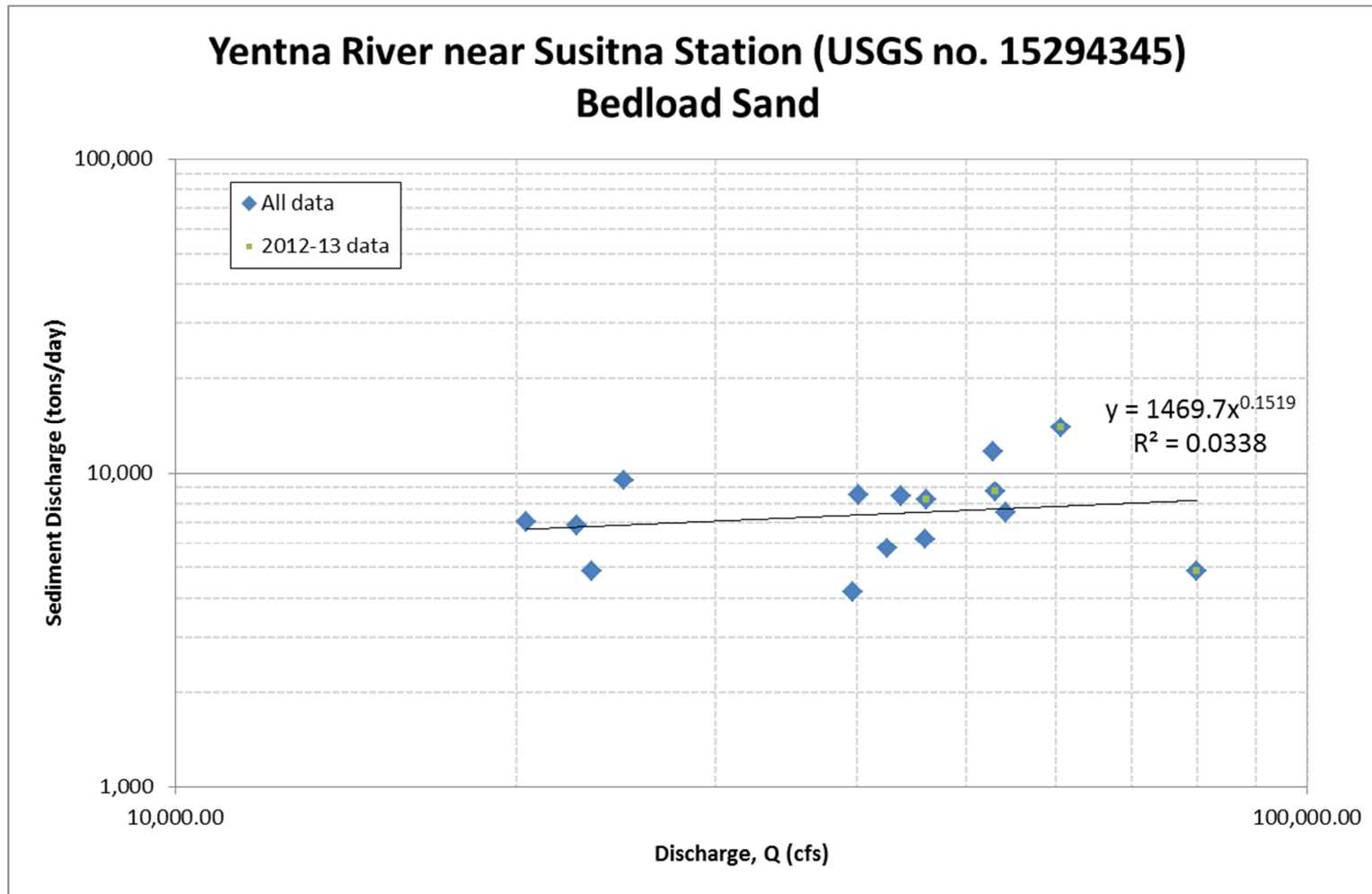
Figure A.19. Bed-load sand sediment-transport data and rating equation for Yentna River near Susitna Station
