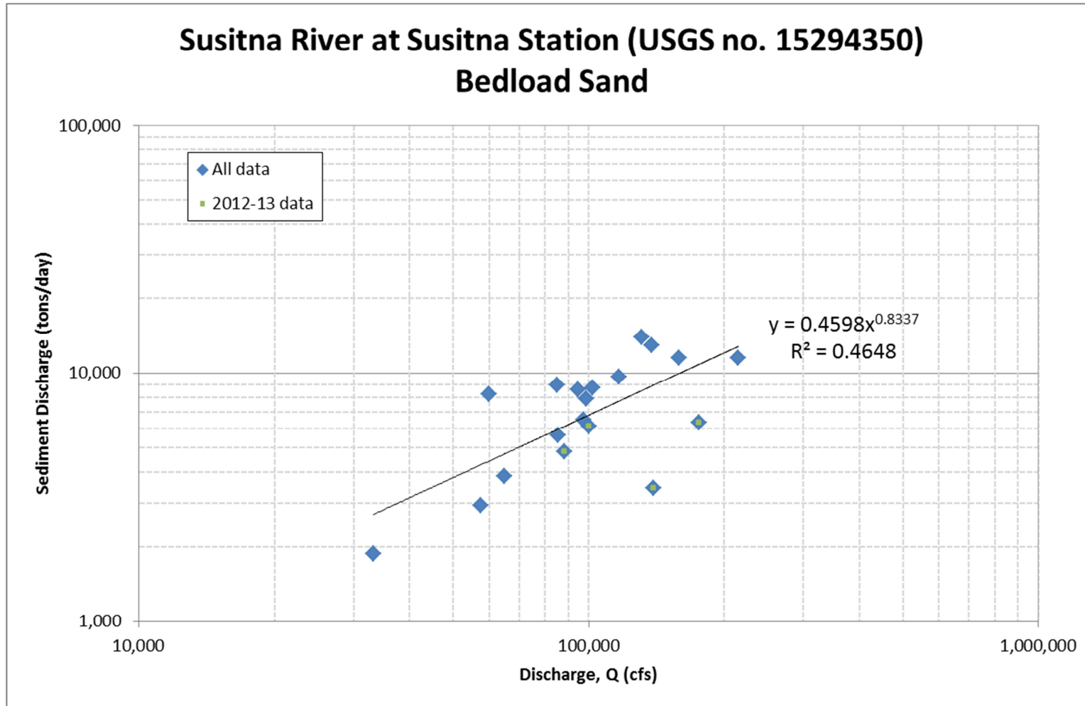
Figure A.23. Bed-load sand sediment-transport data and rating equation for Susitna River near Susitna Station
