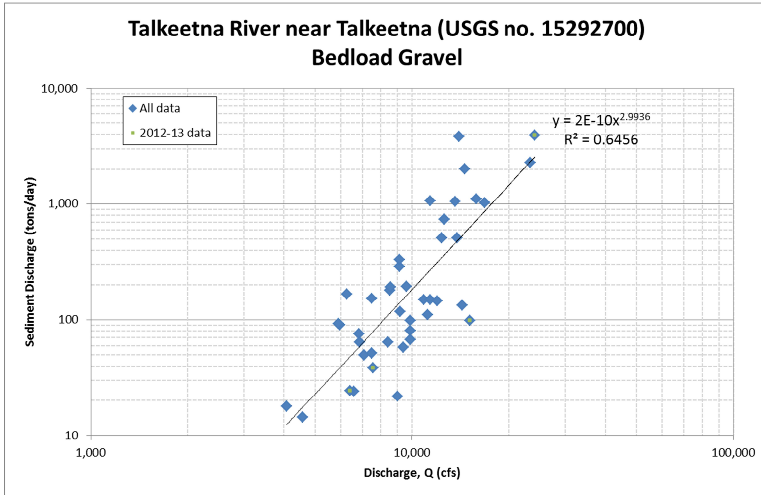
Figure A.12. Bed-load gravel sediment-transport data and rating equation for Talkeetna River near Talkeetna
