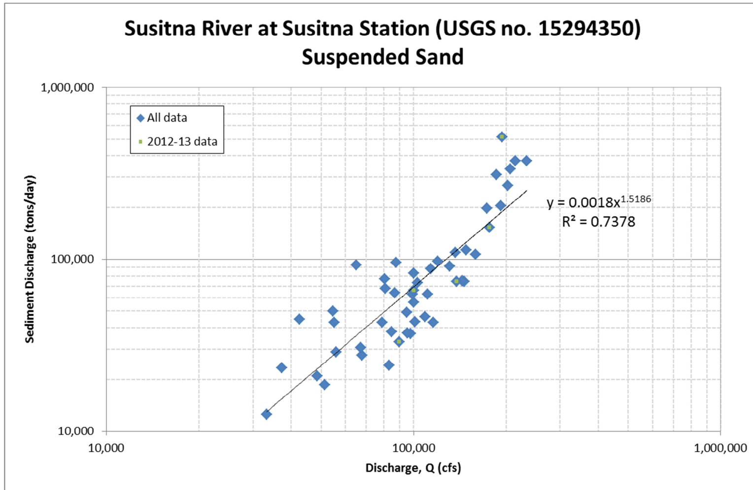
Figure A.22. Suspended sand sediment-transport data and rating equation for Susitna River near Susitna Station
