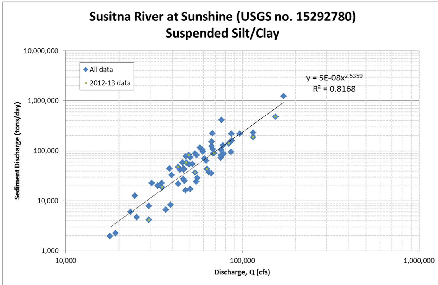
Figure A.13. Suspended silt/clay sediment-transport data and rating equation for Susitna River at Sunshine
