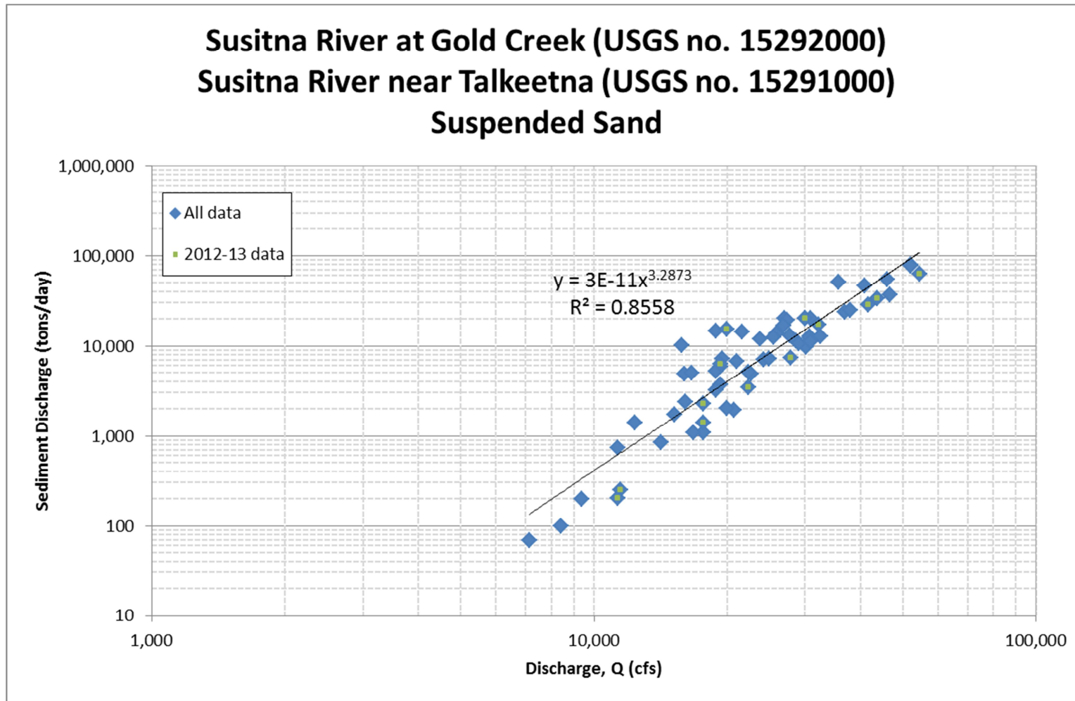
Figure A.2. Suspended sand sediment-transport data and rating equation for Susitna River at Gold Creek and Susitna River near Talkeetna
