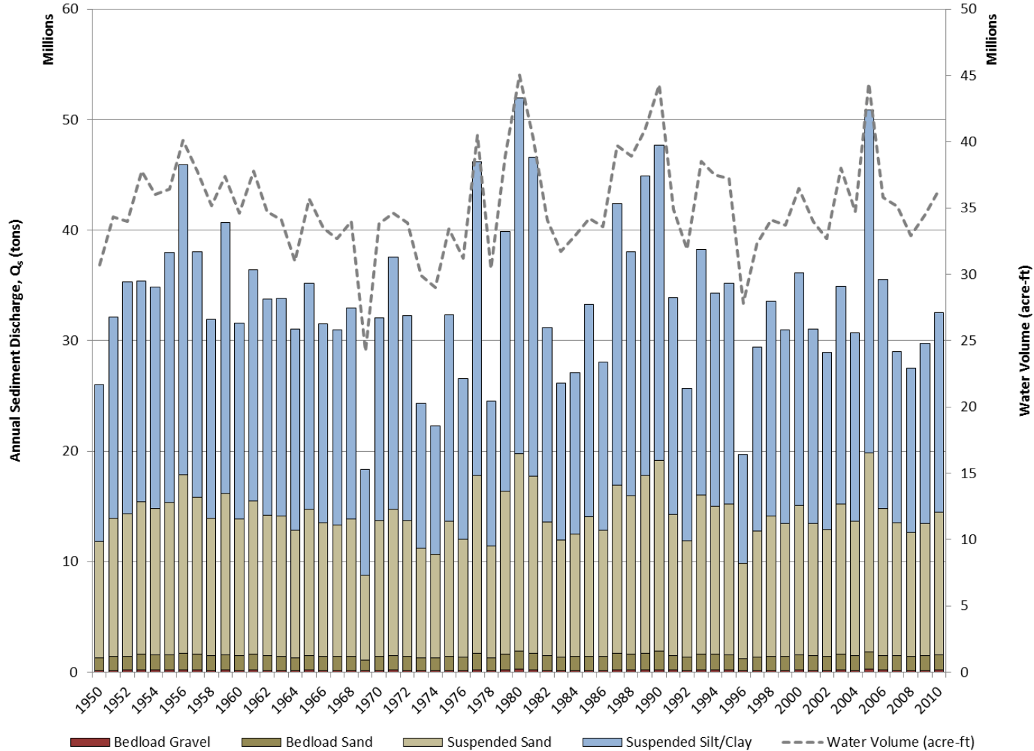
Figure 5.1-3. Estimated annual silt/clay, sand and gravel loads at the Susitna River at Susitna Station (Gage No. 15294350) gage over the 61-year period of flows under pre-Project conditions. Also shown is the annual flow volume for each of the years.
