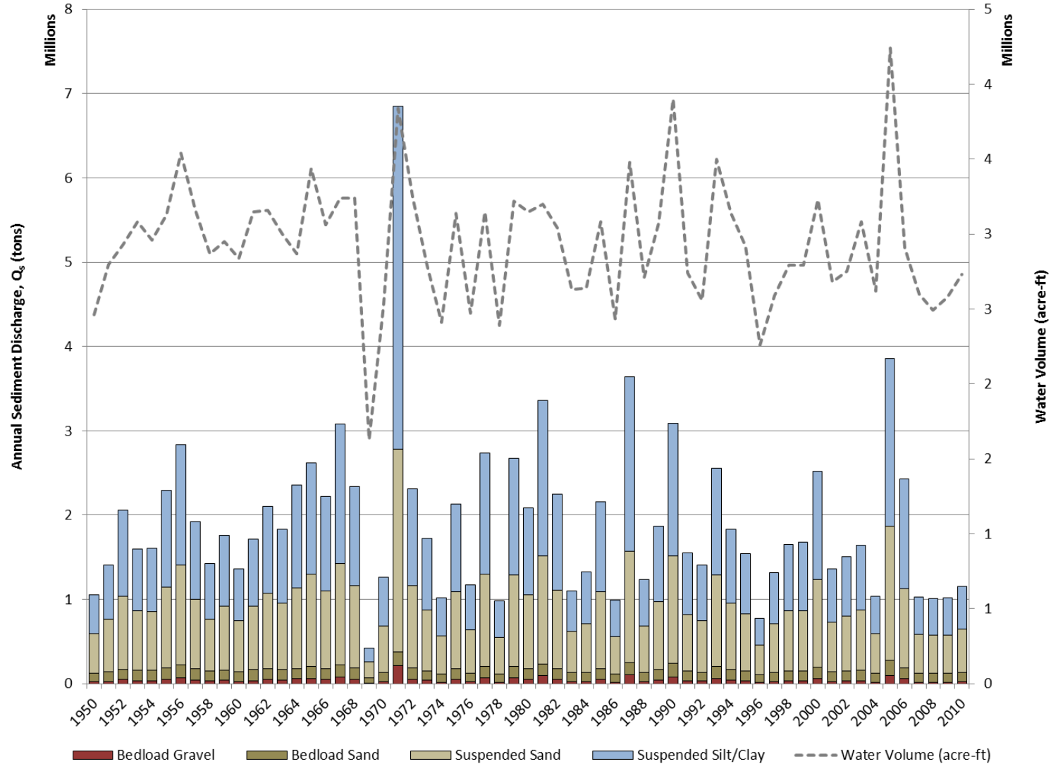
Figure 5.1-5. Estimated annual silt/clay, sand and gravel loads at the Talkeetna River near Talkeetna (Gage No. 15292700) gage over the 61-year period of flows under pre-Project conditions. Also shown is the annual flow volume for each of the years.
