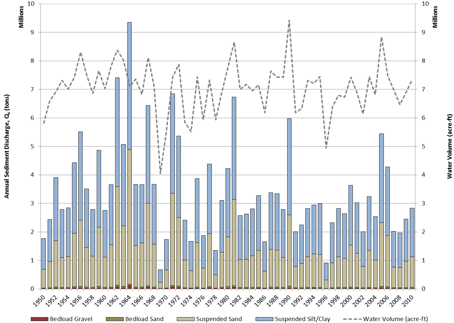
Figure 5.1-1. Estimated annual silt/clay, sand and gravel loads at the Gold Creek (Gage No. 15292000)/, Susitna River near Talkeetna (Gage No. 15292100) gage over the 61-year period of flows under pre-Project conditions. Also shown is the annual flow volume for each of the years.
