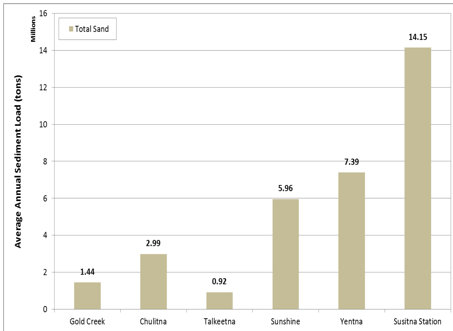
Figure 6.0-2. Average annual sand loads at the three mainstem gages and the three primary tributary gages under pre-Project conditions.
