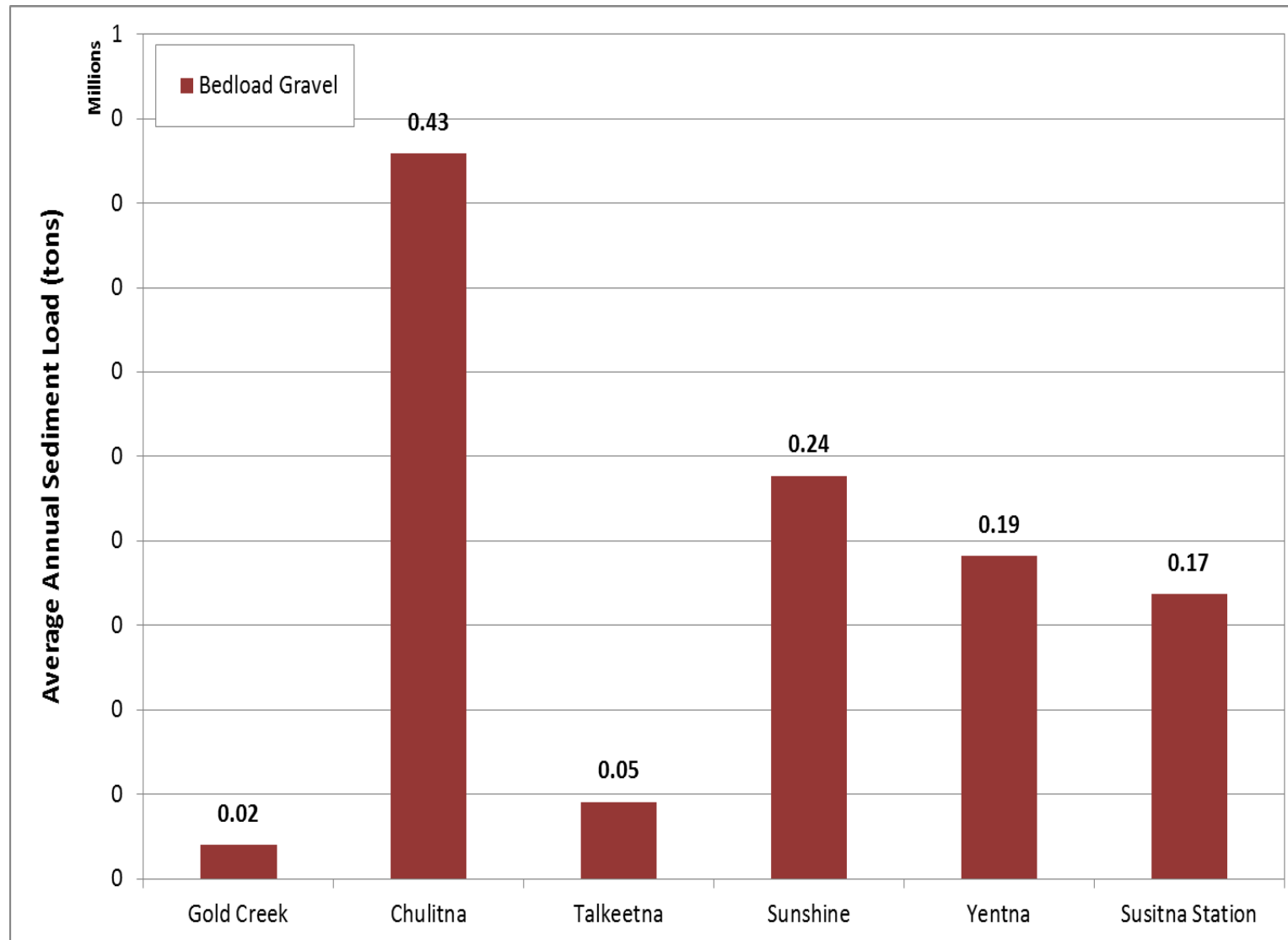
Figure 6.0-3. Average annual gravel loads at the three mainstem gages and the three primary tributary gages under pre-Project conditions.
