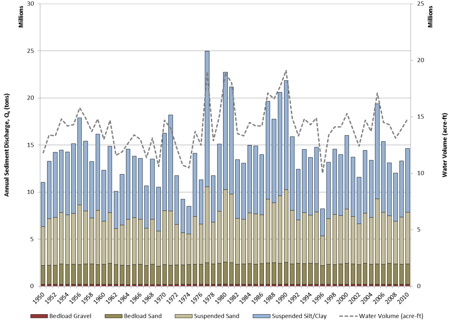
Figure 5.1-6. Estimated annual silt/clay, sand and gravel loads at the Yentna River near Susitna Station (Gage No. 15294345) gage over the 61-year period of flows under pre-Project conditions. Also shown is the annual flow volume for each of the years.
