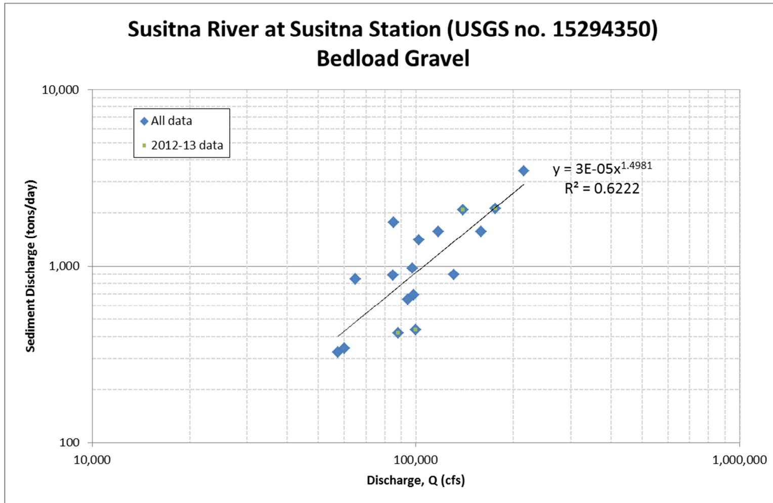
Figure A.24. Bed-load gravel sediment-transport data and rating equation for Susitna River near Susitna Station
