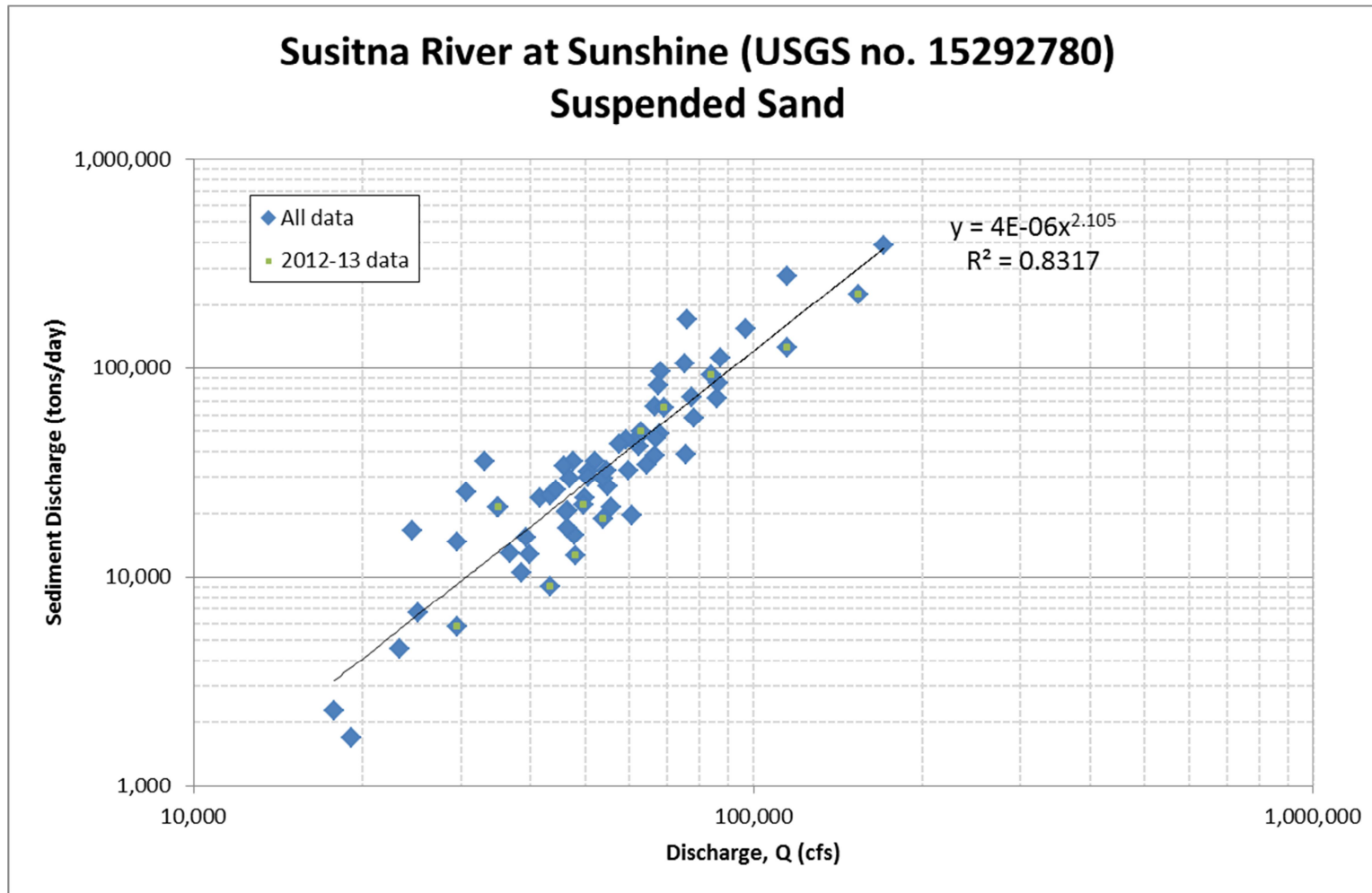
Figure A.14. Suspended sand sediment-transport data and rating equation for Susitna River at Sunshine
