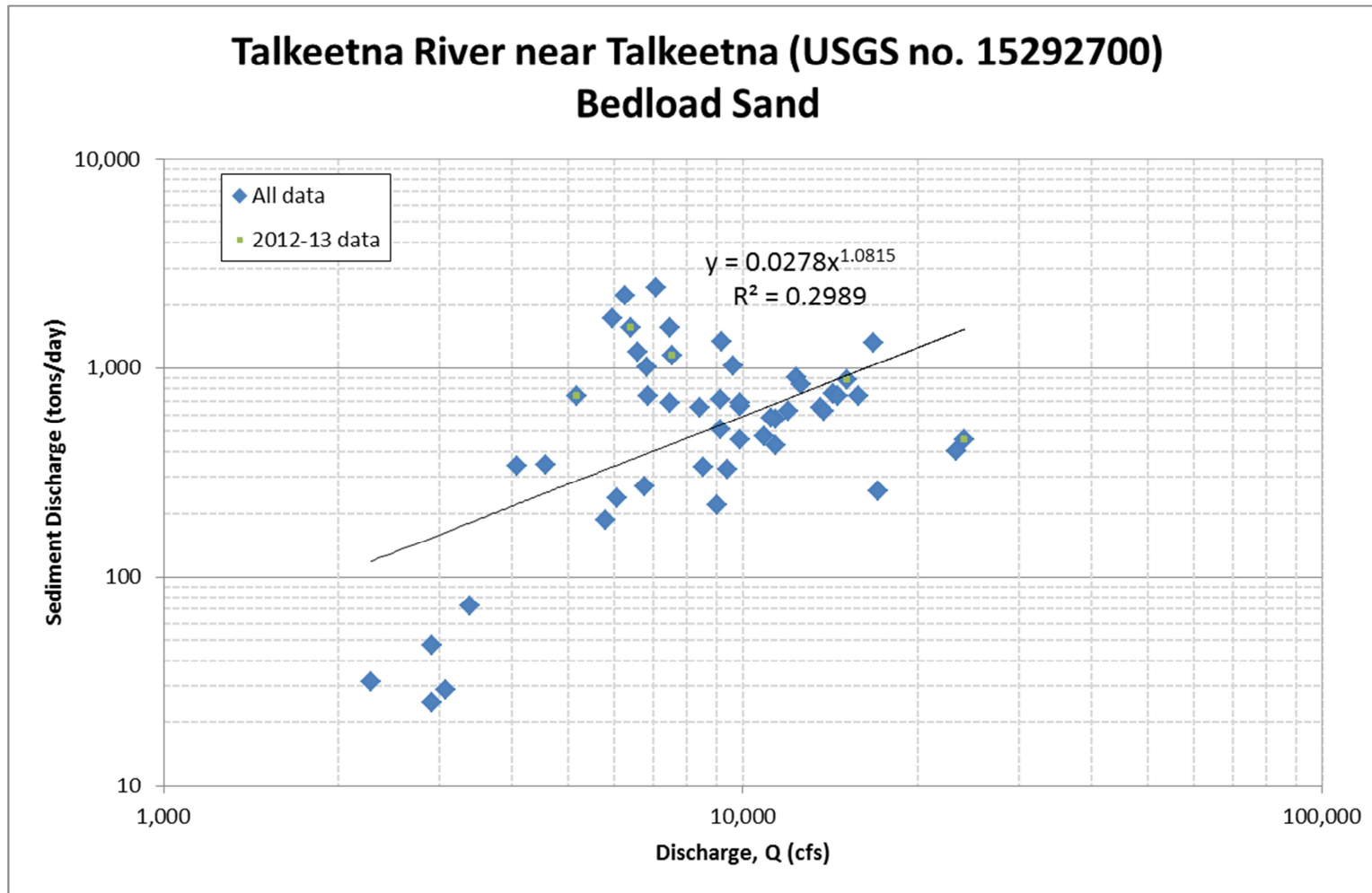
Figure A.11. Bed-load sand sediment-transport data and rating equation for Talkeetna River near Talkeetna
