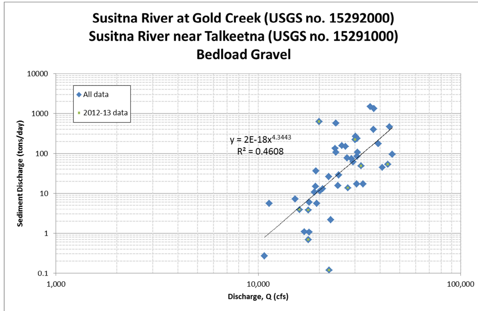
Figure A.4. Bed-load gravel sediment-transport data and rating equation for Susitna River at Gold Creek and Susitna River near Talkeetna
