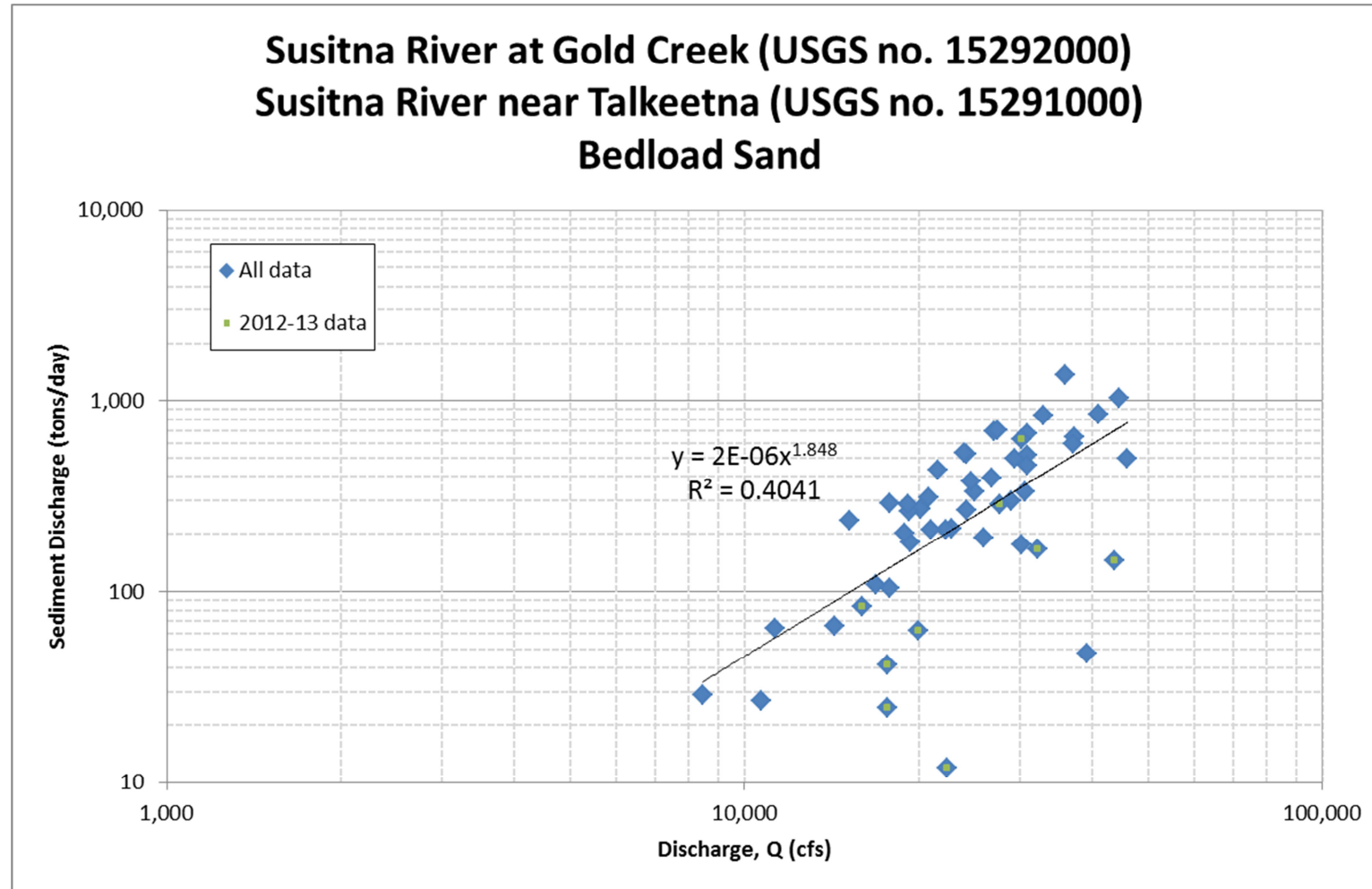
Figure A.3. Bed-load Sand sediment-transport data and rating equation for Susitna River at Gold Creek and Susitna River near Talkeetna
