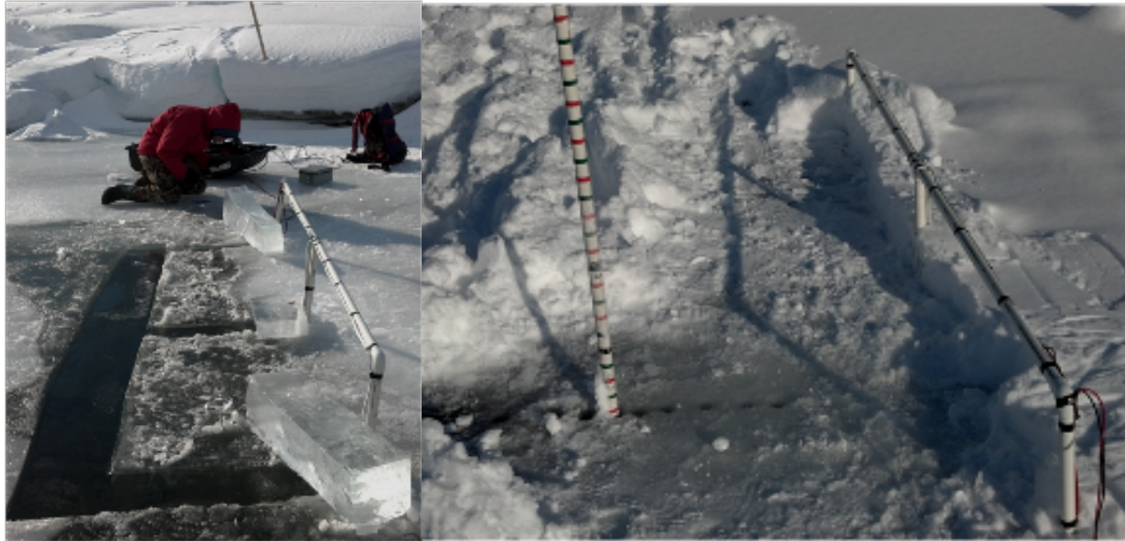
Figure C4.2-1. Swim-through test antenna installation through ice (L) and read distance testing following re-freeze (R).
