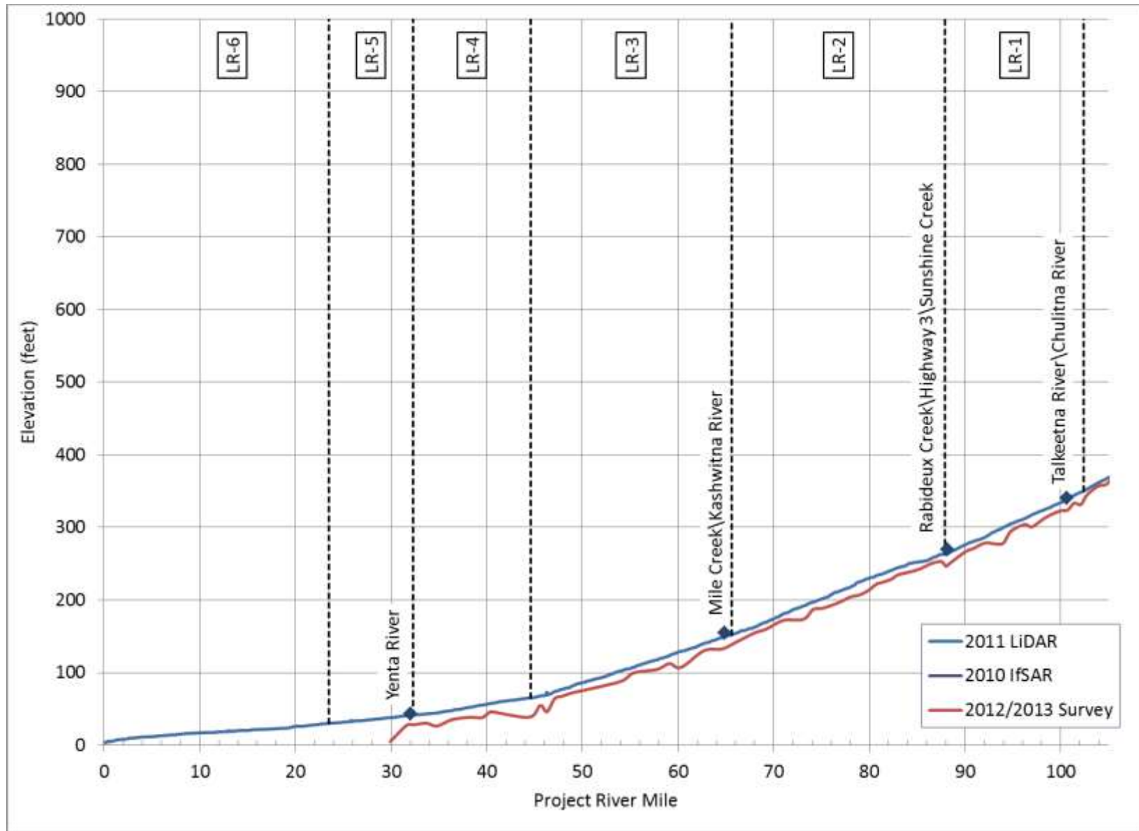
Figure 5.5-2 Longitudinal Profile of Susitna River in Lower River Segment. Sources of data are shown on the figure. Reach boundaries are also included.
