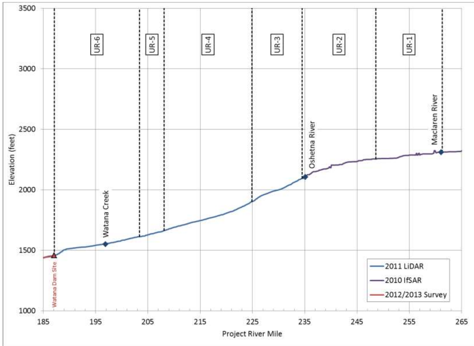
Figure 5.3-2 Longitudinal Profile of Susitna River in Upper River segment. Data Sources are shown on the figure. Reach boundaries are also included.
