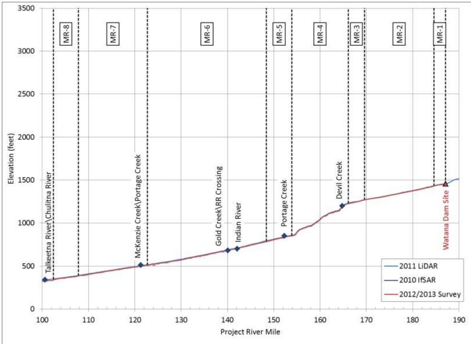
Figure 5.4-2 Longitudinal Profile of Susitna River in Middle River segment. Data sources are shown on the figure. Reach boundaries are also included.
