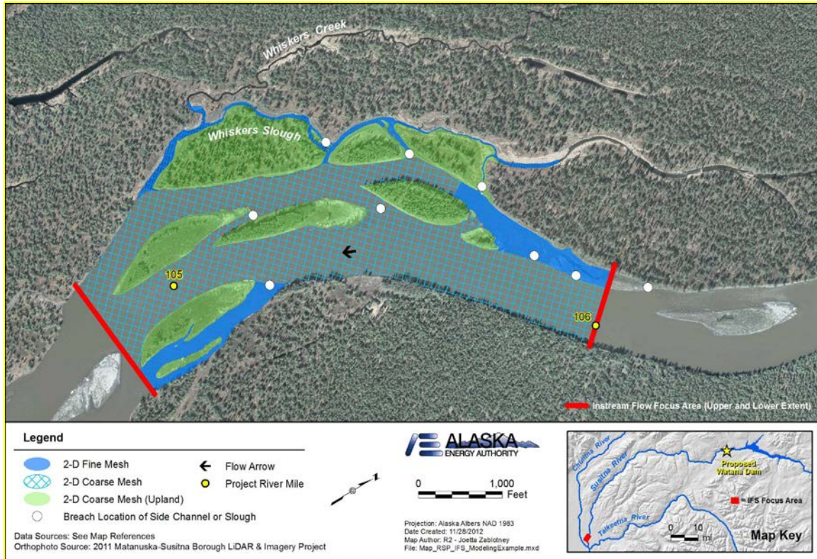
Figure 4-26. Examples of mesh detail for habitat analysis requirements.
