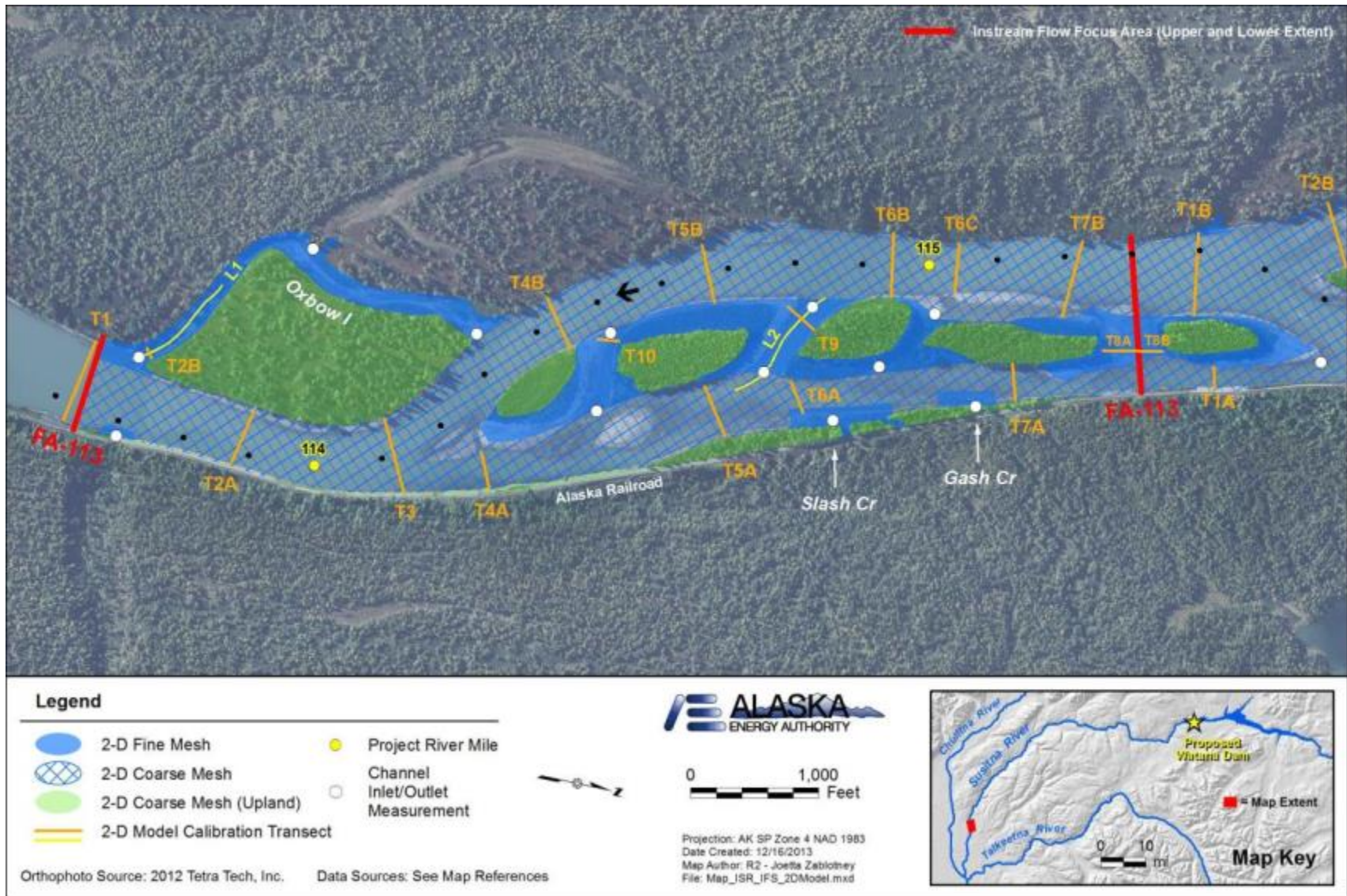
Figure 5.6-2. FA-113 (Oxbow 1) showing fine and course mesh overlays, channel inlet and outlet measurement locations, and alignment of 2013 calibration transects.
