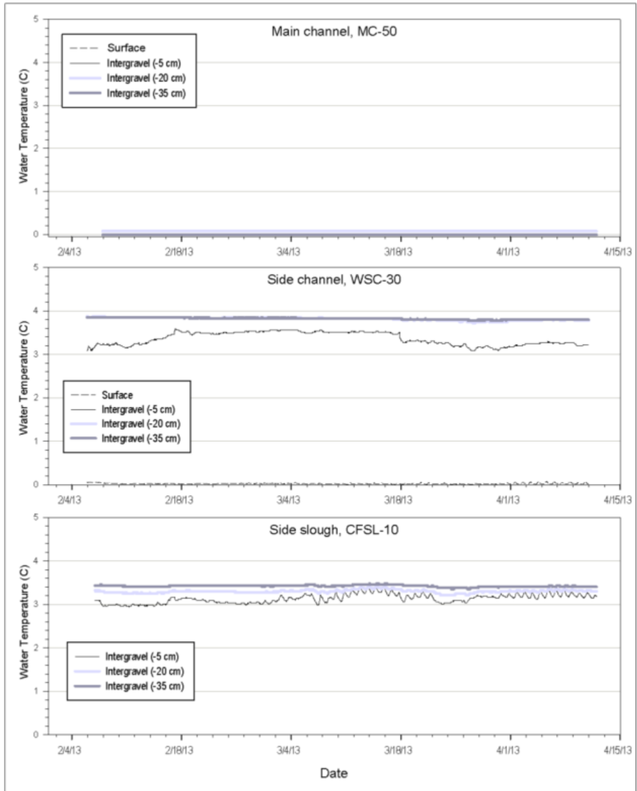
Figure 5.5-13. Water temperature recorded above the substrate surface and at intergravel depths of 5 cm, 20 cm, and 35 cm at main channel (MC-50), side channel (WSC-30) and side slough (CFSL-10) continuous monitoring sites in FA-104 (Whiskers Slough) during February - April 2013. Habitat designations are based on 2012 Middle Susitna River remote line habitat mapping (HDR 2013).
