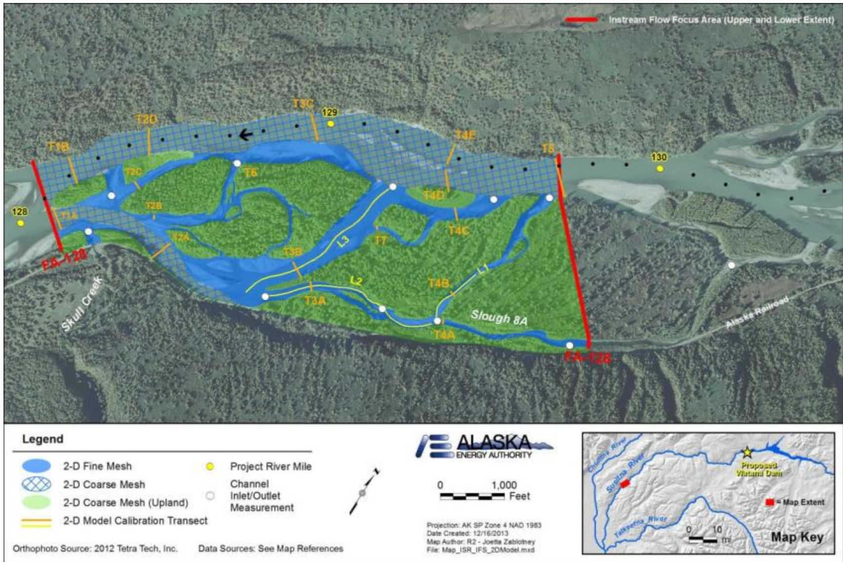
Figure 5.6-4. FA-128 (Slough 8A) showing fine and course mesh overlays, channel inlet and outlet measurement locations, and alignment of 2013 calibration transects.
