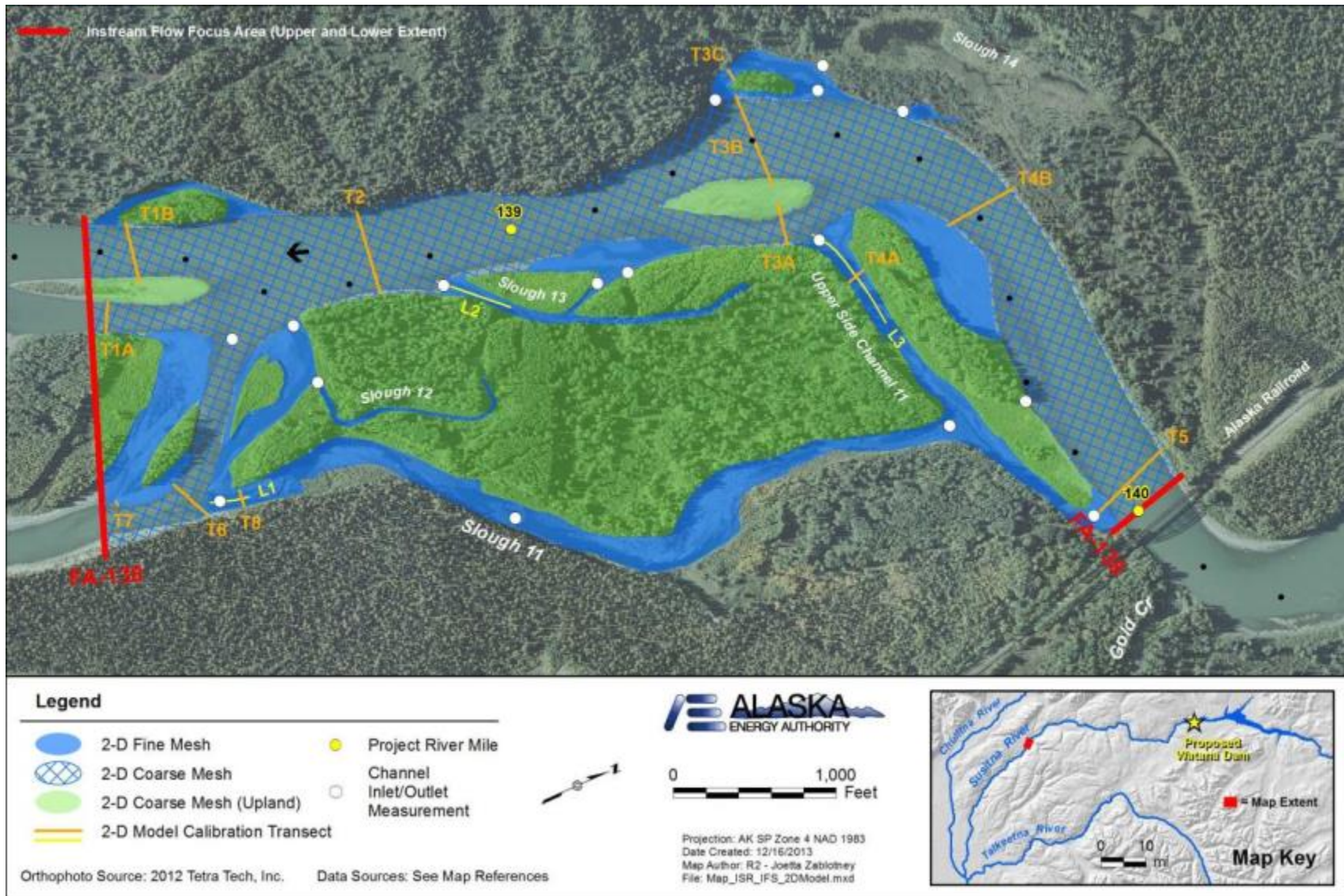
Figure 5.6-5. FA-138 (Gold Creek) showing fine and course mesh overlays, channel inlet and outlet measurement locations, and alignment of 2013 calibration transects.
