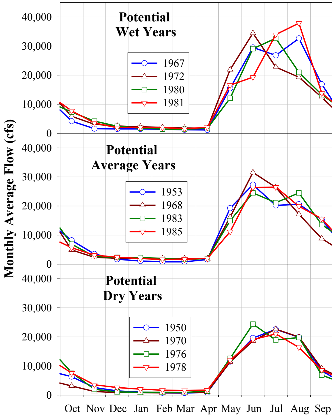
Figure 5.3-8. Monthly average flow for potential wet, average, and dry representative years using a linear scale.
