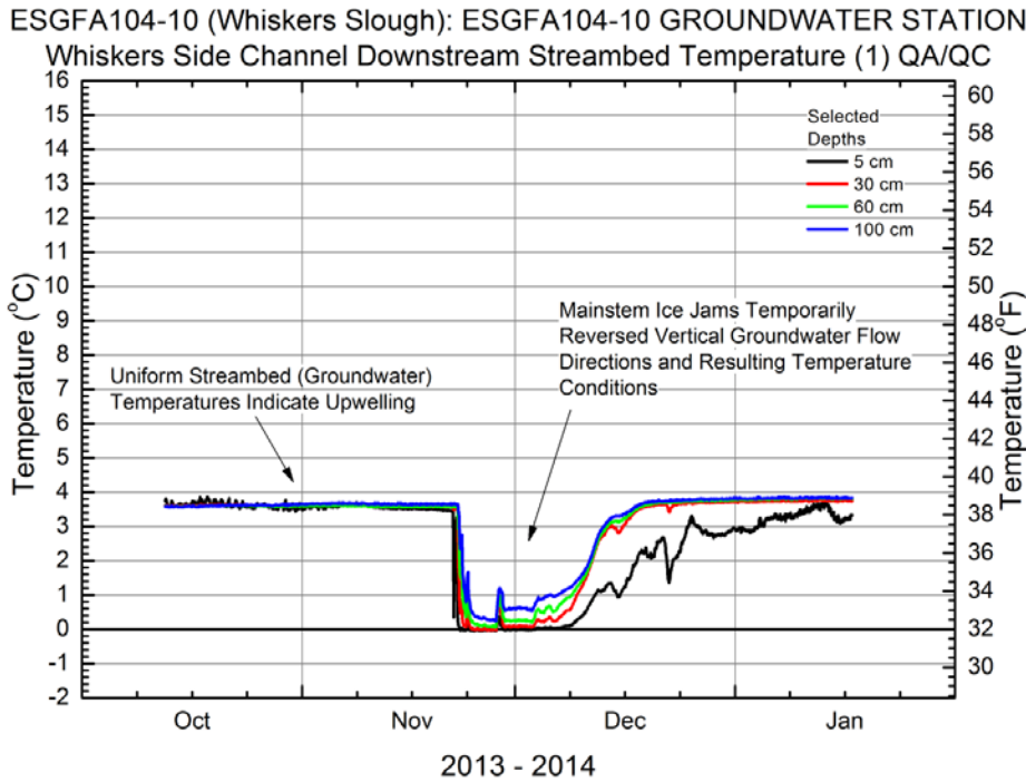
Figure 5.7-9. Example of streambed temperature measurement in the Aquatic Transect in FA-104 (Whiskers Slough) from groundwater station ESGFA104-10. This is the downstream streambed profile. This station is located at the upstream end of Whiskers Side Channel.
