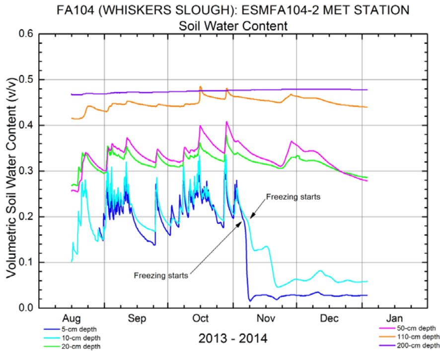
Figure 5.5-6. Example of soil moisture conditions in the Riparian Transect in FA-104 (Whiskers Slough) from meteorological station ESMFA104-2. Data is indicating soil moisture infiltration and freezing events.
