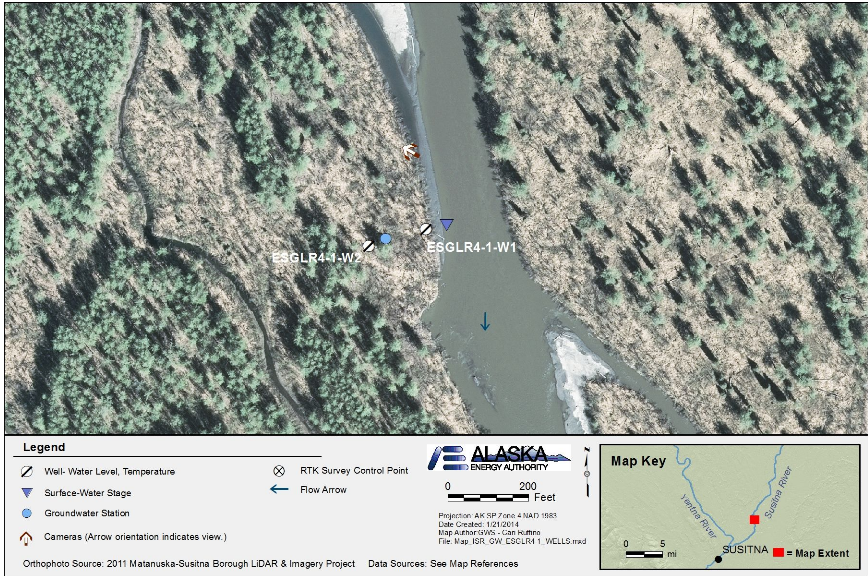
Figure 4.5-23. Well locations and continuously measured parameters at Lower River Transect Groundwater Station ESGLR4-1. Wells are used to obtain groundwater levels and temperature. Surface water stage and temperature, streambed/soil temperature profile, and time-lapse camera locations are shown that record hydrologic and riparian features and processes important to study objectives.
