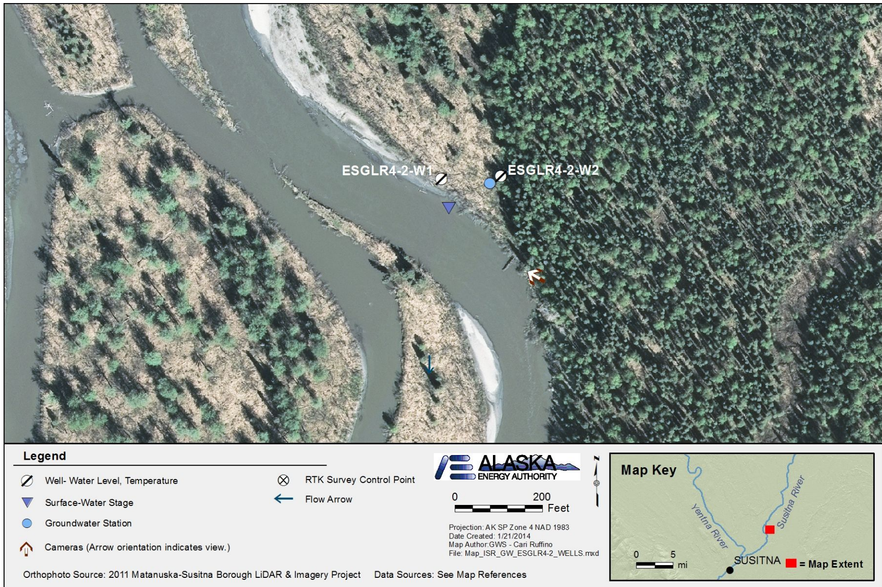
Figure 4.5-24. Well locations and continuously measured parameters at Lower River Transect Groundwater Station ESGLR4-2. Wells are used to obtain groundwater levels and temperature. Surface water stage and temperature, streambed/soil temperature profile, and time-lapse camera locations are shown that record hydrologic and riparian features and processes important to study objectives.
