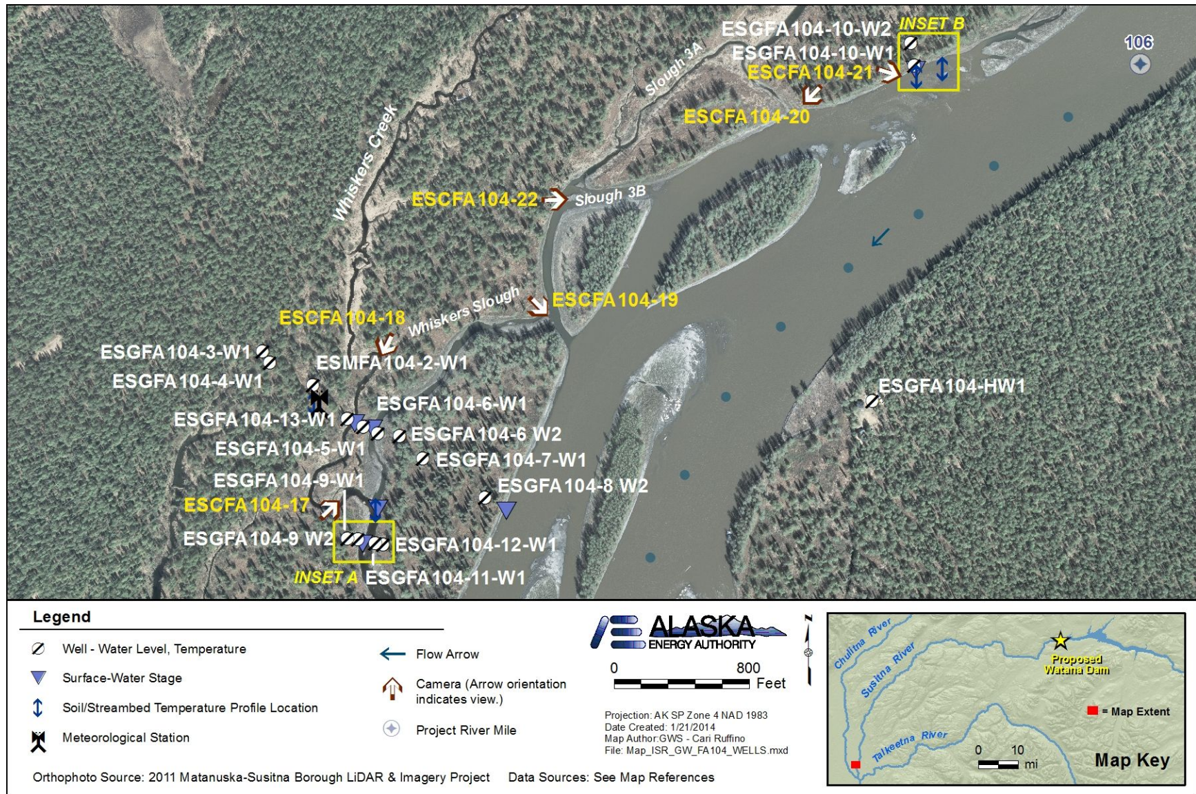
Figure 4.5-18. Well locations and continuously measured parameters at FA-104 (Whiskers Slough) Focus Area. Wells are used to obtain groundwater levels and temperature. Surface water stage and temperature, streambed/soil temperature profile, and time-lapse camera locations are shown that record hydrologic and riparian features. Inset A (left) and B (right) of aquatic transect locations.
