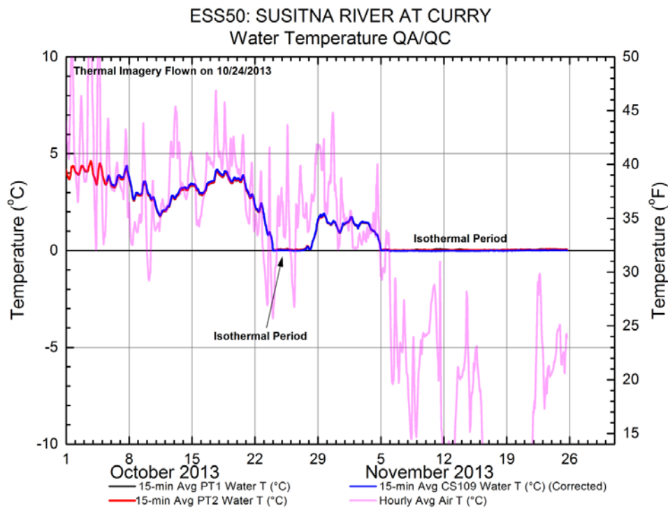
Figure 5.4-2. Example of water quality data processed to support Water Quality Study’s Thermal Infrared (TIR) imagery in the Curry area at hydrology station ESS50.
