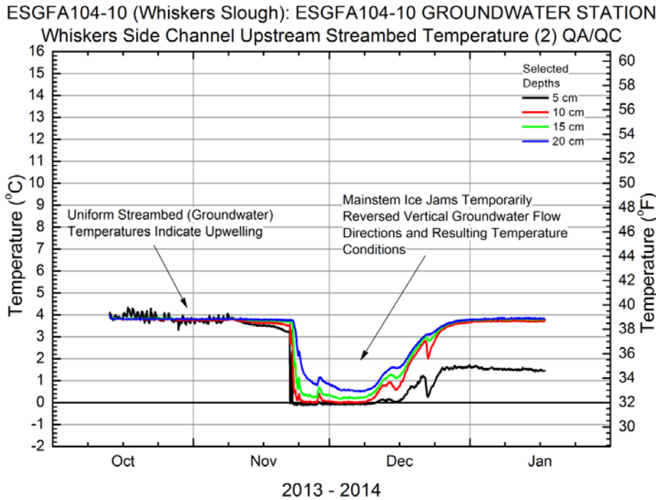
Figure 5.7-10. Example of streambed temperature measurement in the Aquatic Transect in FA-104 (Whiskers Slough) from groundwater station ESGFA104-10. This is the upstream streambed profile sensor at the station (Figure 4.5-19). This station is located at the upstream end of Whiskers Side Channel.
