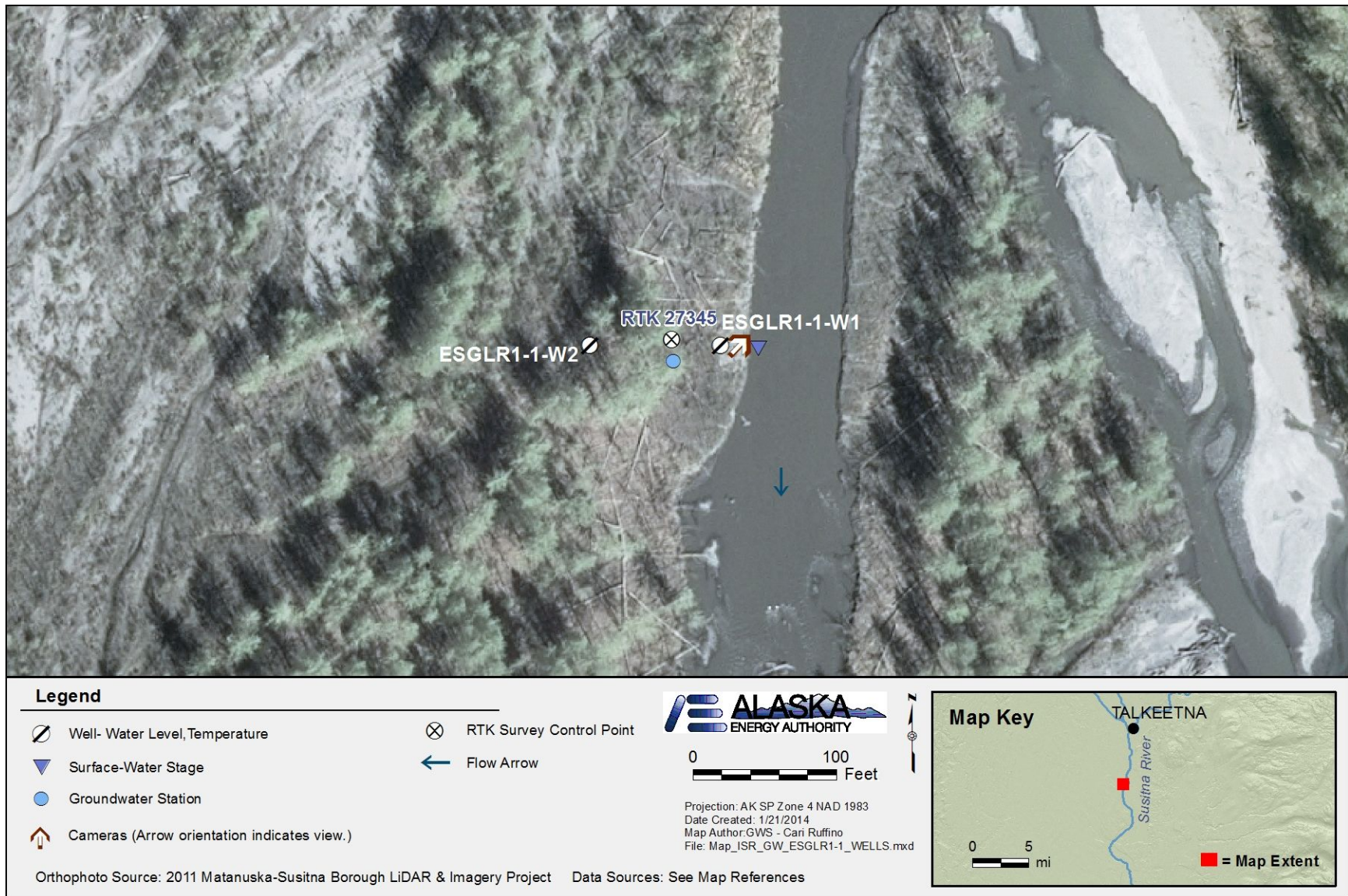
Figure 4.5-20. Well locations and continuously measured parameters at Lower River Transect Groundwater Station ESGLR1-1. Wells are used to obtain groundwater levels and temperature. Surface water stage and temperature, streambed/soil temperature profile, and time-lapse camera locations are shown that record hydrologic and riparian features and processes important to study objectives.
