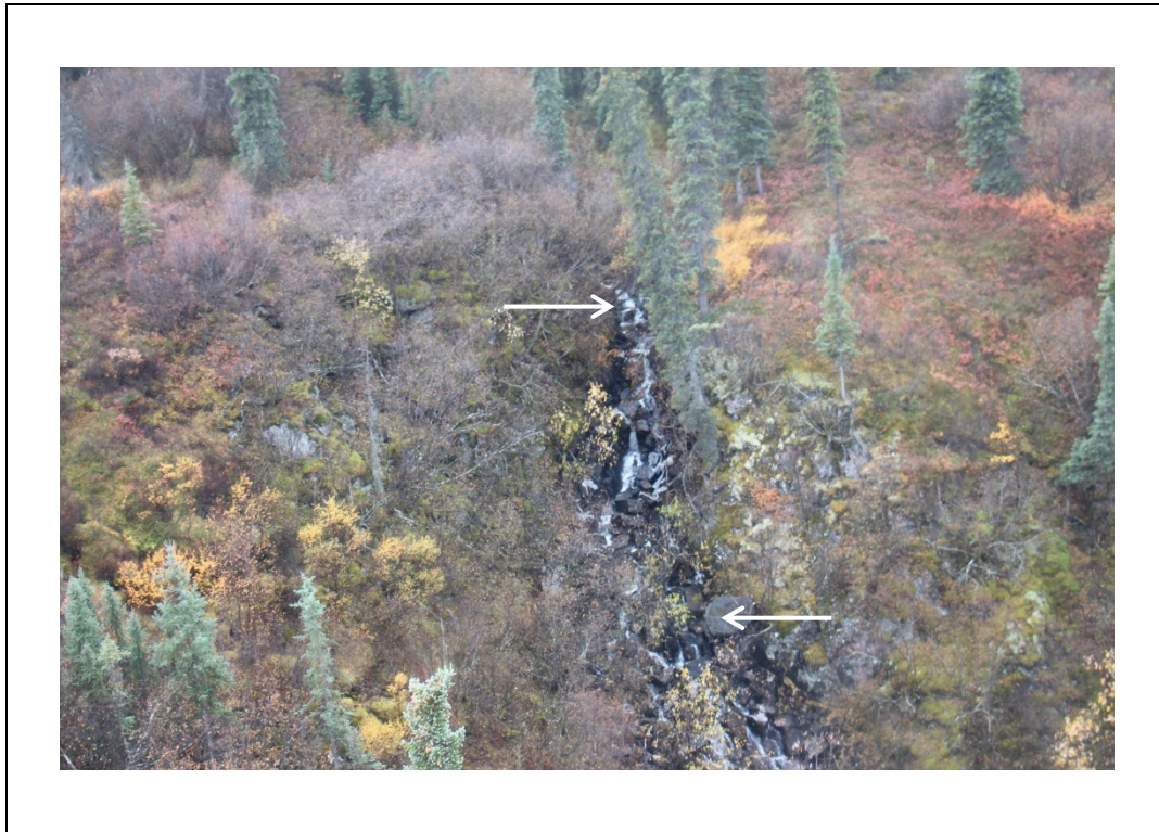
Figure A1. Barrier A in Unnamed Tributary 189.7. Fixed seasonal boulder cascade, 29 ft in height and horizontal length of 36 ft with an average channel gradient of 82 percent.
