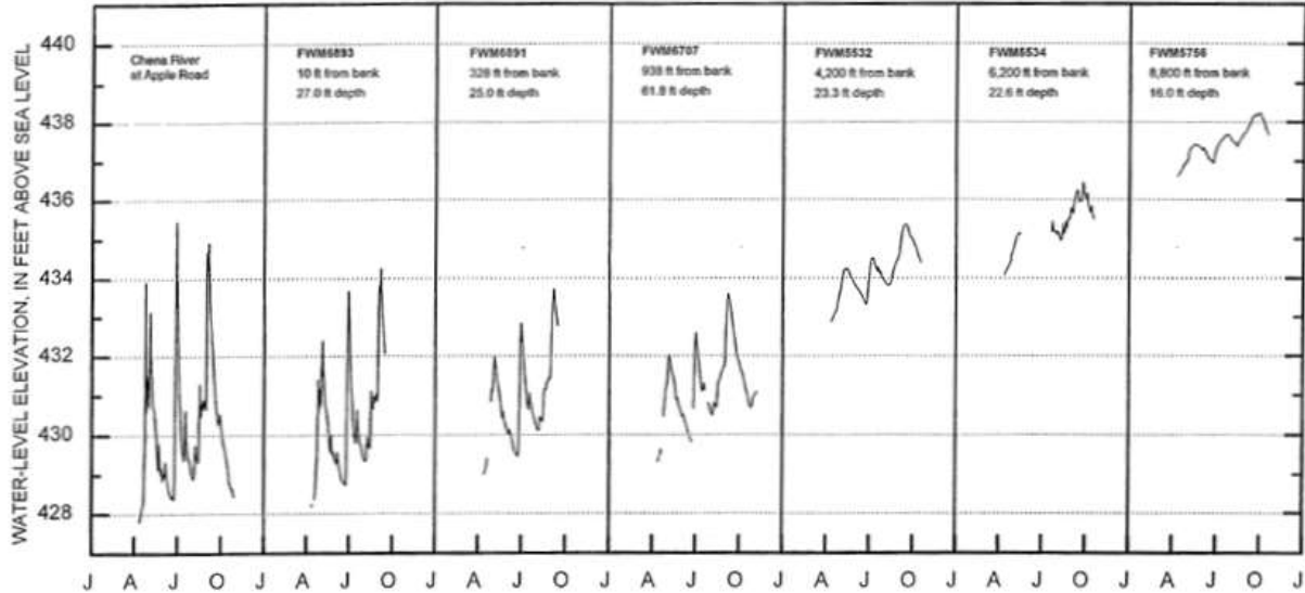
Figure 7.5-6. Groundwater responses to stage changes in the Chena River (Nakanishi and Lilly 1998).
