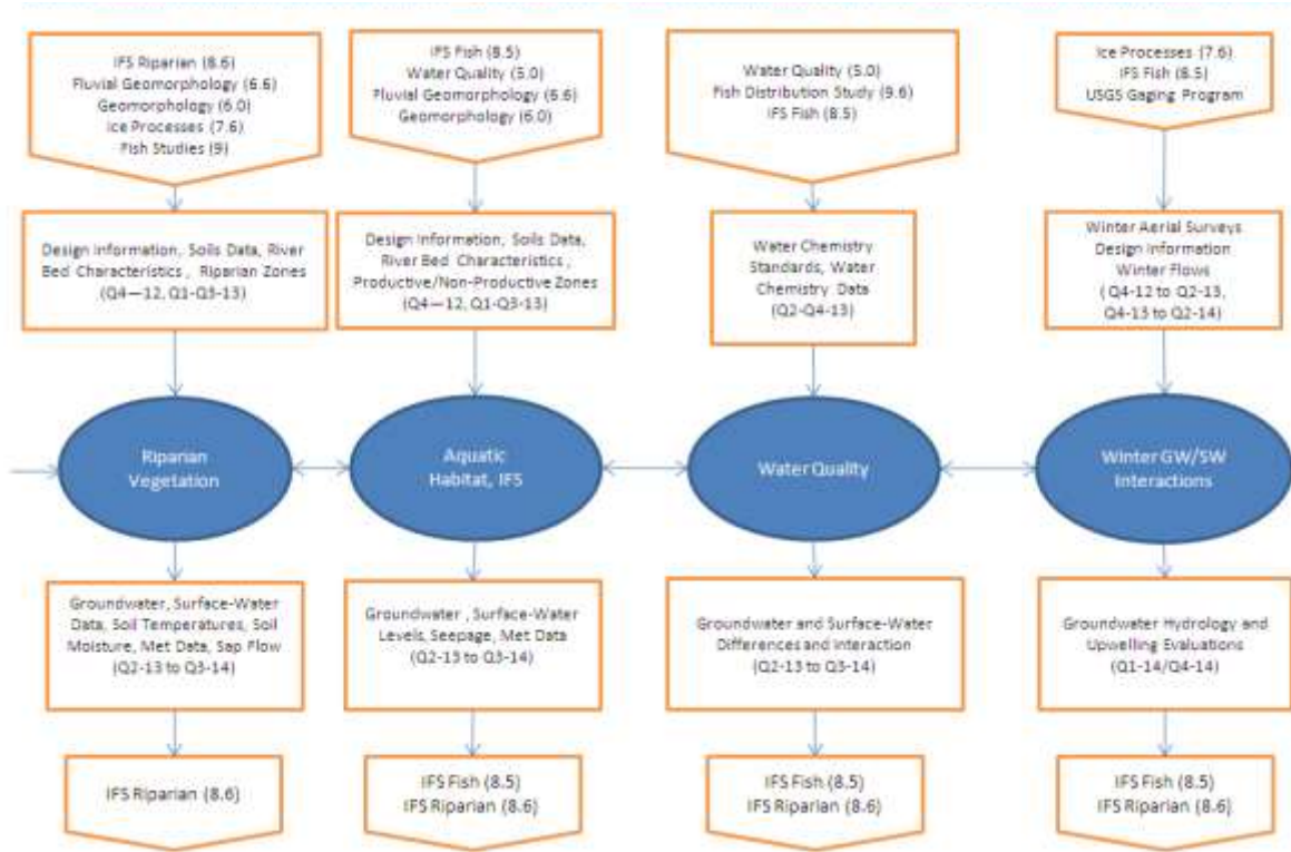
Figure 7.5-3. Study interdependencies for the Groundwater Study (continued).
