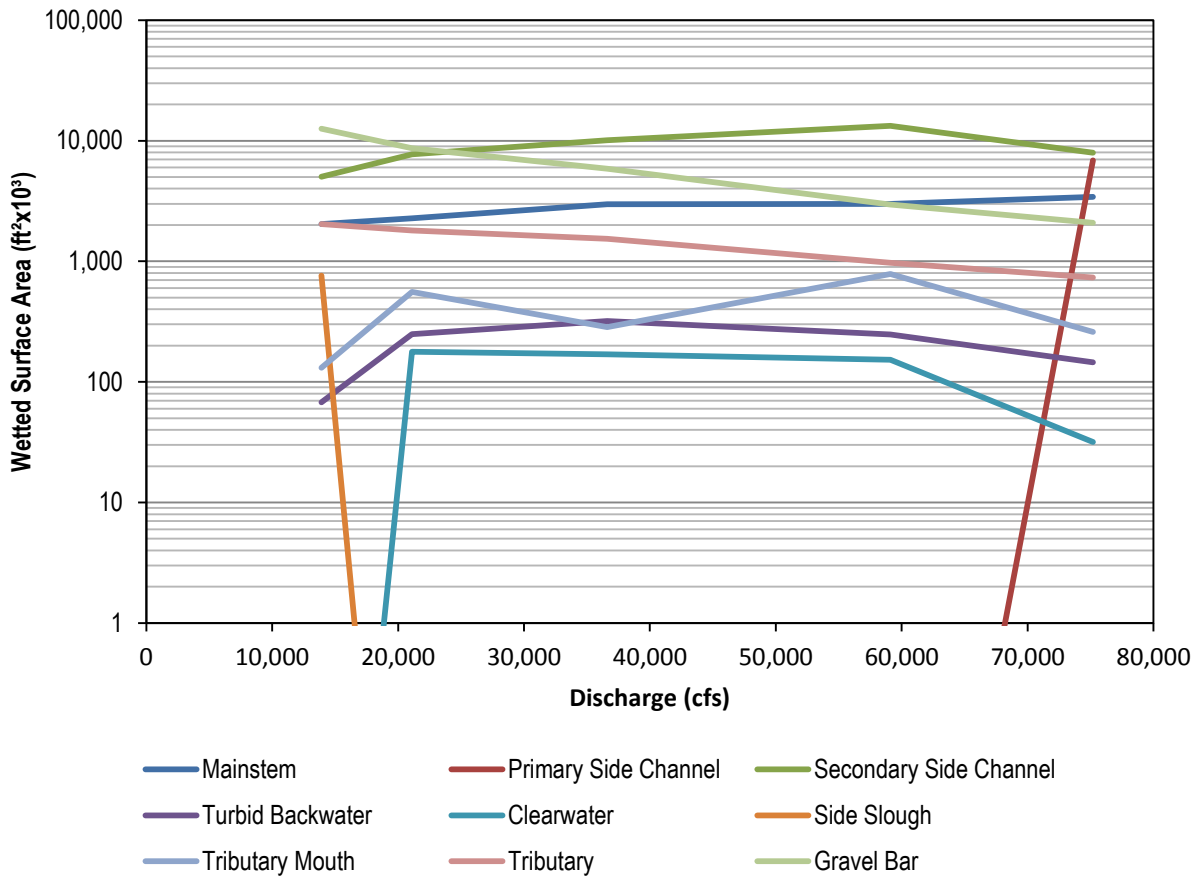
Figure 5.1-1. Wetted surface area ( \text{ft}^2 \times 10^3 ) response to Susitna River discharge at Sunshine by habitat type for Willow Creek. Reproduced from R&M Consultants and Trihey & Associates (1985a).
