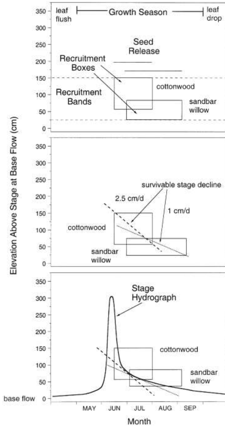
Figure 5. The riparian “Recruitment Box Model” describing seasonal flow pattern, associated river stage (elevation), and flow ramping necessary for successful cottonwood and willow seedling establishment (from Amlin and Rood 2002; Rood et al., 2005). Cottonwood species ( Populus deltoides ), willow species ( Salix exigua ). Stage hydrograph and seed release timing will vary by region, watershed, and plant species.
