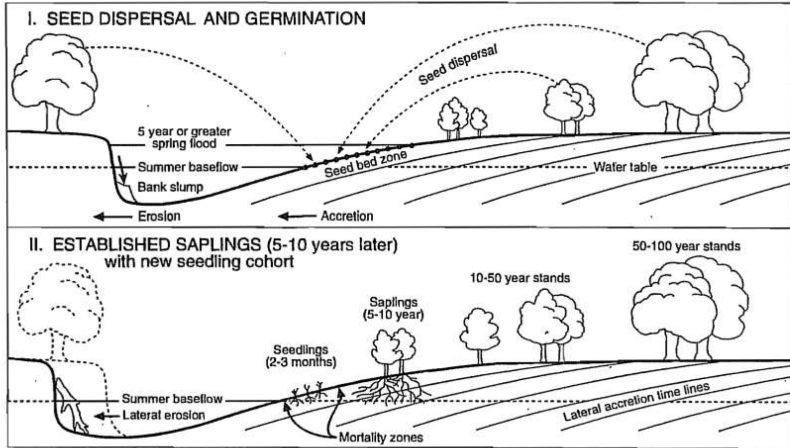
Figure 6. Cottonwood ( Populus ) life history stages: seed dispersal and germination, sapling to tree establishment. Cottonwood typically germinates on newly created bare mineral soils associate with lateral active channel margins and gravel bars. Note proximity of summer baseflow and floodplain water table (Braatne et al. 1996).
