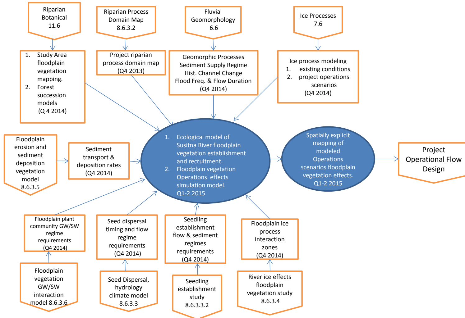
Figure 3. Floodplain Vegetation Study Synthesis, Focus Area to Riparian Process Domain Scaling & Project Operations Effects Modeling (Source: RSP Section 8.6.3.7).
