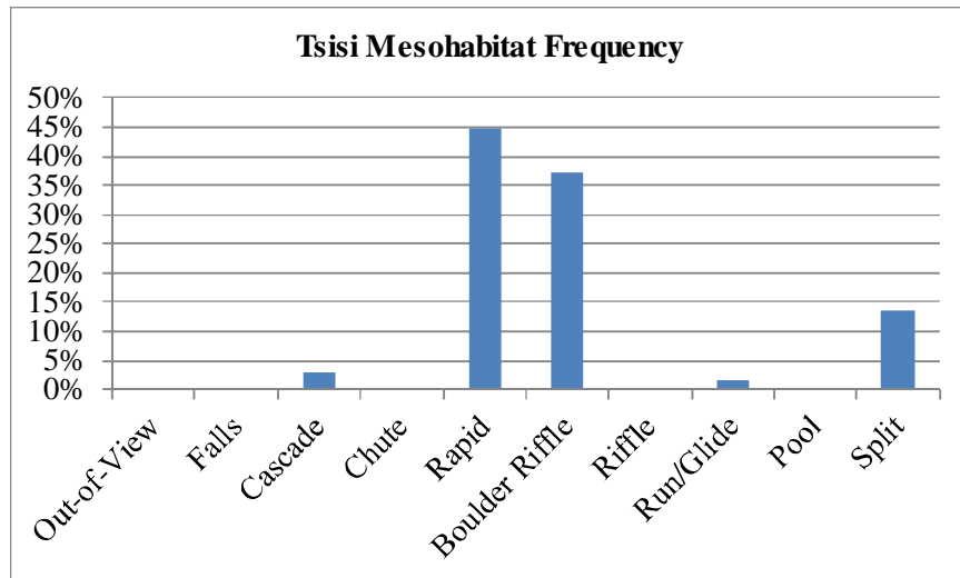
Figure 4.6-1. Tsihi Creek main channel mesohabitat frequency . Aerial video method – 5-second interval
