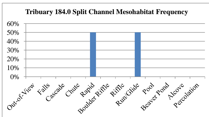
Figure 4.13-2. Tributary 184.0 split channel mesohabitat frequency . Aerial video method – 5-second interval.
