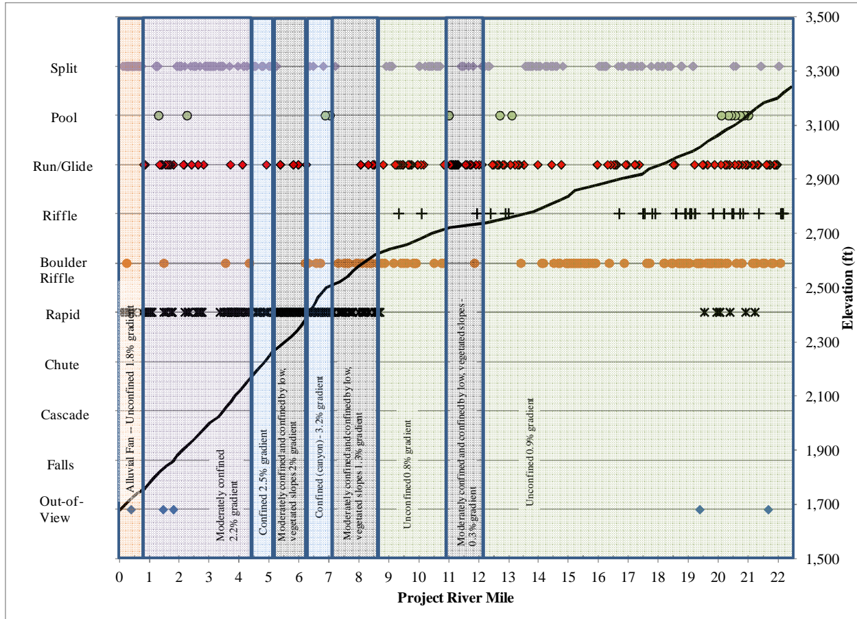
Figure 4.5-3. Kosina Creek distribution of mesohabitat types by rivermile, gradient, and geomorphic reach type.
