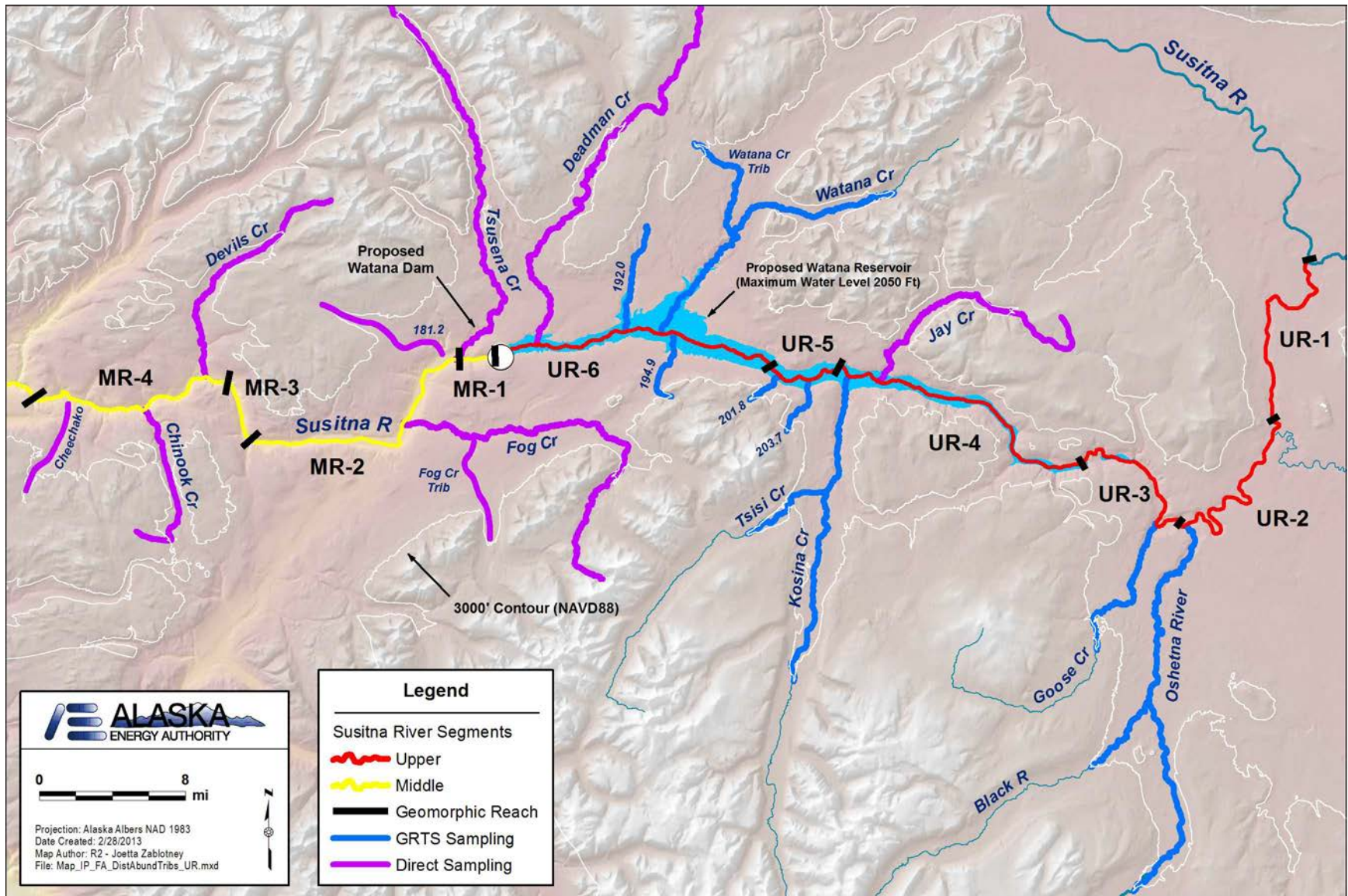
Figure 5.2-1. Locations of 20 tributaries upstream of Devils Canyon selected for sampling.
