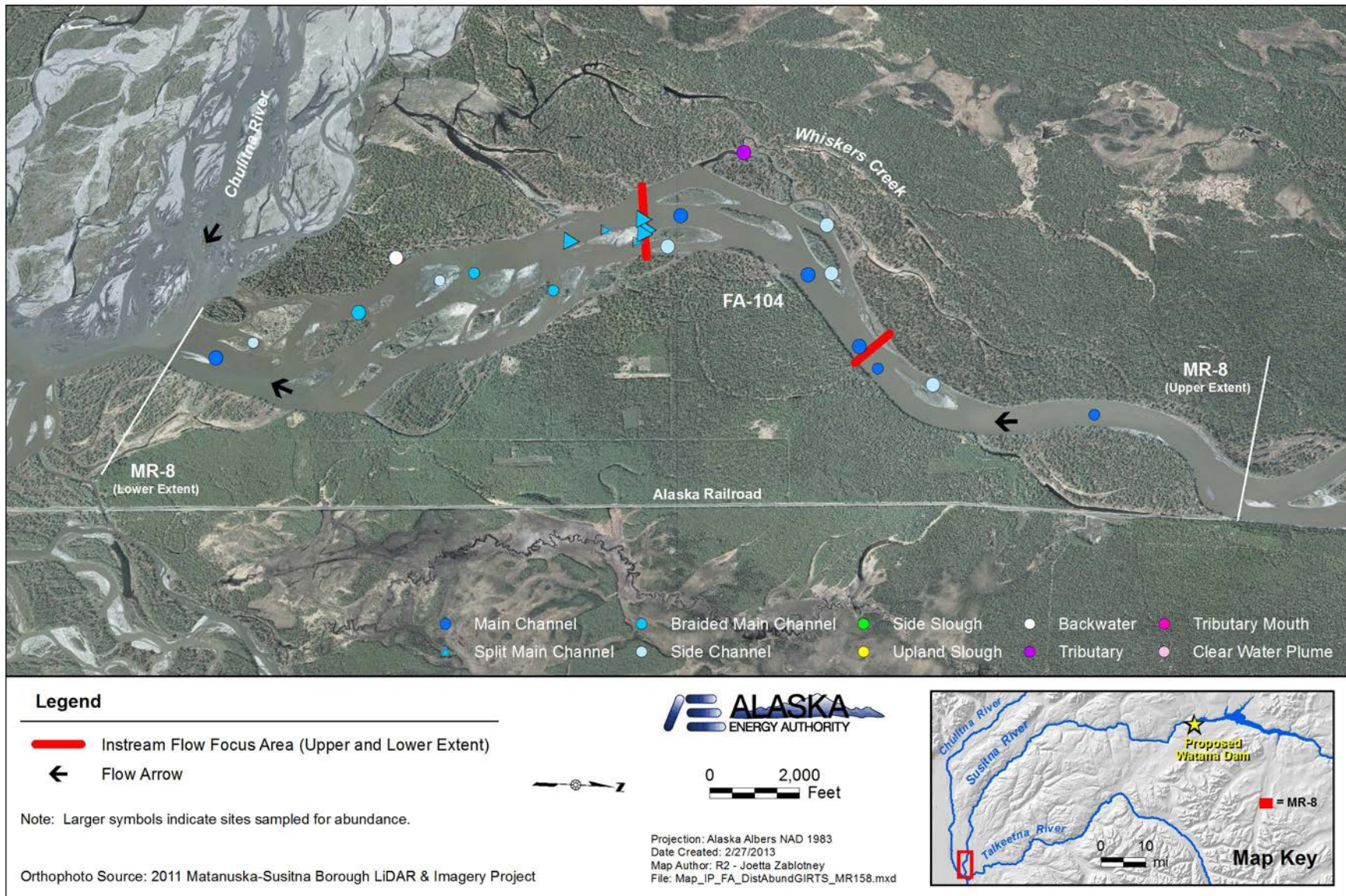
Figure 5.3-6. GRTS site selection by habitat type for Geomorphic Reach MR-8. Note: In addition, three sampling sites in upland slough habitats that are identified in Table 5.3-1 are not identified in this map.
