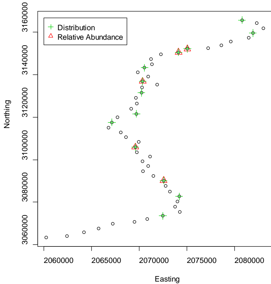
Figure 5.2-2. GRTS sample locations selected for the Oshetna River. Each black circle represents the downstream edge of an 800m sample unit.
