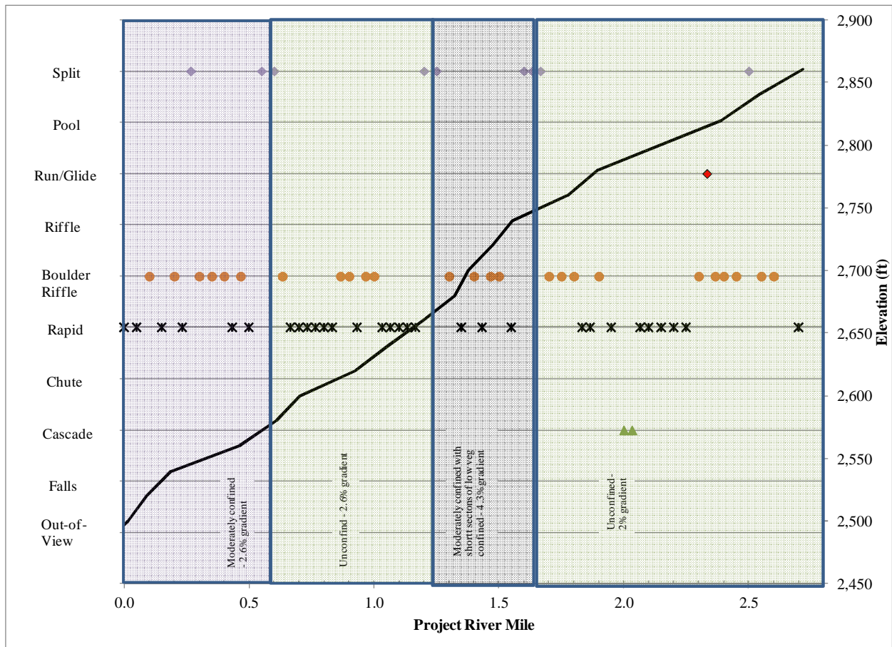
Figure 4.6-3. Tsis Creek distribution of mesohabitat types by rivermile, gradient, and geomorphic reach type.
