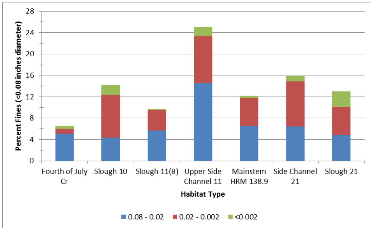
Figure 4.3-2. Percent size composition of fine substrate (<0.08 in. diameter) in McNeil samples collected at chum salmon redds during May 1984 in study sites of middle Susitna River, Alaska. Source Vining et al. (1985).
