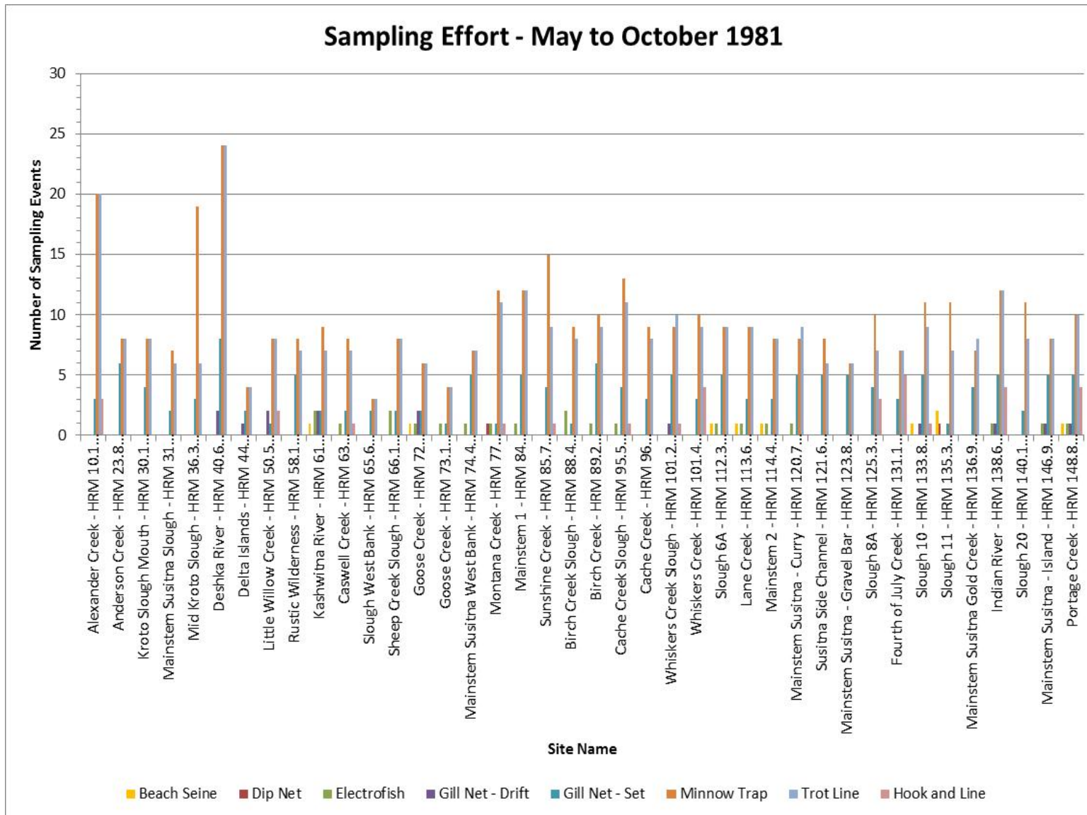
Figure 4.1-3. Sampling effort at 39 habitat location sites (including mainstem, slough, side channel, tributary, and tributary mouth sites) from May to mid-October 1981. Source: Delaney et al. (1981b).
