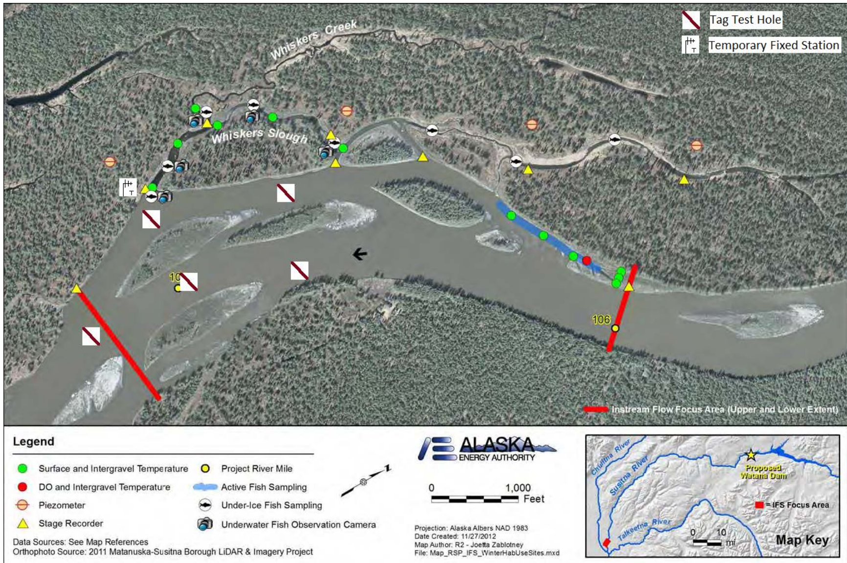
Figure 1. Winter fish sampling locations at Whiskers Creek. Proposed layout for testing radio telemetry equipment through the ice has been added.
