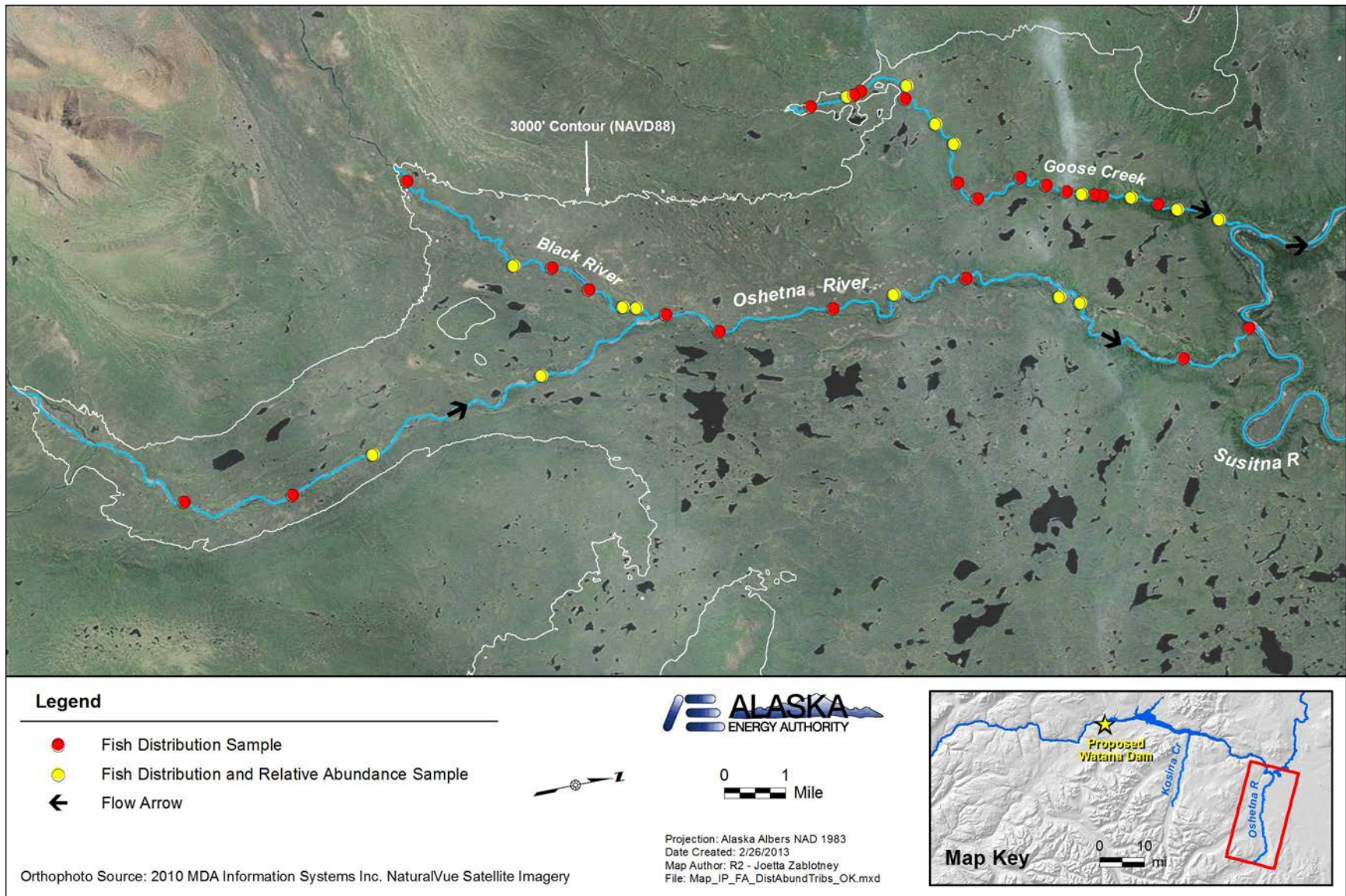
Figure 5.2-5. Map showing sample locations in the Oshetna River, Black River and Goose Creek. Dots represent location of sampled reaches of length 800 meters (Oshetna River), 400 meters (Black River) or 200 meters (Goose Creek).
