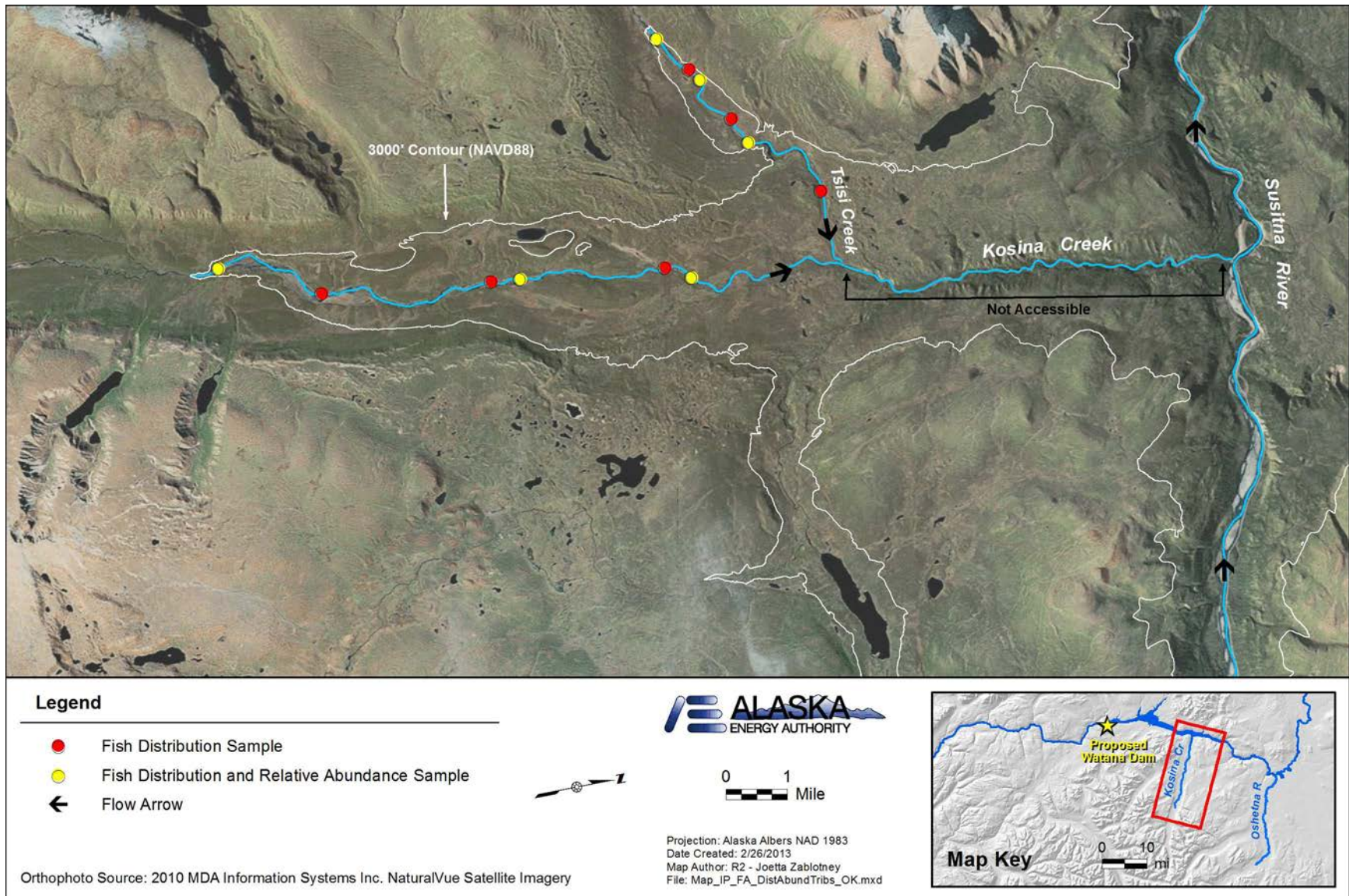
Figure 5.2-6. Map showing sample locations in Kosina and Tsihi creeks. Dots represent locations of 800 meters (Kosina Creek) or 400 meters (Tsihi Creek) sampling units.
