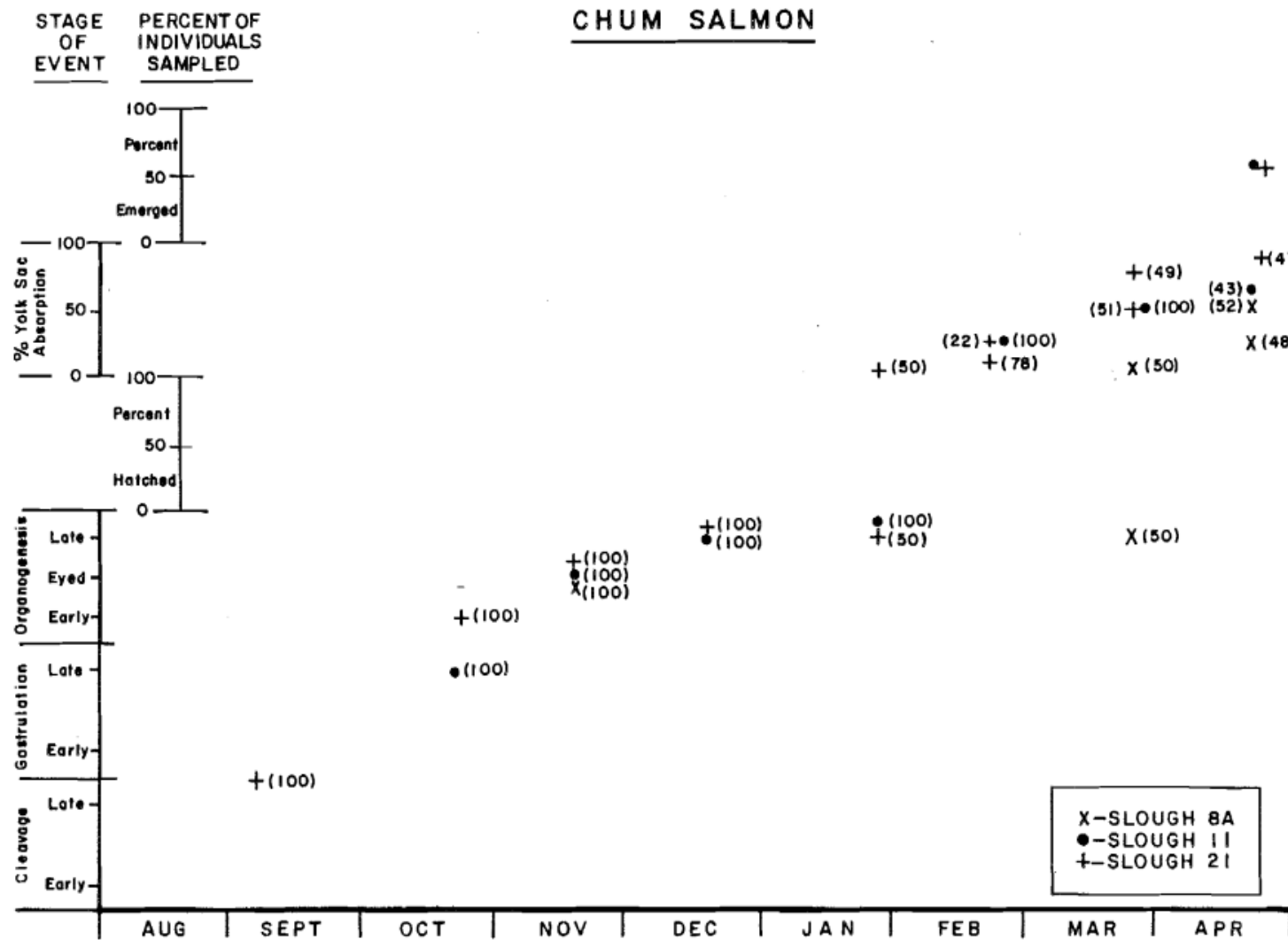
Figure 4.3-4. Embryonic development, hatching, yolk sac absorption, and emergence data for chum salmon at three sloughs, winter, 1982-1983. Numbers in parentheses are the percentages of individuals sampled which were at the indicated stage. Source: Hoffman et al. (1983).
