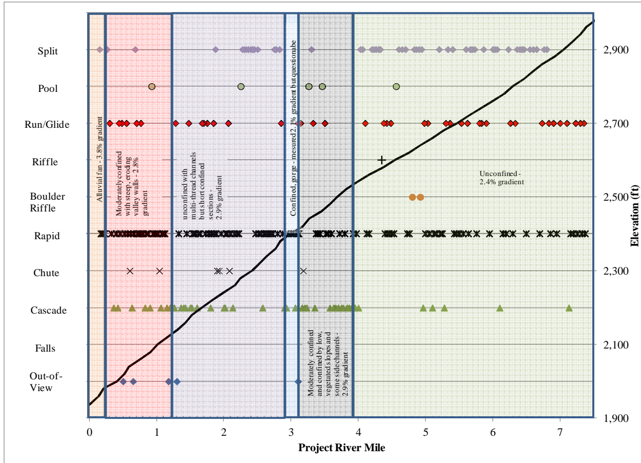
Figure 4.12-3. Fog Creek Tributary L1 distribution of mesohabitat types by rivermile, gradient, and geomorphic reach type.
