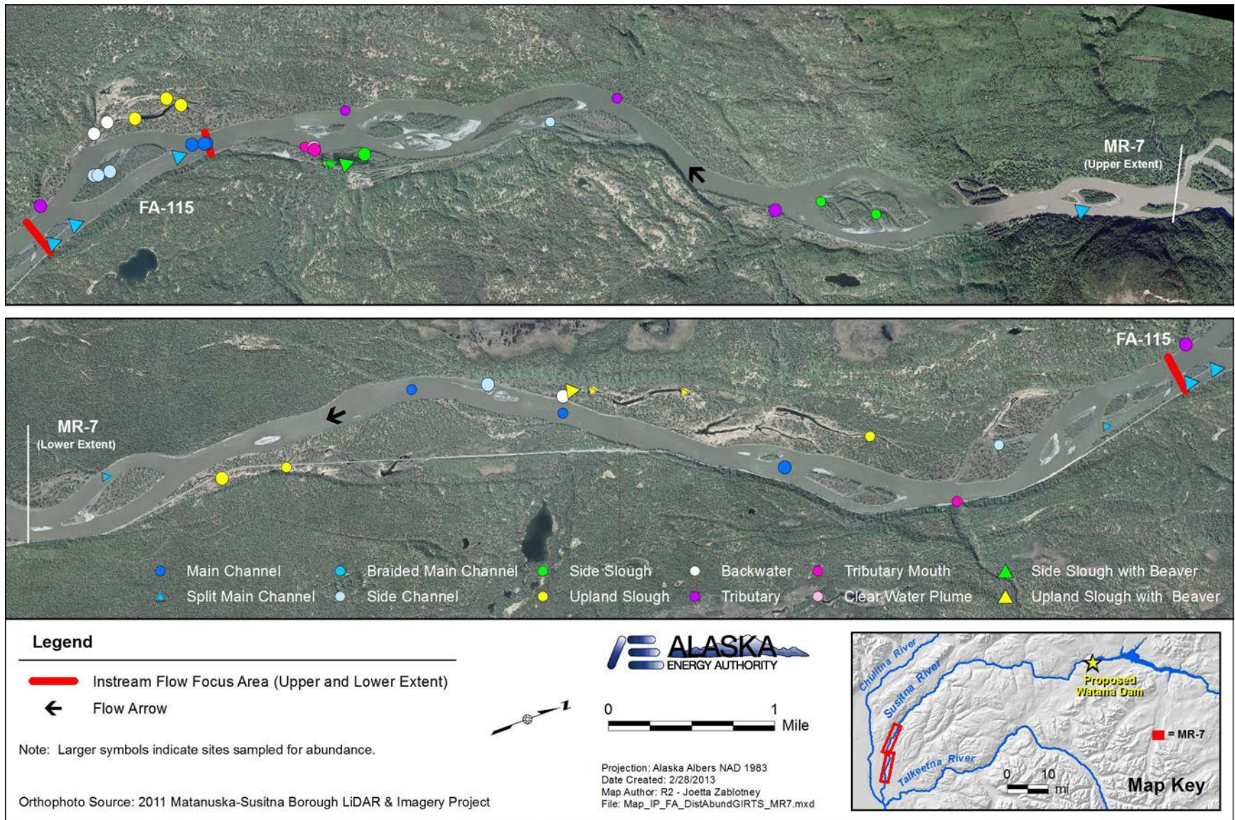
Figure 5.3-5. GRTS site selection by habitat type for Geomorphic Reach MR-7.
