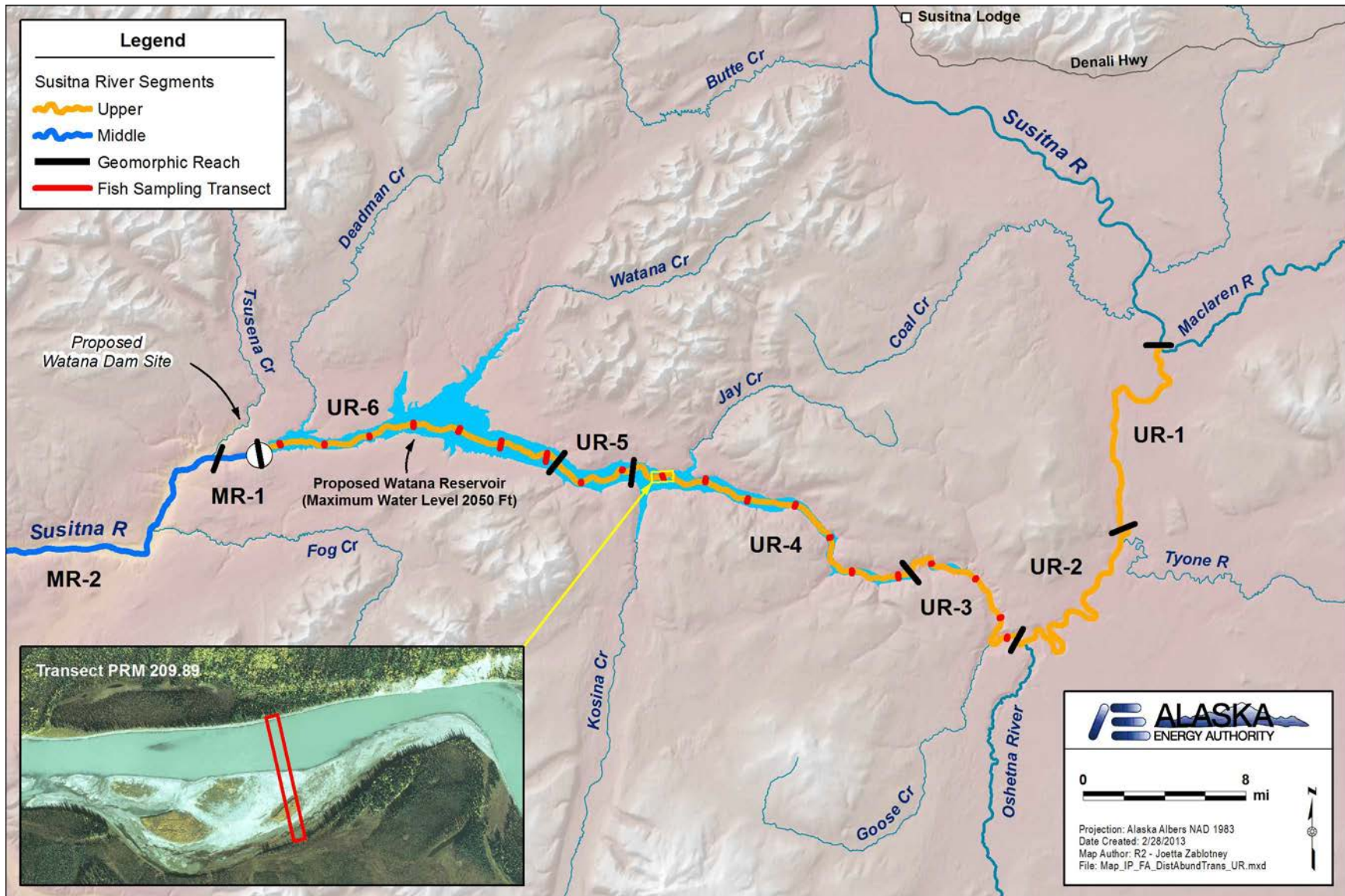
Figure 5.4-2. Fish distribution and abundance sampling transects in the Upper Susitna River.
