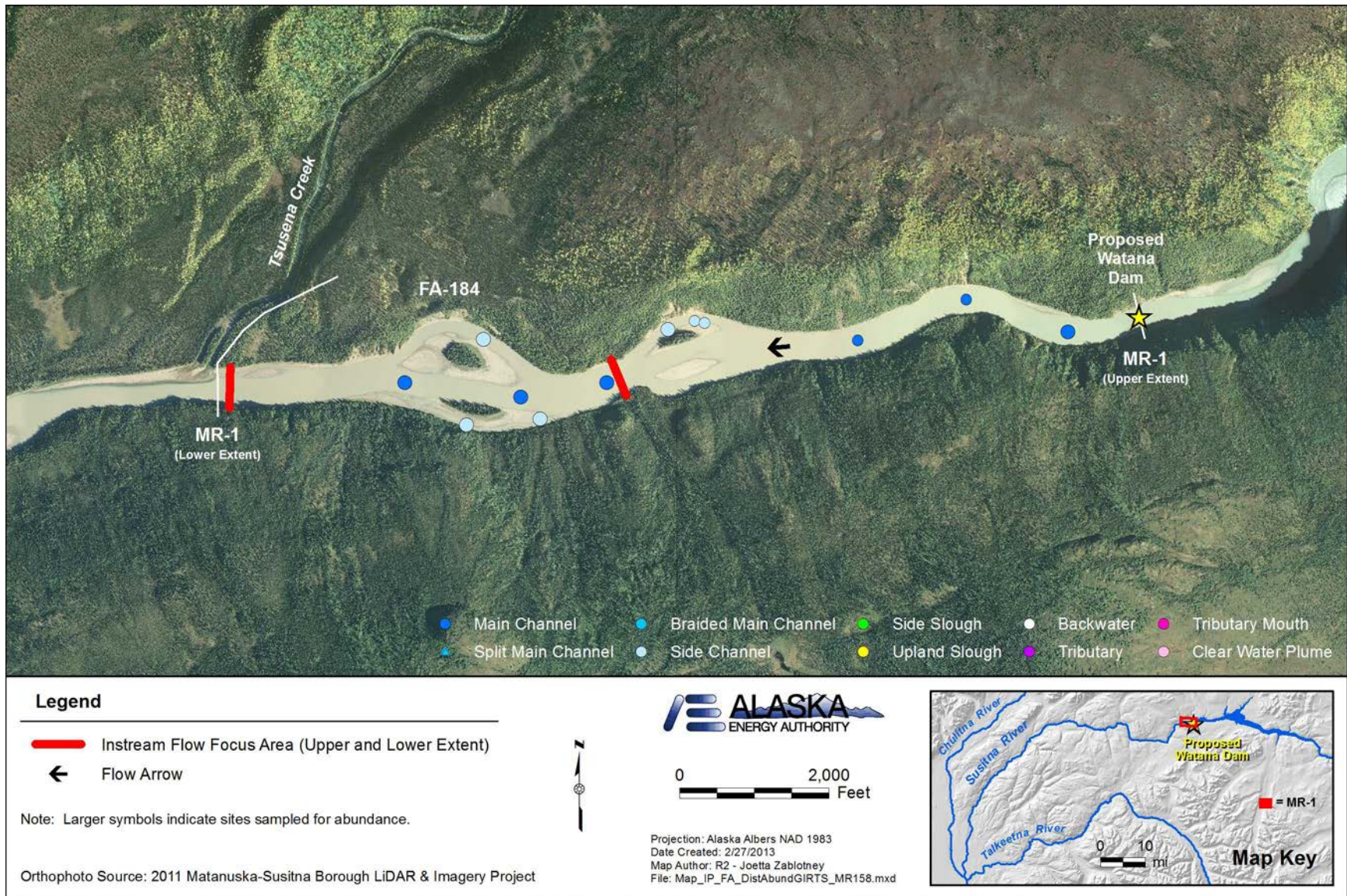
Figure 5.3-1. GRTS site selection by habitat type for Geomorphic Reach MR-1.
