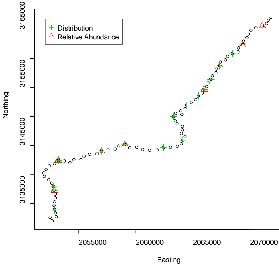
Figure 5.2-3. GRTS sample locations selected for Goose Creek. Each black circle represents the downstream edge of a 200- meter sample unit.
