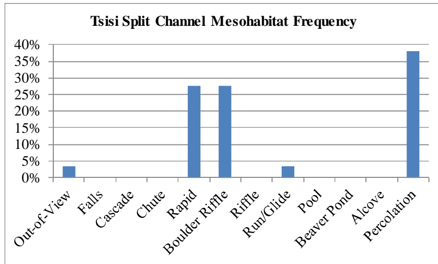
Figure 4.6-2. Tsihi Creek split channel mesohabitat frequency . Aerial video method – 5-second interval.
