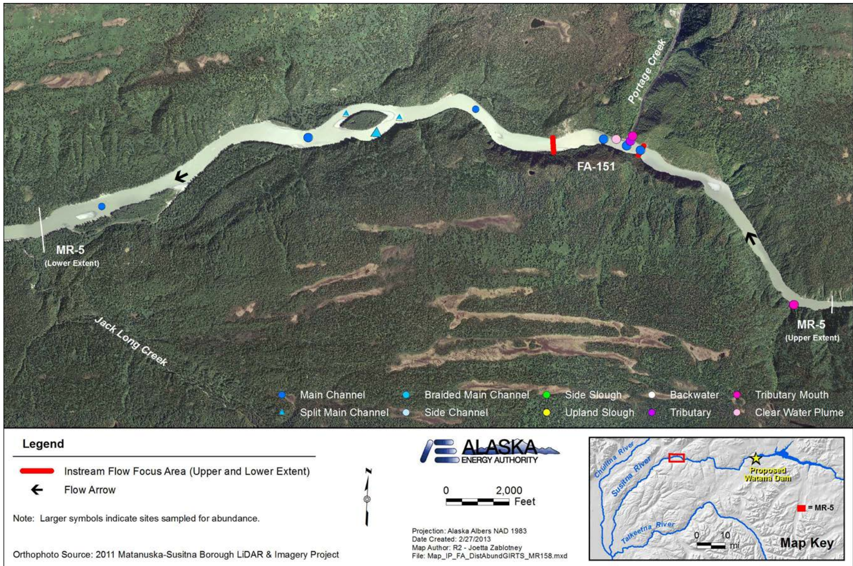
Figure 5.3-3. GRTS site selection by habitat type for Geomorphic Reach MR-5.
