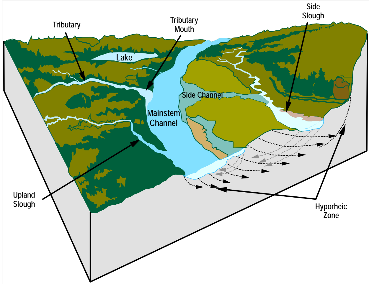
Figure 4.1-2. Habitat types identified in the Middle Susitna River during the 1980s studies (adapted from Schmidt et al. 1983; Trihey 1982).
