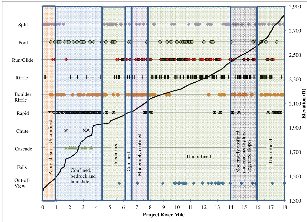
Figure 3. Fog Creek distribution of mesohabitat types by rivermile, gradient, and geomorphic reach.
