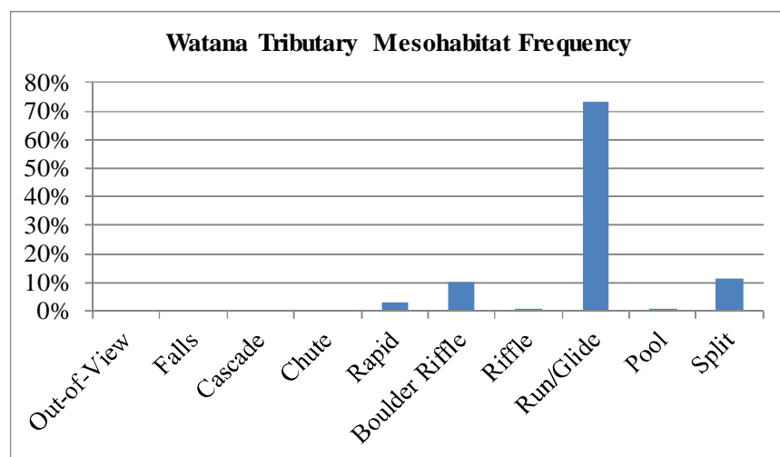
Figure 4.8-1. Watana Creek Tributary R5 main channel mesohabitat frequency . Aerial video method – 5-second interval
