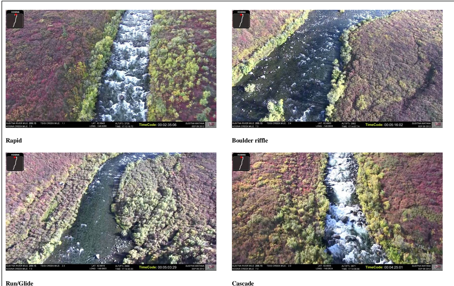
Figure 4.6-4. Tsisi Creek video captures of example mesohabitat types.
