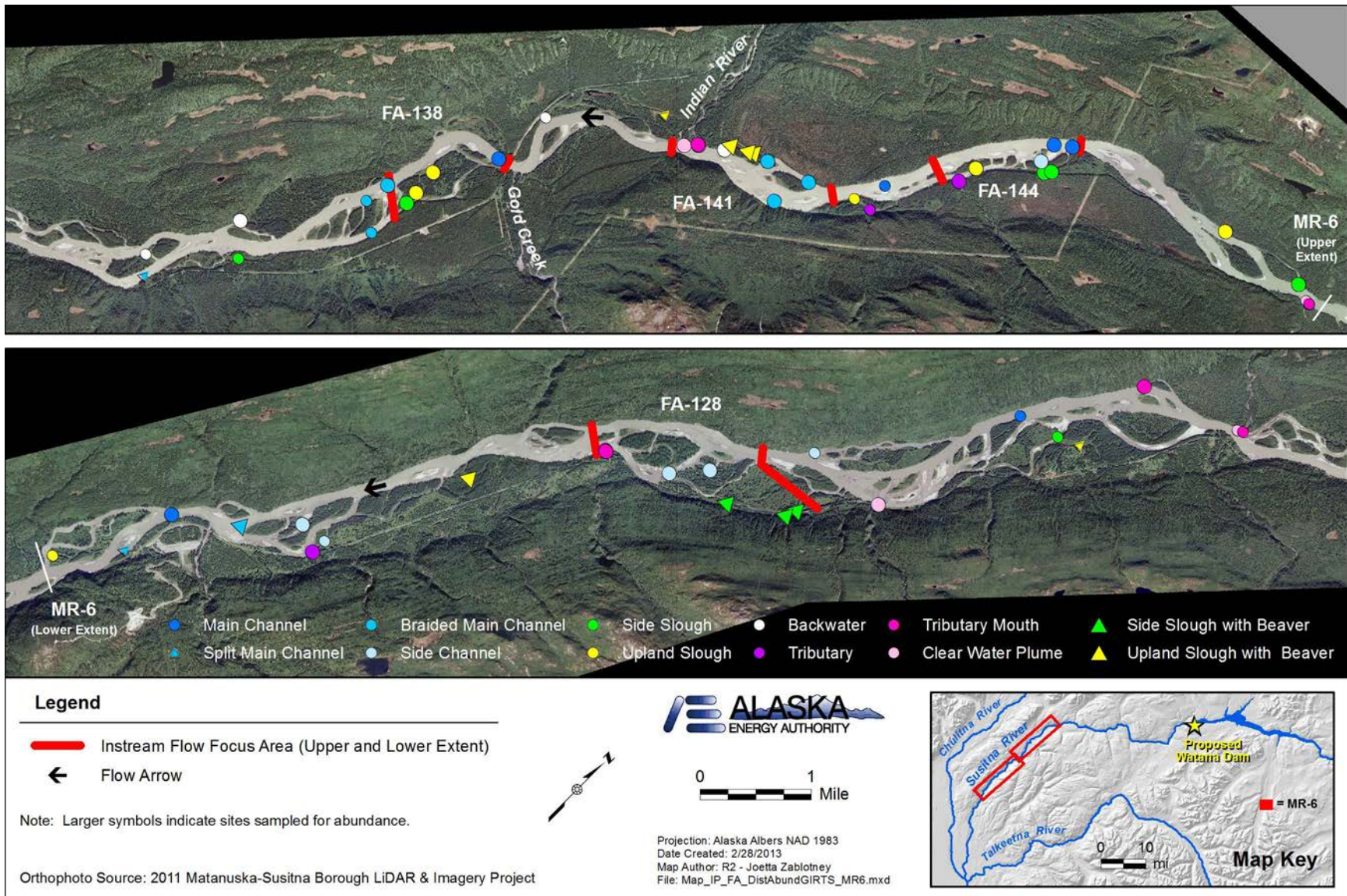
Figure 5.3-4. GRTS site selection by habitat type for Geomorphic Reach MR-6.
