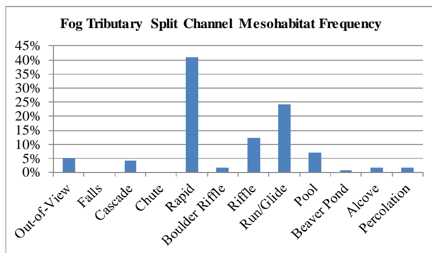
Figure 4.12-2. Fog Creek Tributary L1 split channel mesohabitat frequency . Aerial video method – 5-second interval.
