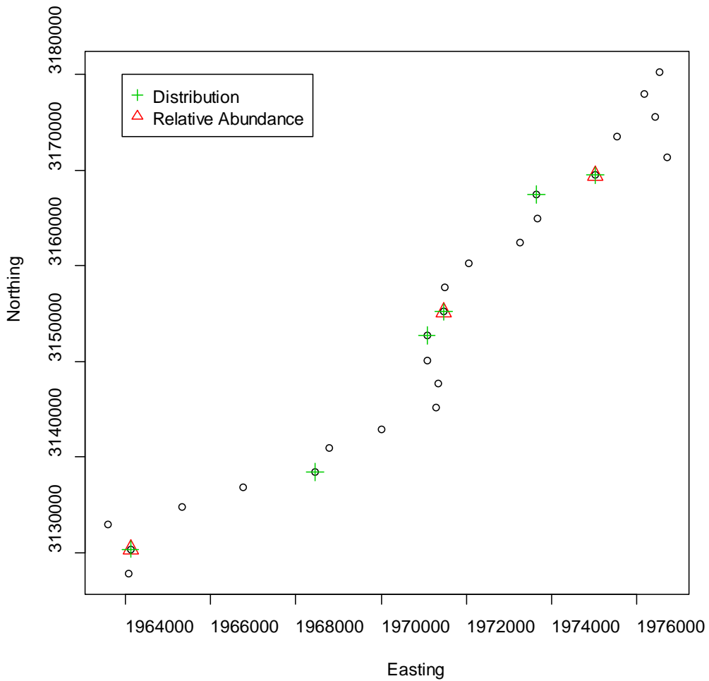
Figure 5.2-4. GRTS sample locations selected for the Kosina River. Each black circle represents the downstream edge of an accessible 800-meter sample unit.
