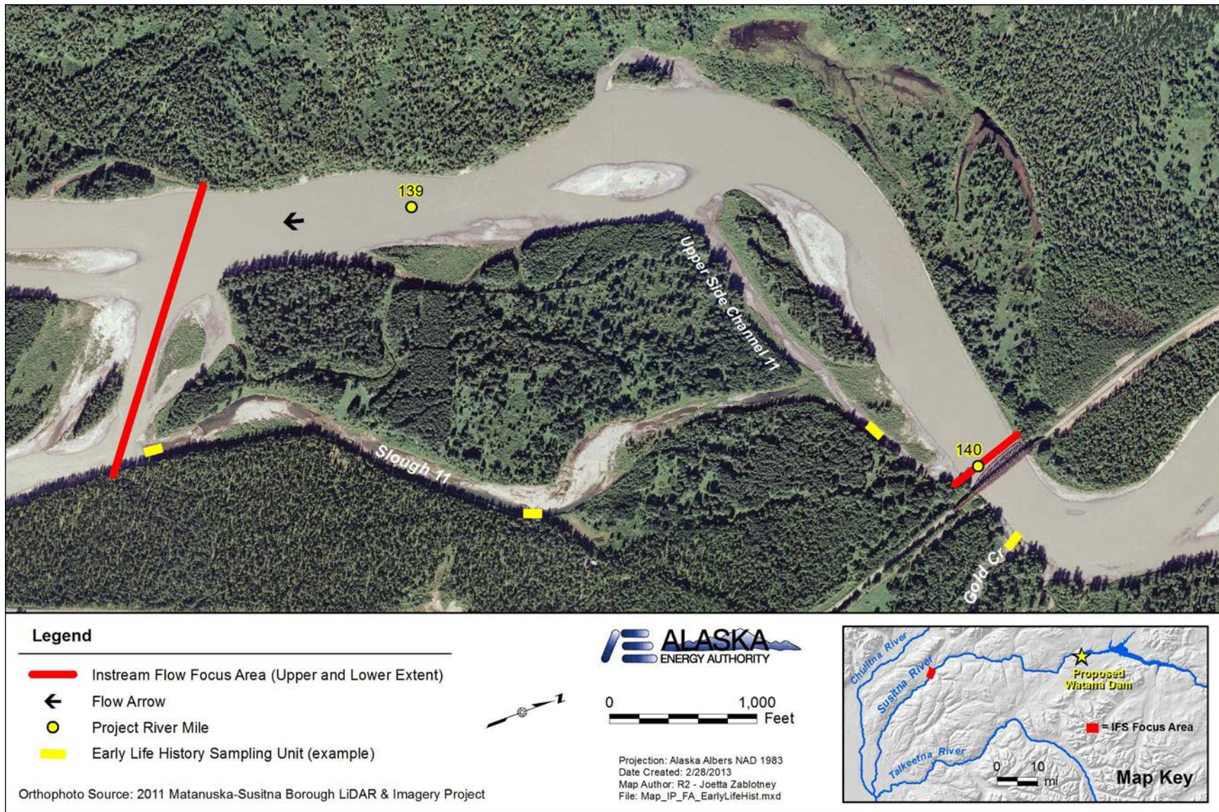
Figure 5.5-1. An example of early-life history sampling units located at (1) mouth of spawning tributary, (2) upper side slough, (3) middle side slough, and (4) side slough mouth. Note: sampling units are 40-meters long and not to scale on figure.
