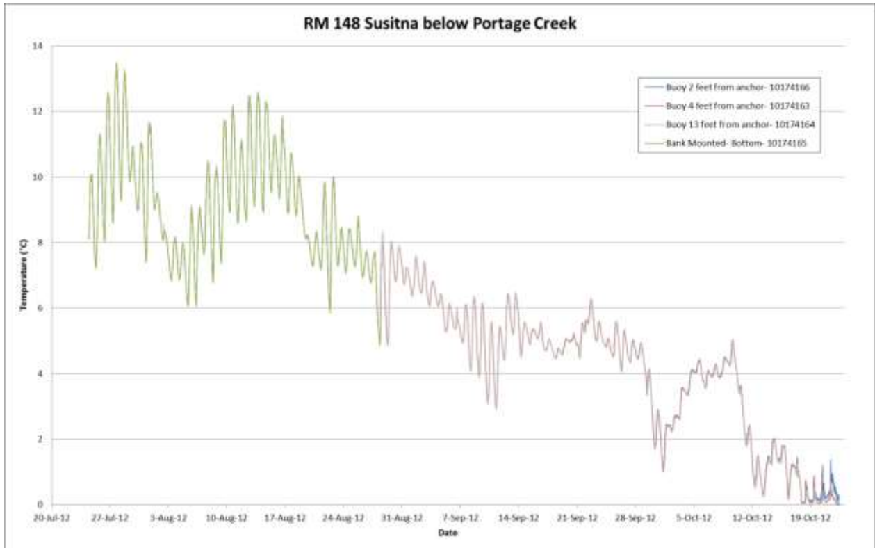
Figure 6.17. Temperature Data RM 148
