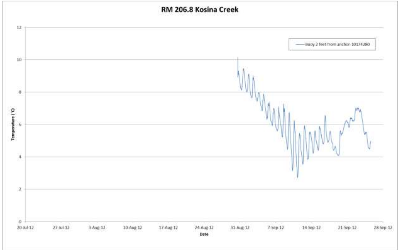
Figure 6.21. Temperature Data RM 206.8
