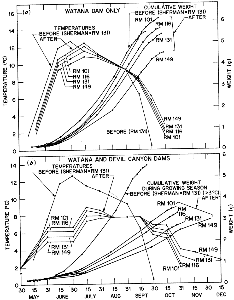
Figure I.2-3. Temperature and cumulative growth for representative juvenile salmon in the Susitna River between Devil Canyon and Talkeetna, before and after the project.
